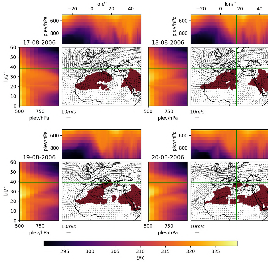
Figure 3. Intrusion event observed during the days 18-19 August 2006. The days before (17 August 2006) and after (20 August 2006) the event are also displayed to frame the intrusion in the synoptic configuration that was occurring at the time. The air mass identified as Saharan is shaded in dark red while the contours show the geopotential height at 500 hPa and the quivers show the direction and magnitude of the wind at 850 hPa. The sub-panels to the left and top of the maps correspond to the vertical sections between pressure levels (plev) 975-500 hPa of potential temperature along the vertical and horizontal green lines.
