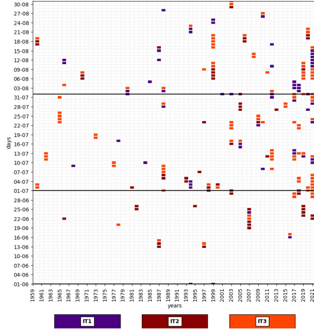
Figure 5. Historical catalogue of intrusion days in the period 1959-2022 (x-axis) and from the 1st June to 30th August (JJA, y-axis). The days identified as intrusions are coloured with their assigned IT. Black lines indicate the change of months.
