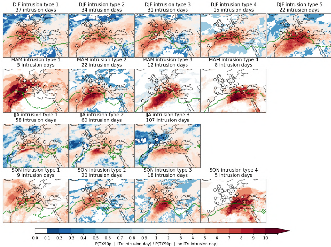
Figure 7. Risk ratio of having an extreme temperature day (TX90p) in days with and without Saharan warm air intrusions for each season (rows) and IT (columns). It is computed as the fraction of the impact divided by the probability of having an extreme temperature day when no ITn day is recorded. Colored dots are results from ECA&D station data (Table S1). The area of influence is displayed with a green (dotted) contour, and represents the limit where Saharan air masses have been recorded in the historical period for a specific IT.
