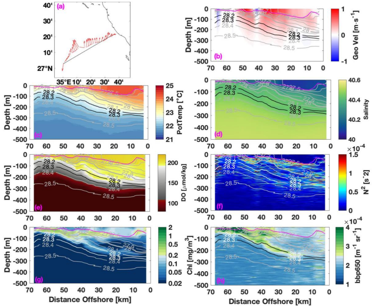
Fig. 5: Glider section of a) Depth Averaged Current (DAC), b) Geostrophic velocity, c) Potential temperature, d) Salinity, e) DO, f) Brunt-Väisälä frequency, g) CHL, and h) Backscattering coefficient at 650 nm, for February 5–9, 2019. Density isopycnals are shown in subfigures b, c, d, e, f, g, and h with solid grey lines, while the isopycnals of 28.2 and 28.3 are distinguished with black lines (or while for f, g, h). The solid magenta line represents the MLD. Geostrophic velocity, calculated relative to 500 m, is positive to the north-northwest and negative to the south-southeast parallel with the coastline.
