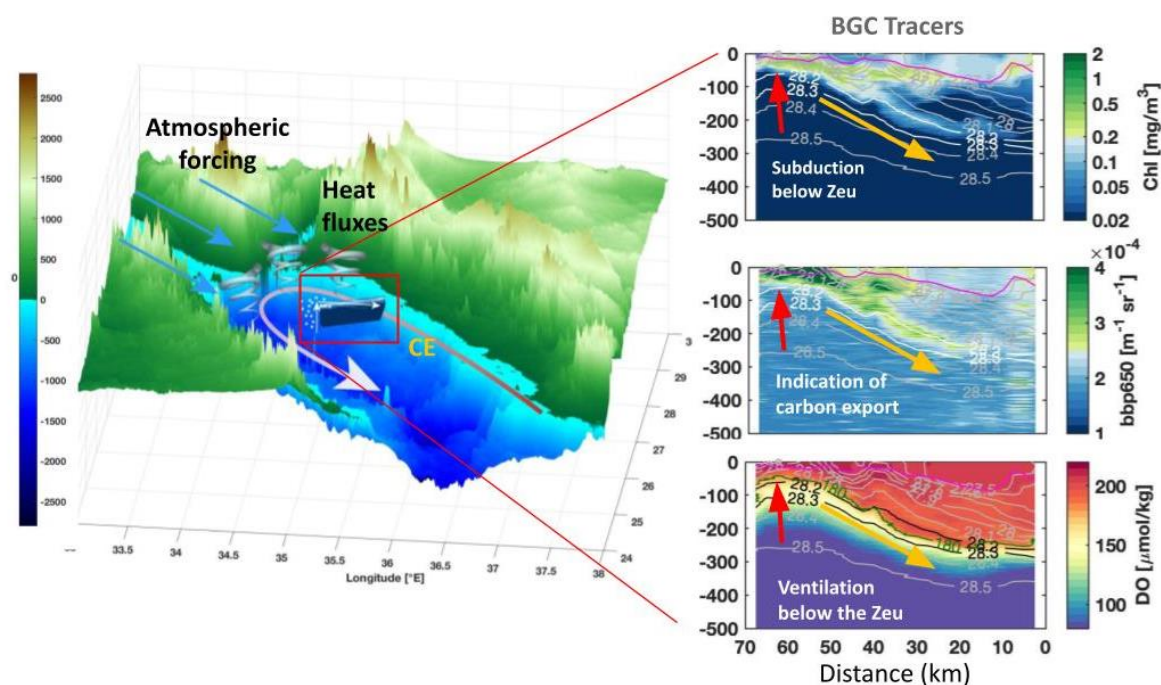
599 Fig. 12: Conceptual diagram of RSOW subduction and its biogeochemical impact on the NRS. 600 Topographic and bathymetric representation of the study area where physical and atmospheric processes 601 superimposed on the map indicate the general cyclonic circulation (grey arrow), the influence of 602 atmospheric forcing (blue arrows), and heat fluxes (grey spirals; left panel). Panels on the right display
