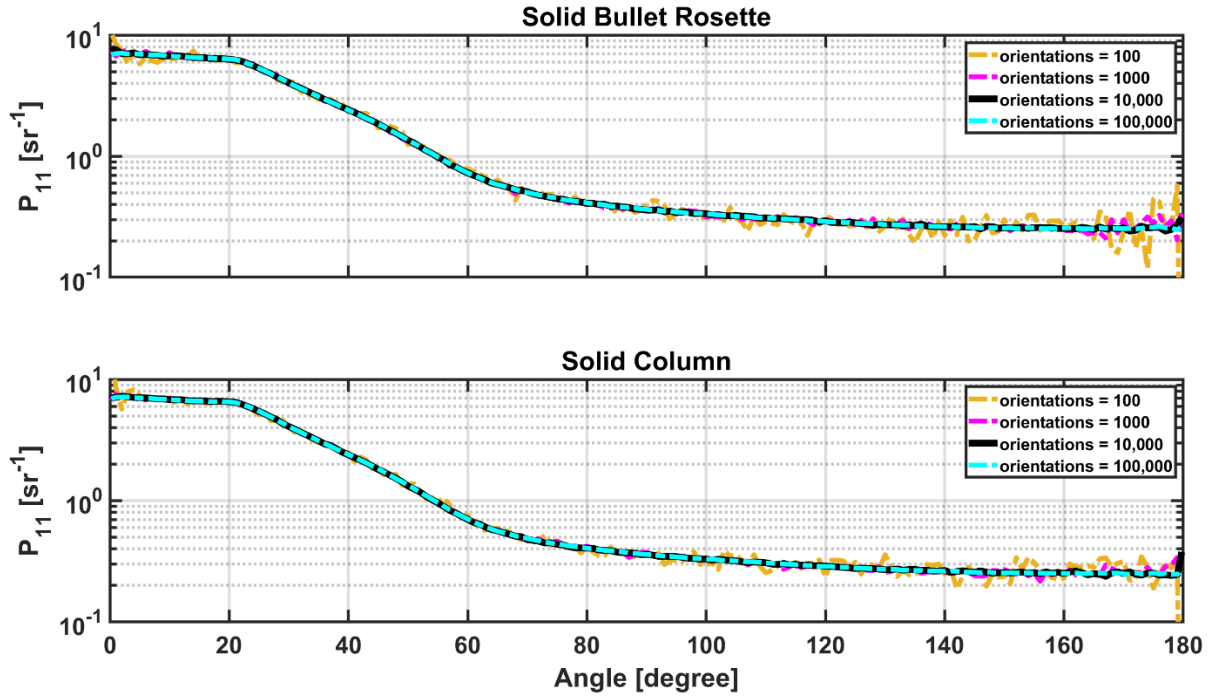
Figure 3: The theoretical phase functions for the modeled solid rosette and solid column, where D = 125 \mu\text{m} and d = 0.6 with a range of orientations from 100 to 100,000. Calculations were performed using the Uniform Tilted Angle (UTA) method.
