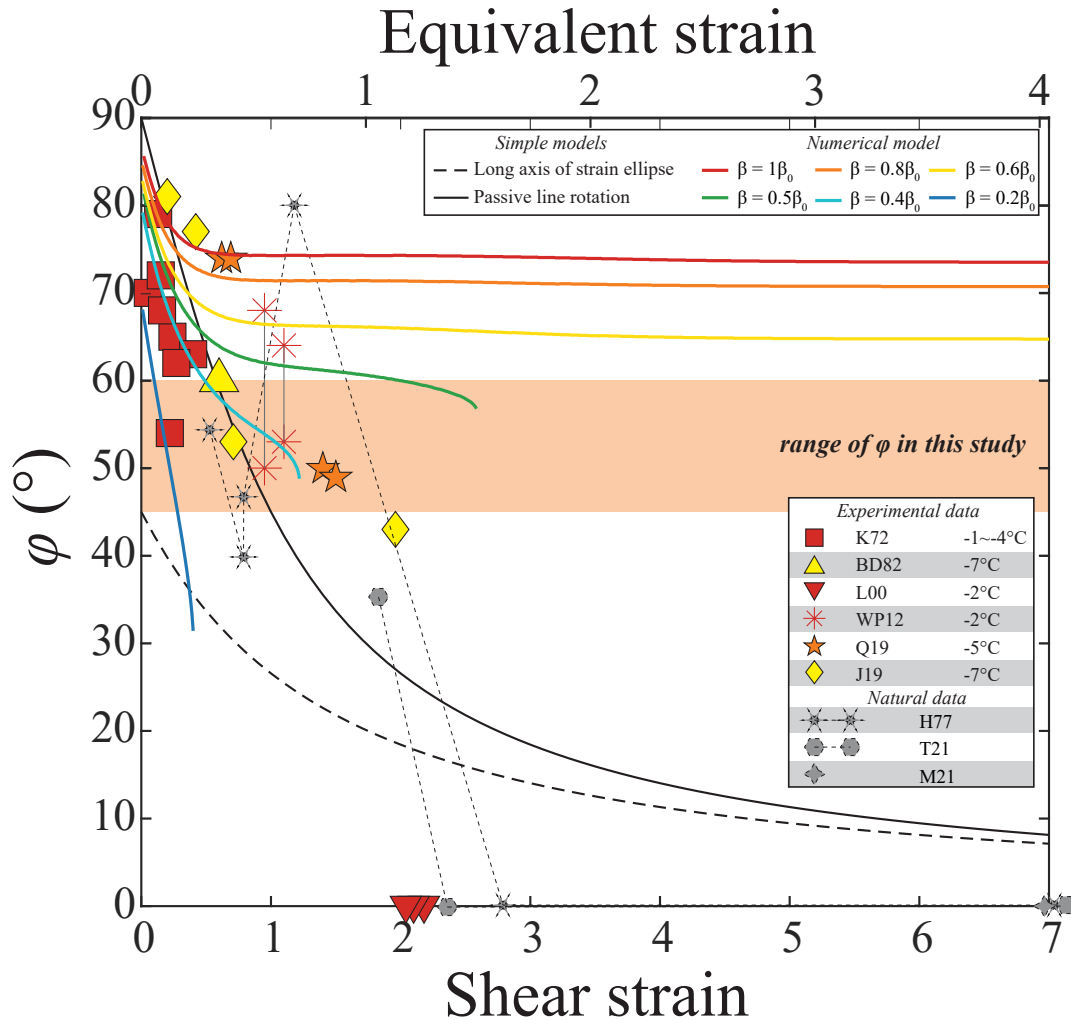
Figure 11. Plot of the angle between c-axis clusters, \phi , for experiments from this study, experiments from the literature, results of simple models and results of the numerical model. Since the nominal shear strains in this study cannot be directly compared with those in previous experimental studies, a range of \phi is marked by a shaded box in the plot, independent of strain. Experimental data are from the following studies: K72: Kamb (1972); BD82: Bouchez and Duval (1982); L00: Li et al. (2000); WP12: Wilson and Peternell (2012); Q19: Qi et al. (2019); J19: Journaux et al. (2019). Only experimental data at -5 \pm 4^\circ\text{C} were illustrated here. Symbol colors broadly indicate deformation temperature, with red, orange and yellow colors indicating > -5^\circ\text{C} , -5^\circ\text{C} and < -5^\circ\text{C} , respectively. Data from natural ice are as follows: H77: Hudleston (1977); T21: Thomas et al. (2021); M21: Monz et al. (2021). Symbols tied by lines indicate they are from one sample. The maximum strains for the natural samples were estimated to be larger than the scale of our experiments, and thus, three markers (M21, H77 and T21) were placed at the right end of the x-axis suggesting that their shear strains are larger than 7. Outcomes from the numerical model based on Richards et al. (2021) are marked by colored thick lines. The parameter, \beta , represents the rate of migration recrystallization in the model. The termination of these curves suggests that a single-cluster fabric forms.
