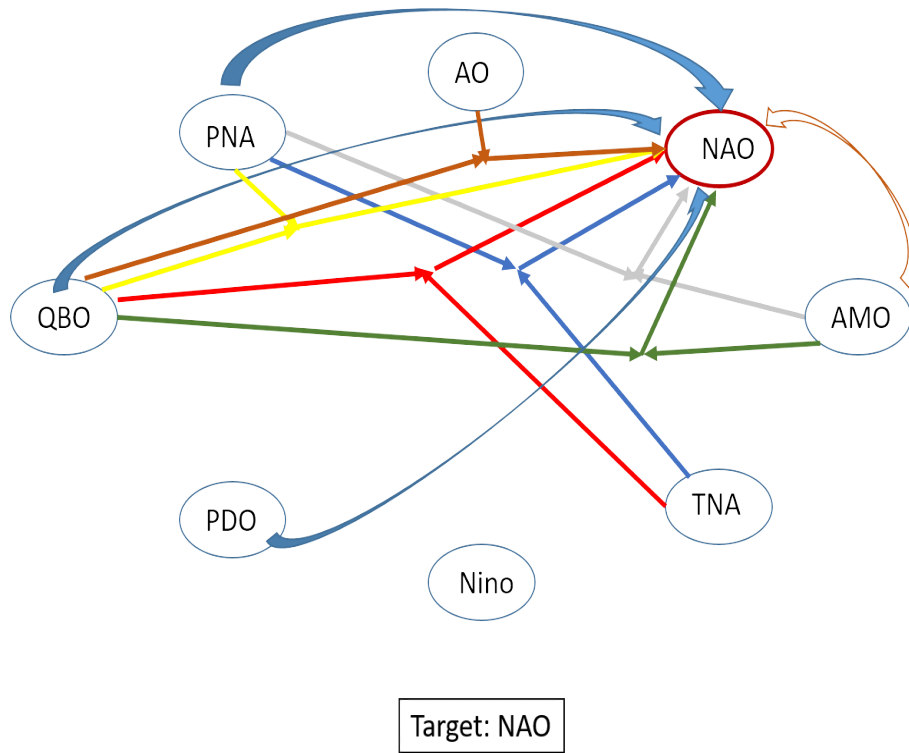
Figure 4. A visual representation of the linear and nonlinear influences from the set of indices to the NAO for the low-frequency variability dataset. the curved plain arrows refer to the linear influence, the triple straight arrows with the same colors refer to the influence of the quadratic nonlinearities: two straight arrows are emanating from two indices, joining somewhere in between the indices, and from there the third straight arrow indicates the target.
