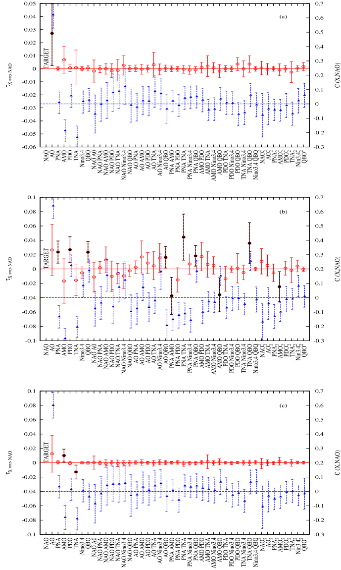
Figure 3. The rate of information transfer (left y-axis, red open circles) and the correlation (right y-axis, blue full triangles) are plotted as a function of the observables for the targeted observable (labelled TARGET in the plot): the NAO. Panels (a), (b) and (c) are for the original, the LFV and the high-frequency time series, respectively. The observable set is composed of 7 linear terms and 36 nonlinear quadratic terms, all listed along the x-axis. The points in black refer to the significant dependencies at the 1% level.
