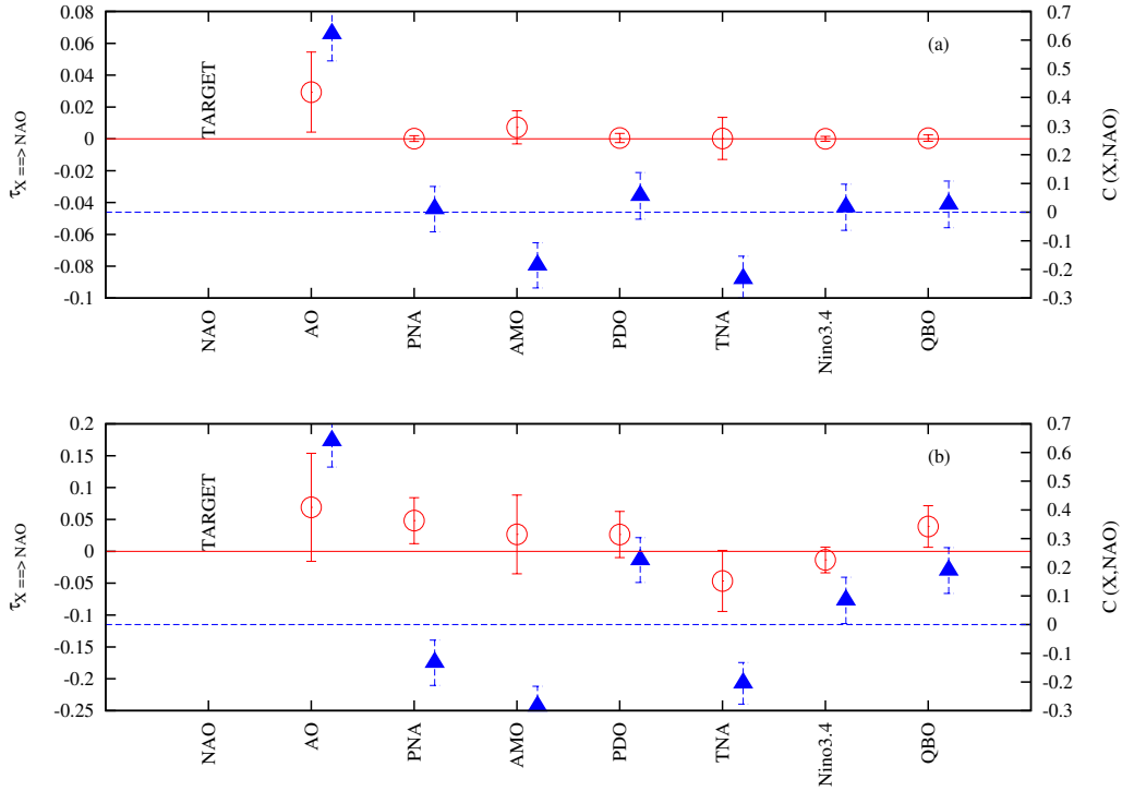
Figure 2. The rate of information transfer (left y-axis, red open circles) and the correlation (right y-axis, blue full triangles) are plotted as a function of the observables for the targeted observable (labelled TARGET in the plot): the NAO. Panels (a) and (b) are for the original and LFV time series, respectively.
