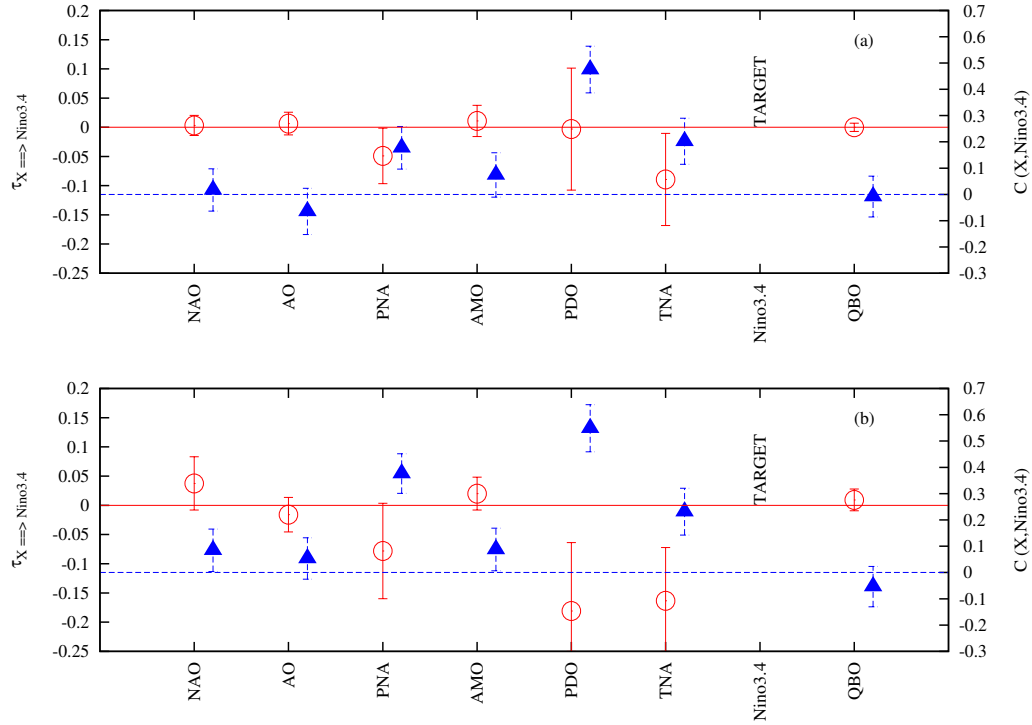
Figure 5. The rate of information transfer (left y-axis, red open circles) and the correlation (right y-axis, blue full triangles) are plotted as a function of the observables for the targeted observable (labelled TARGET in the plot): the Niño3.4. Panels (a) and (b) are for the original and LFV time series, respectively.
