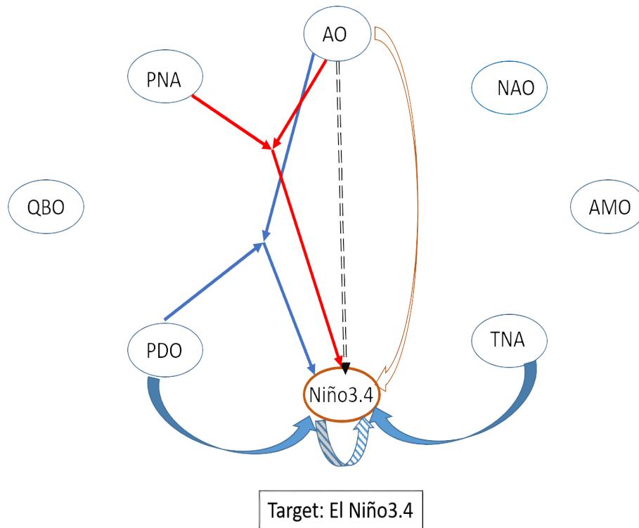
Figure 7. A visual representation of the linear and nonlinear influences from the set of indices to the El Niño3.4 for the low-frequency variability dataset. the curved plain arrows refer to the linear influence, the triple straight arrows with the same colors refer to the influence of the quadratic nonlinearities: two straight arrows are emanating from two indices, joining somewhere in between the indices, and from there the third straight arrow indicates the target. The double dashed straight (black) arrow indicates the influence of the product between the source and the target. The empty curved arrow indicates the quadratic influence of the source, while the striped curved arrow the quadratic influence of the target.
