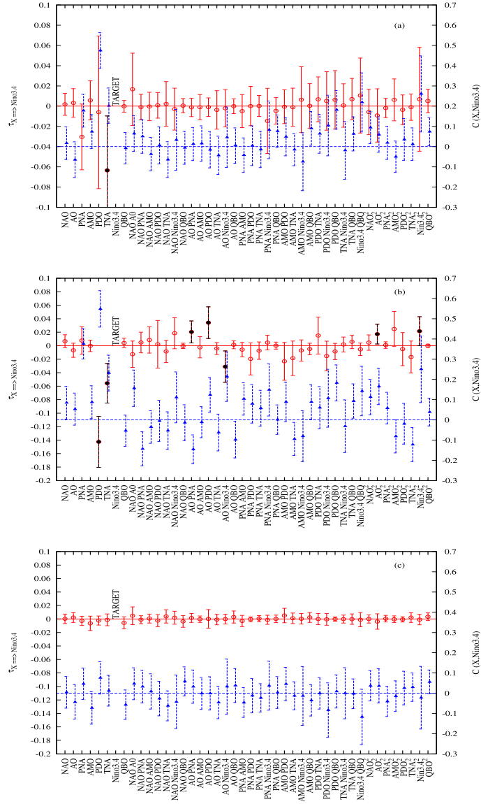
Figure 6. The rate of information transfer (left y-axis, red open circles) and the correlation (right y-axis blue full triangles) are plotted as a function of the observables for the targeted observable (labelled TARGET in the plot): the Niño3.4. Panels (a), (b) and (c) are for the original, the LFV and the high-frequency time series, respectively. The observable set is composed of 7 linear terms and 36 nonlinear quadratic terms, all listed along the x-axis. The points in black refer to the significant dependencies at the 1% level.
