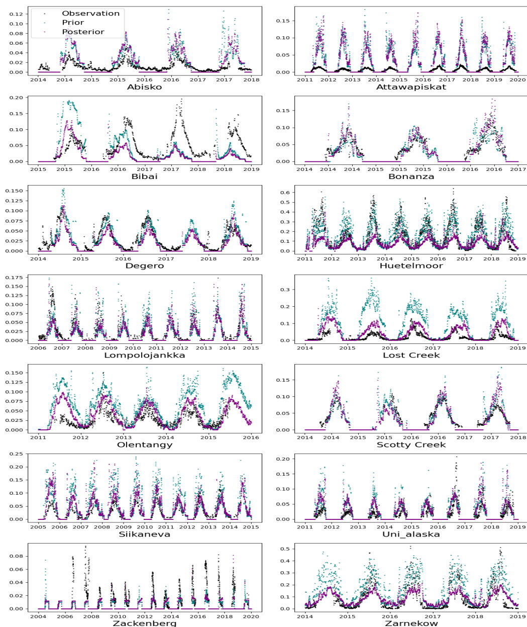
Figure 5. The CH 4 simulation from the LPJ-GUESS model from 14 different wetland sites (purple dots) after optimising with the GRaB-AM algorithm. The black dots are the real CH 4 flux observations from corresponding wetlands. The teal dots are the prior simulation with the prior model parameters used to start the MCMC chain. Three days of running averages are calculated from the original time series, and from most of the figure a few outliers on the vertical axis have been removed for better visualisation.
