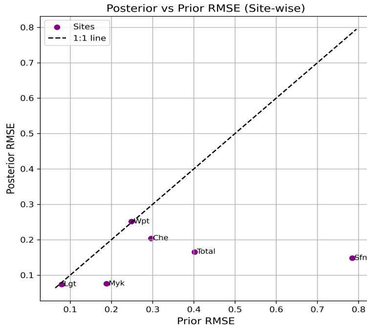
Figure 8. Scatterplot comparing prior and posterior RMSE values for each site. Each point represents one of the study sites. The 1:1 dashed line indicates no change in RMSE. Points below the line indicate improved model performance after assimilation.
