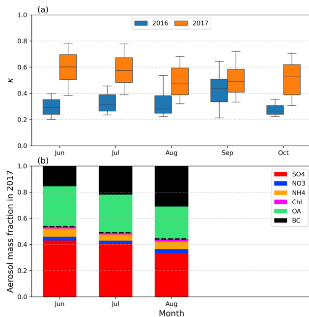
Figure 2. (a) Monthly distributions of \kappa values calculated at 0.1% supersaturation during the BB seasons of 2016 and 2017. The boxes represent the 25th, 50th (median), and 75th percentiles, while the whiskers extend to the 10th and 90th percentiles. (b) Monthly mean aerosol chemical mass fractions measured by ACSM and SP2 during the 2017 BB season. The black dashed line in (b) represents the separation between inorganic and organic fractions of the aerosol components.
