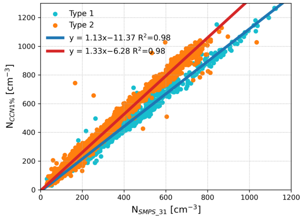
Figure 1. Correlations between the CCN concentration measured at 1% supersaturation ( N_{CCN1\%} ) and the integrated aerosol concentration with diameters from 31 to 1000 nm based on SMPS measurements ( N_{SMPS\_31} ). Two distinct correlations were identified in the data using the K-means clustering method, indicated by light blue and orange points. Type 1 (light blue) 130 includes data from June, July, September, and October of 2016, while Type 2 (orange) includes data from August 2016 and June to October 2017. The blue and red lines represent linear regressions fitted to each correlation type, respectively.
