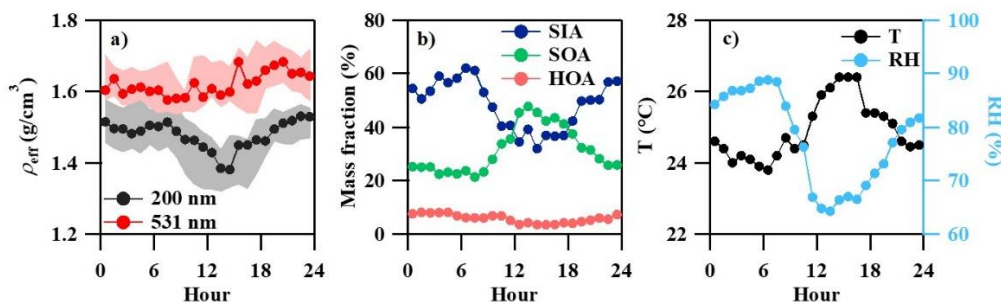
Figure 4 Diurnal variations in a) size-resolved \rho_{\text{eff}} , b) mass fractions of the main components and c) meteorological parameters during the whole observation period.
