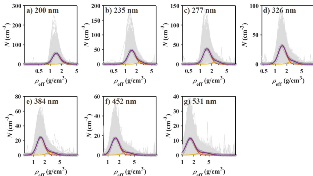
Figure 2: Averaged particle \rho_{\text{eff}} distributions at (a) 200 nm, (b) 235 nm, (c) 277 nm, (d) 326 nm, (e) 384 nm, (f) 452 nm, and (g) 531 nm. The gray lines represent the measured \rho_{\text{eff}} distributions. The red and yellow lines are the Gaussian fits of the average \rho_{\text{eff}} and the Gaussian fits of doubly charged particles, respectively. The purple line represents the sum of Gaussian fits.
