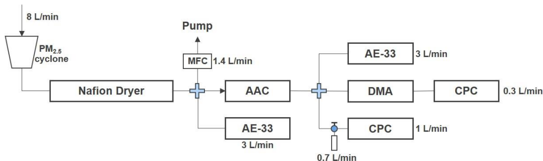
80 Figure 1: Instrumental setup used in this study. MFC: Mass flow controller.
