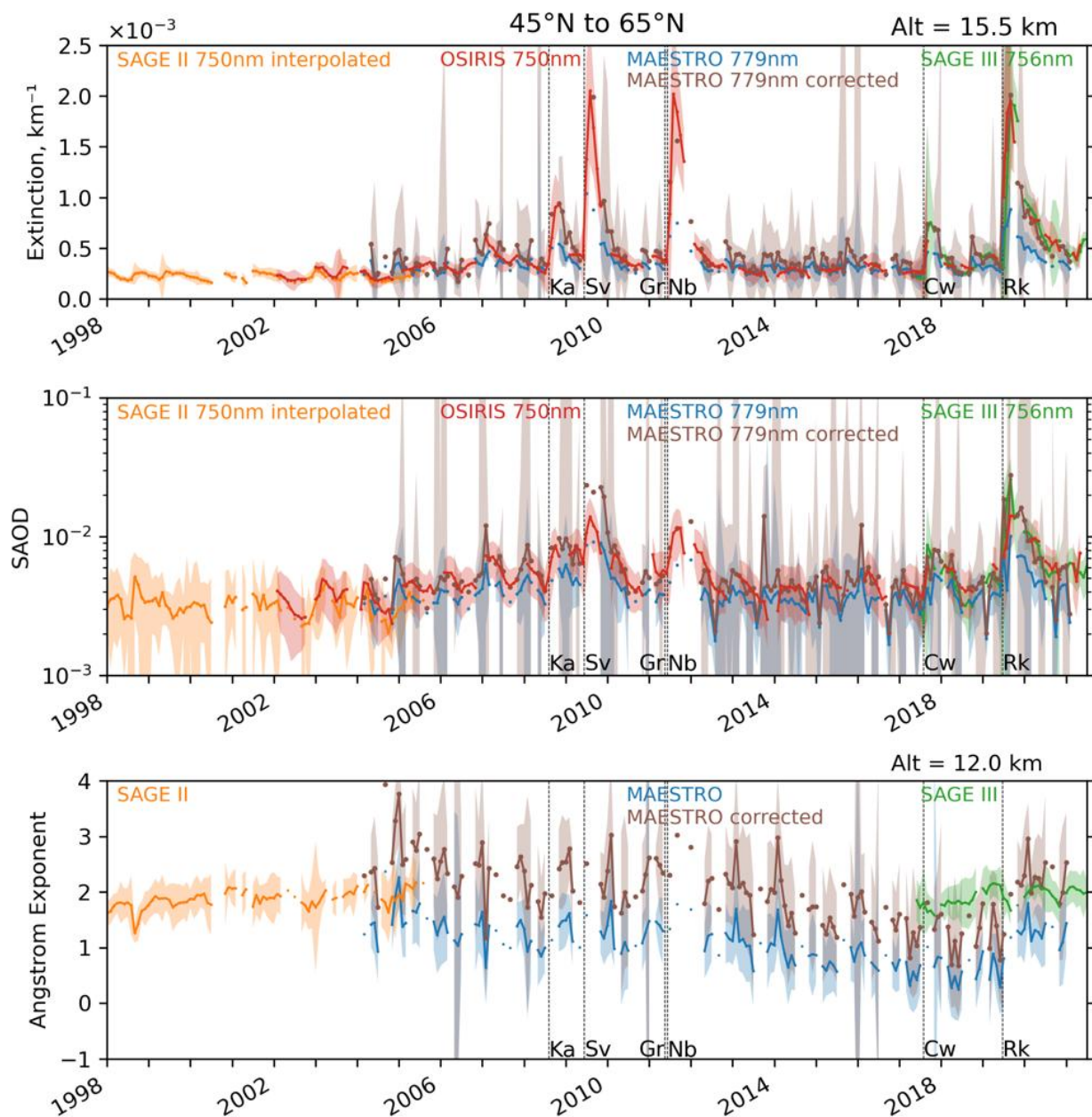
Figure 11: Comparison of median stratospheric aerosol extinction coefficients (top panel), SAOD (middle panel) and AE (bottom panel) between measurements from different instruments in northern midlatitudes. Shaded area represents \pm one standard deviation. Data in two 10-degree latitude bins are combined to show the time series by calculating the average of the medians. There is no AE data from OSIRIS because it is based on single 750 nm measurements. Selected wavelengths for each instrument are labelled. Selected altitude for extinction and AE plots is also labeled on the top right of each plot. For MAESTRO, values before and after correction are shown.
