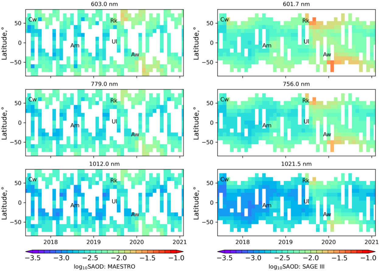
Figure 5: Monthly median SAOD derived from MAESTRO (left panel) and SAGE III (right panel) extinctions at three different wavelengths as a function of latitude and time. Labels Cw, Am, Rk, Ul and Aw mark the latitude and dates of the Canadian wildfires, the Ambae, Raikoke and Ulawun eruptions, and the Australian wildfires, respectively.
