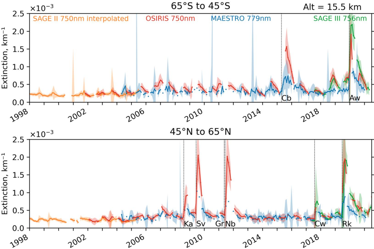
Figure 3: Comparison of monthly zonal median extinction coefficients measured by SAGE II, OSIRIS, MAESTRO, and SAGE III at an altitude of 15.5 km in the midlatitudes of the (top) SH and (bottom) NH. Shaded area represents \pm one standard deviation. Data in two 10-degree latitude bins are combined to show the timeseries by calculating the average of the medians. Dotted vertical lines correspond to the time when notable volcanic eruptions or wildfires occurred within or near respective latitude ranges. They represent Calbuco (Cb, 41°S) and the Australian Wildfires (Aw) in the SH and Kasatochi (Ka, 52°N), Sarychev (Sv, 48°N), Grimsvothn (Gr, 64°N), Nabro (Nb, 13°N), the Canadian Wildfires (Cw) and Raikoke (Rk, 48°N) in the NH. Although Nabro was a tropical eruption, it is shown here because it impacted the high latitudes in the NH. Note the multiplicative factor of 10^{-3} (shown above y-axis) used to get the extinction coefficients in units of 1/km.
