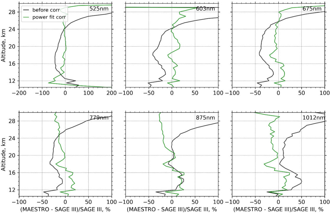
410 Figure 10: Coincident comparison of MAESTRO aerosol extinction measurements with SAGE III. Lines show the median of differences computed as (\text{MAESTRO} - \text{SAGE III})/\text{SAGE III} . Black lines show the median of differences for the raw data, while green lines show the same for the data after the correction of Sec. 4.1 is applied to the MAESTRO data.
