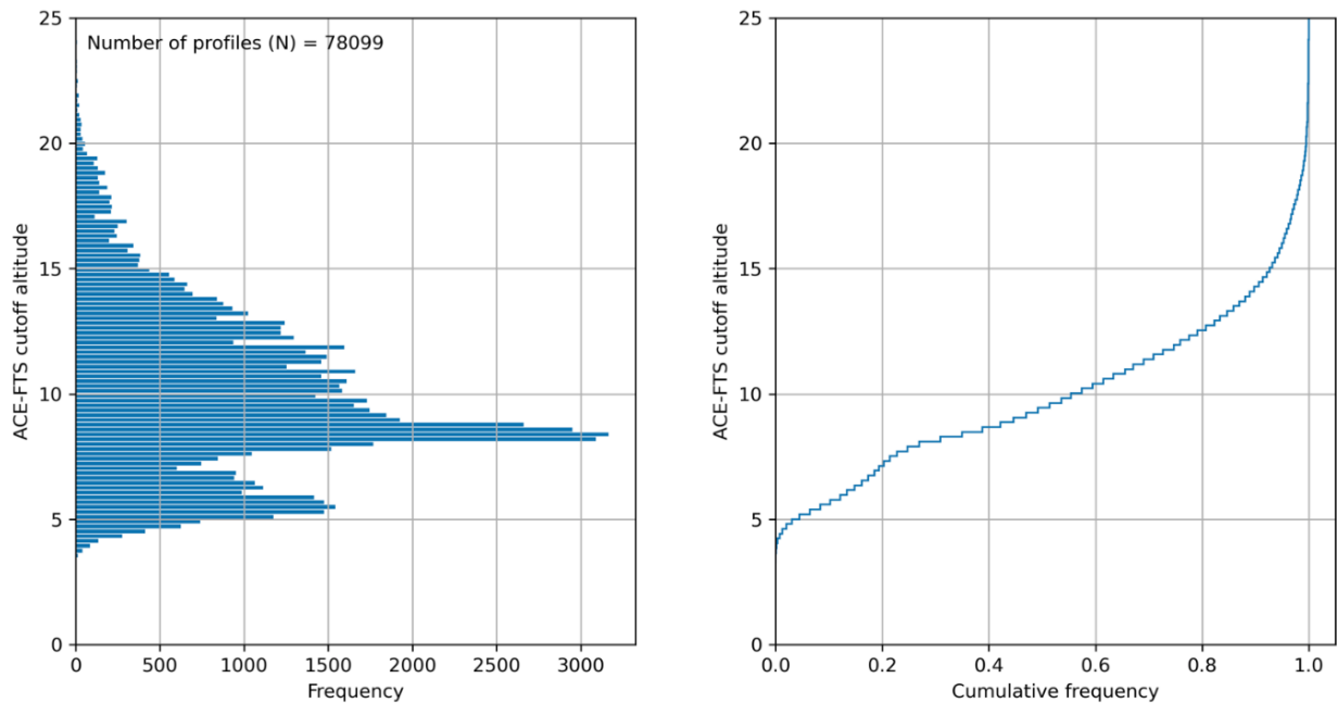
455 Figure 11: Frequency distribution of the number of MAESTRO profiles with the corresponding ACE-FTS cutoff altitude (left panel) and corresponding cumulative frequency distribution (right panel).
