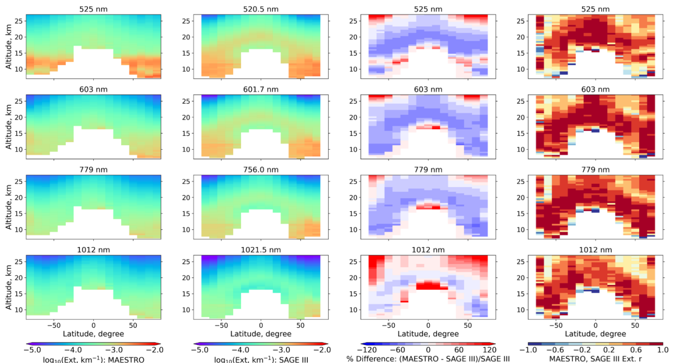
Figure 4: Median extinction coefficient from the full MAESTRO (first column) and SAGE III (second column) data sets at four different wavelengths during their overlap period from June 2017 to February 2021, shown as a function of altitude and latitude. The data is binned in 10^\circ latitude bins. The third column shows the percentage difference (\text{MAESTRO} - \text{SAGE III})/\text{SAGE III} in extinction coefficients compiled from the two instrument data sets. The fourth column shows the Pearson's correlation coefficients between MAESTRO and SAGE III extinction coefficients.
