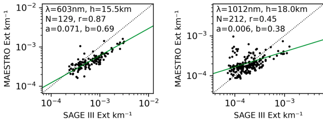
Figure 8: Scatterplot in log-scale showing the MAESTRO and SAGE III extinction coefficients at 603 nm and an altitude of 15.5 km (left panel) and at 1012 nm and an altitude of 18.0 km (right panel). Each point represents the median extinction value for each instrument within a 10-degree latitude bin and for a single month, where and when both instruments have measurements. Number of data points and the Pearson's correlation coefficient is also shown. Green line represents the power-law regression line whose scaling and exponent parameters are given by 'a' and 'b' respectively. The dotted black line is the one-to-one line.
