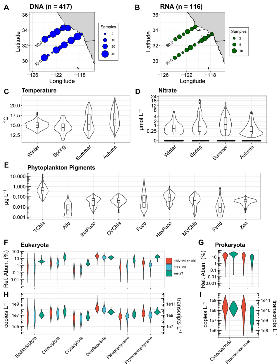
135 Figure 1. Overview of CalCOFI samples used in this study. (A, B) Locations and quantity of samples for DNA and RNA with corresponding phytoplankton pigment samples. (C, D) Temperature ( ^{\circ}\text{C} ) and nitrate concentrations ( \mu\text{mol L}^{-1} ) across seasons for the paired DNA and pigment samples used here. Corresponding data for the RNA samples are shown in Fig. S1. Nitrate concentrations are shown on a cube-root scale. (E) Phytoplankton pigment concentrations. Pigment abbreviations: TChla, total 140 chlorophyll a ; Allo, alloxanthin; ButFuco, 19'-butanoyloxyfucoxanthin; DVChla, divinyl chlorophyll a ; Fuco, fucoxanthin; HexFuco; 19'-hexanoyloxyfucoxanthin; MVChlb, monovinyl chlorophyll b ; Perid, Peridinin; Zea, zeaxanthin. (F, G) Relative abundances of different phytoplankton groups using 18S-V4 rRNA gene (red), 18S-V9 rRNA gene (blue), or transcript (metaT, green) abundances. For prokaryota, the 16S V4-V5 region was used and is shown in red. (H, I) Absolute abundances for 18S or 16S rRNA genes (copies \text{L}^{-1} , left y-axis) and transcripts (transcripts \text{L}^{-1} , right y-axis). Different metrics are colored as in panels F and G.
