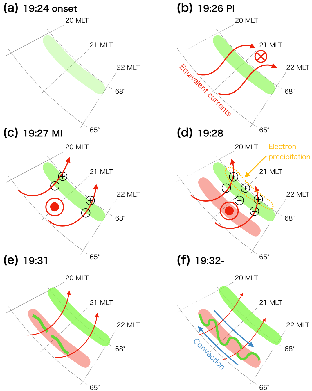
Figure 6. Schematic illustration of the relative locations of pre-existing arc, red diffuse aurora, and secondary arc. The coordinates of auroras were calculated by assuming the altitudes of green and red emissions were at 100 km and 250 km, respectively. The blue arrows indicate the convection directions suggested by the vortex motion of the secondary arc.
