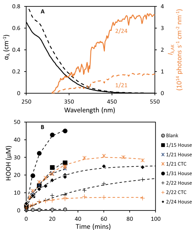
Figure 1. (A) Absorbance spectra of two representative extracts (black lines) and their corresponding midday total (downwelling and upwelling) actinic fluxes in Fairbanks, Alaska (orange lines). Dashed and solid lines represent values for the composite samples of 1/21 and 2/24, respectively. (B) Examples of HOOH photoformation in PM extracts during solar simulator illumination in the lab. Rates for each extract, normalized to a standard photon flux ( j_{2NB} = 0.020 \text{ s}^{-1} ), are listed in Table S3.
