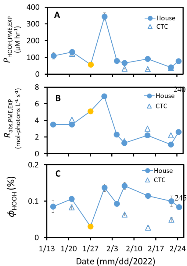
250 Figure 2. (A) Experimentally measured photoformation rates of HOOH in aqueous extracts of PM collected from the House (filled circles) and CTC (open triangles) sites, normalized to a constant photon flux of j_{2\text{NB}} = 0.020 \text{ s}^{-1} . Blue symbols are pH 1 extracts, while the gold symbol is pH 4. (B) Rate of light absorption in the extracts under our standard laboratory simulated sunlight. (C) Quantum yield of HOOH formation. Error bars for panels A and C are 1 standard error, determined from the kinetic fit of the experimental data (panel A) or propagated from this error (panel C). There are no errors shown in panel B, but these are expected to be smaller than the symbols, i.e., \text{RSE} < 5\% .
