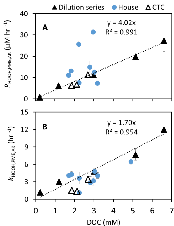
350 Figure 5. Results from the dilution experiment for the 2/14 CTC pH 1 composite (filled triangles) shown with results from the other pH 1 CTC (open triangles) and House (blue circles) composites. (A) Photoformation rate of HOOH as a function of DOC concentration (as a proxy for extract concentration). The 1/31 House sample is outside the plot boundaries, at 4.9 mM DOC and P_{\text{HOOH,PME,AK}} = 71 \mu\text{M hr}^{-1} , and so is not shown. (B) Rate constant for loss of HOOH versus DOC. The dotted lines in the two panels represent linear regression fits (with y intercepts fixed at zero) to just the dilution series data (filled triangles). Error bars on points represent 1 standard error from the kinetic fits of the experimental data.
