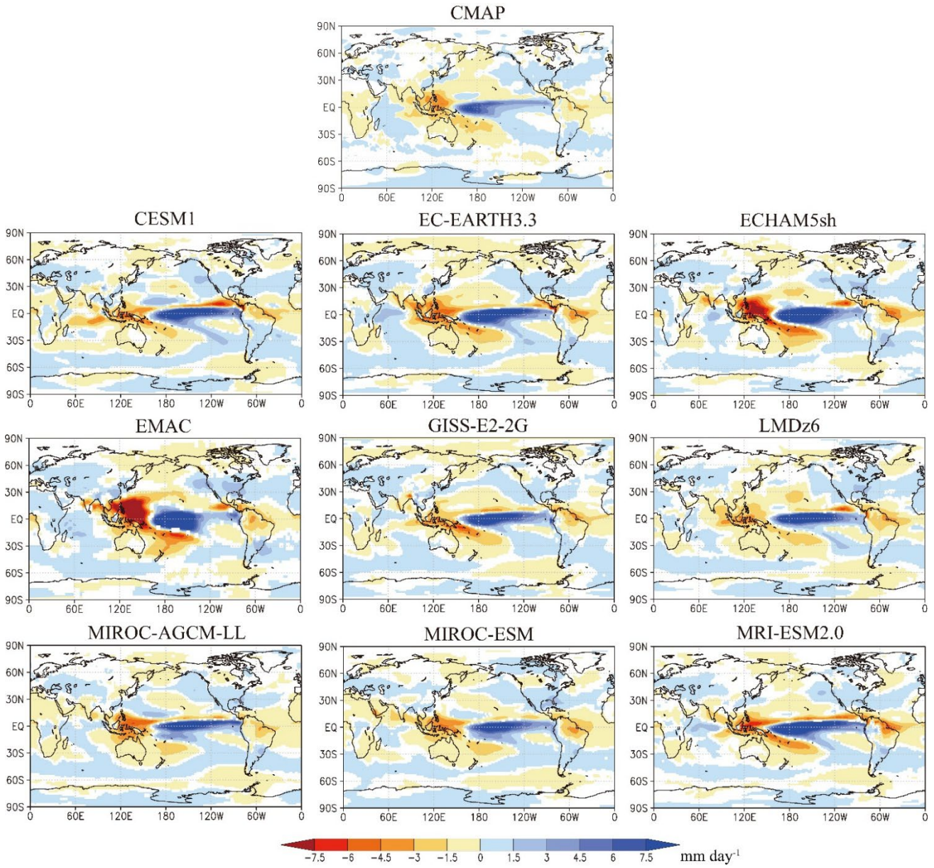
Fig. 8. Climatological annual mean precipitation differences for El Niño minus La Niña conditions for (center-top) CMAP and (others) individual models. Differences with absolute values \geq 0.1 \text{ mm day}^{-1} are shaded in CMAP, and those with a statistical confidence \geq 95\% are shaded for models.
