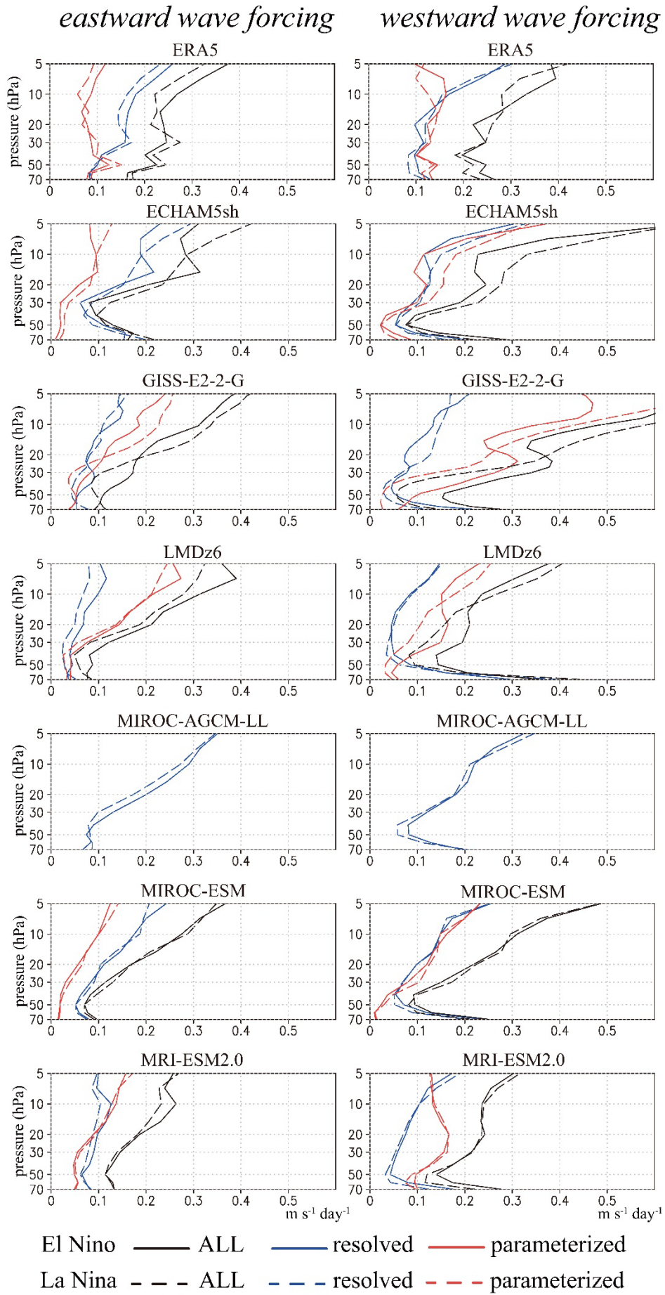
780 Fig. 13: Vertical profiles of the 10°S–10°N averaged wave forcing of the zonal mean flow from (blue) resolved forcing, (red) parameterized non-orographic gravity waves and (black) their sum. Solid and dashed lines correspond to El Niño and La Niña runs. Note that in ERA5, the parameterized forcing includes not only non-orographic gravity waves but also other types of zonal forcing.
