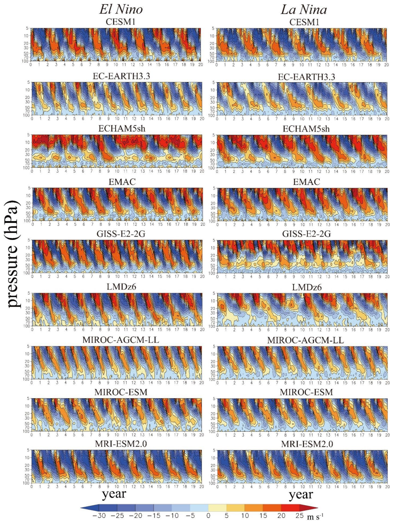
Figure 2: Time-height sections of the monthly mean, zonal mean zonal wind over the equator in the (left) El Niño and (right) La Niña runs for each model. Results from the first 20 years of one ensemble member for each model are shown. Model names are noted above each panel. The contour interval is 5 \text{ m s}^{-1} .
