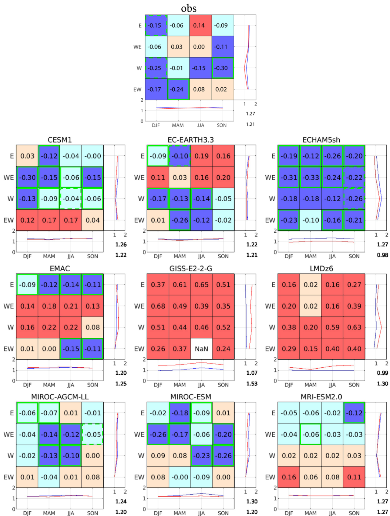
470 Fig. 6: Same as Fig. 5, but for QBO amplitude, defined as the distance from the origin in the two-dimensional phase space constructed from the first two EOF components of equatorial zonal wind anomalies. Red (blue) shading indicates stronger (weaker) amplitude during El Niño. Mean values and composite lines follow the same format as in Fig. 5.
