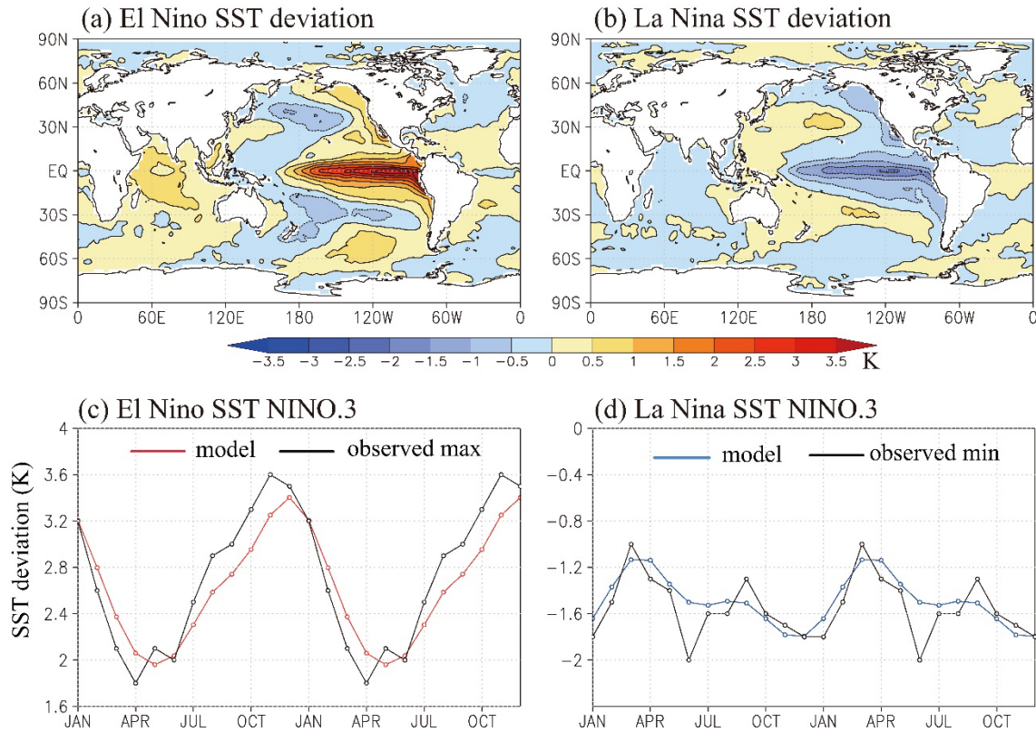
240 Figure 1: Annual mean composite SST deviations from climatology for the (a) El Niño and (b) La Niña composites. The contour interval is 0.5 K. The annual cycle of NINO.3 (5°S-5°N, 90°W-150°W) SST deviation from climatology for our (c) El Niño (red line) and (d) La Niña (blue line) composites. Black lines represent the maximum/minimum observed monthly values during 1950-2016. For visualization, two full repeating cycles are shown.
