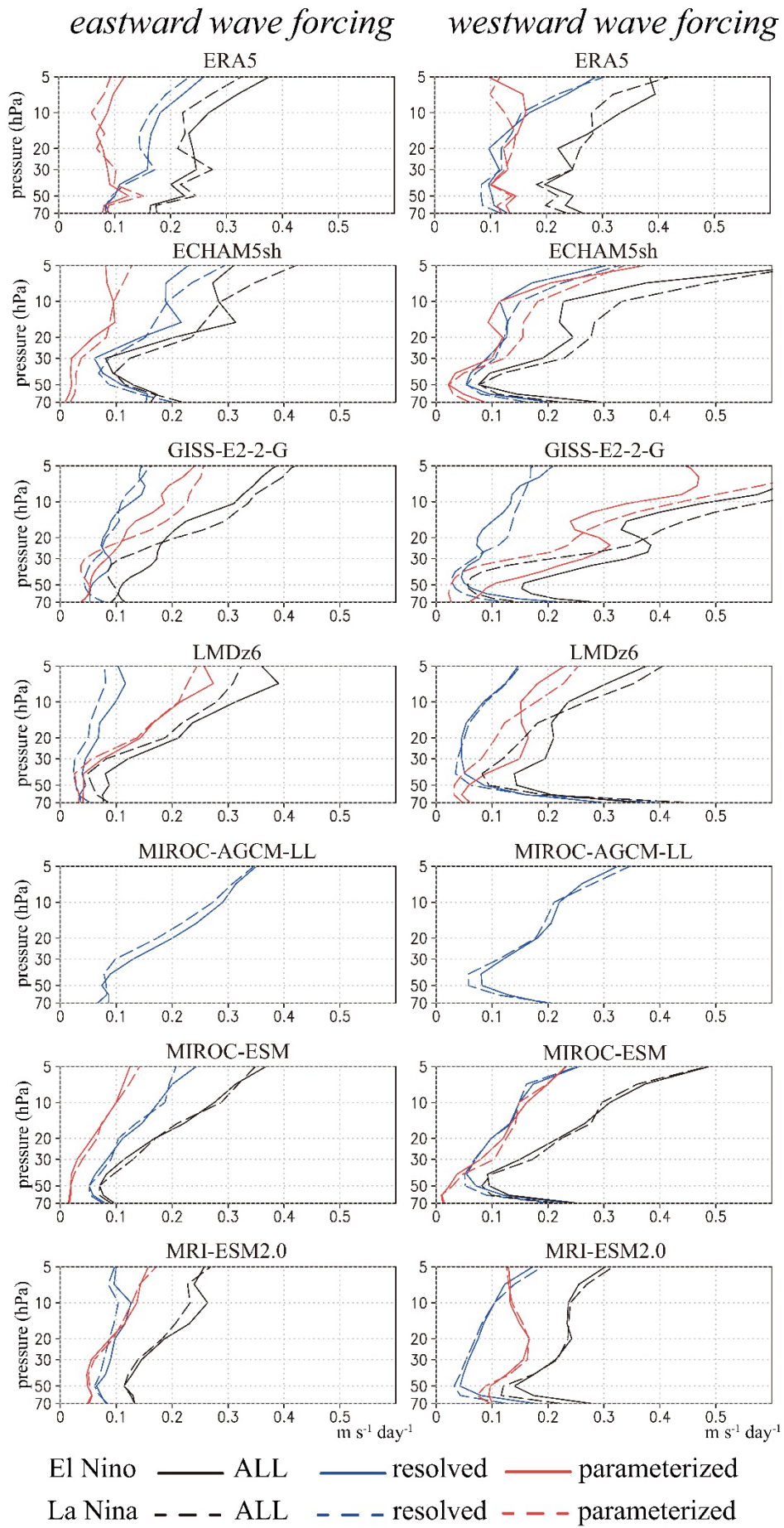
785 Fig. 13: Vertical profiles of the 10°S–10°N averaged wave forcing of the zonal mean flow from (blue) resolved forcing, (red) parameterized non-orographic gravity waves and (black) their sum. Solid and dashed lines correspond to El Niño and La Niña runs. Note that in ERA5, the parameterized forcing includes not only non-orographic gravity waves but also other types of zonal forcing.
