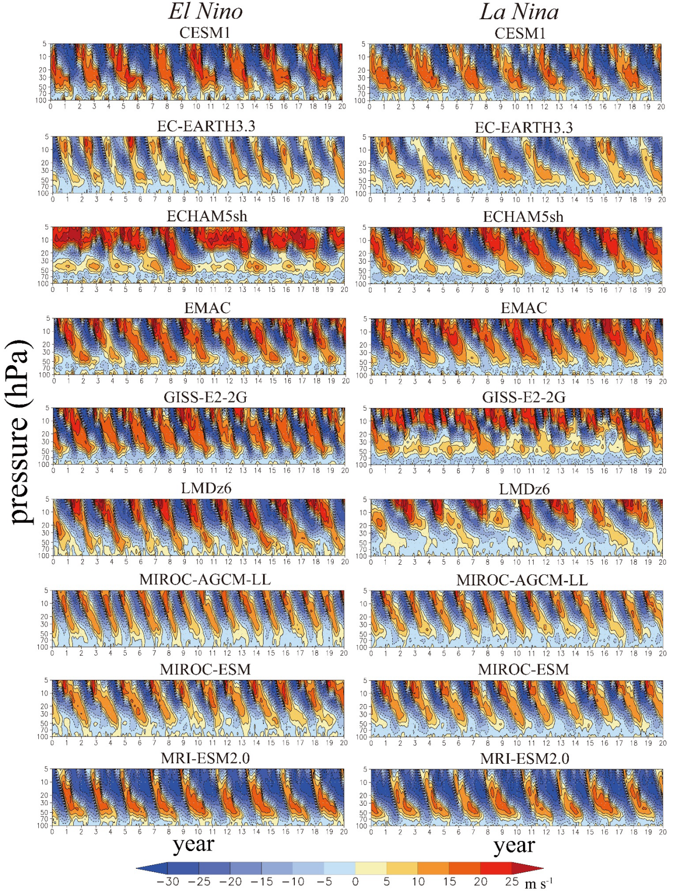
Figure 2: Time-height sections of the monthly mean, zonal mean zonal wind over the equator in the (left) El Niño and (right) La Niña runs for each model. Results from the first 20 years of one ensemble member for each model are shown. Model names are noted above each panel. The contour interval is 5 m s -1 .
