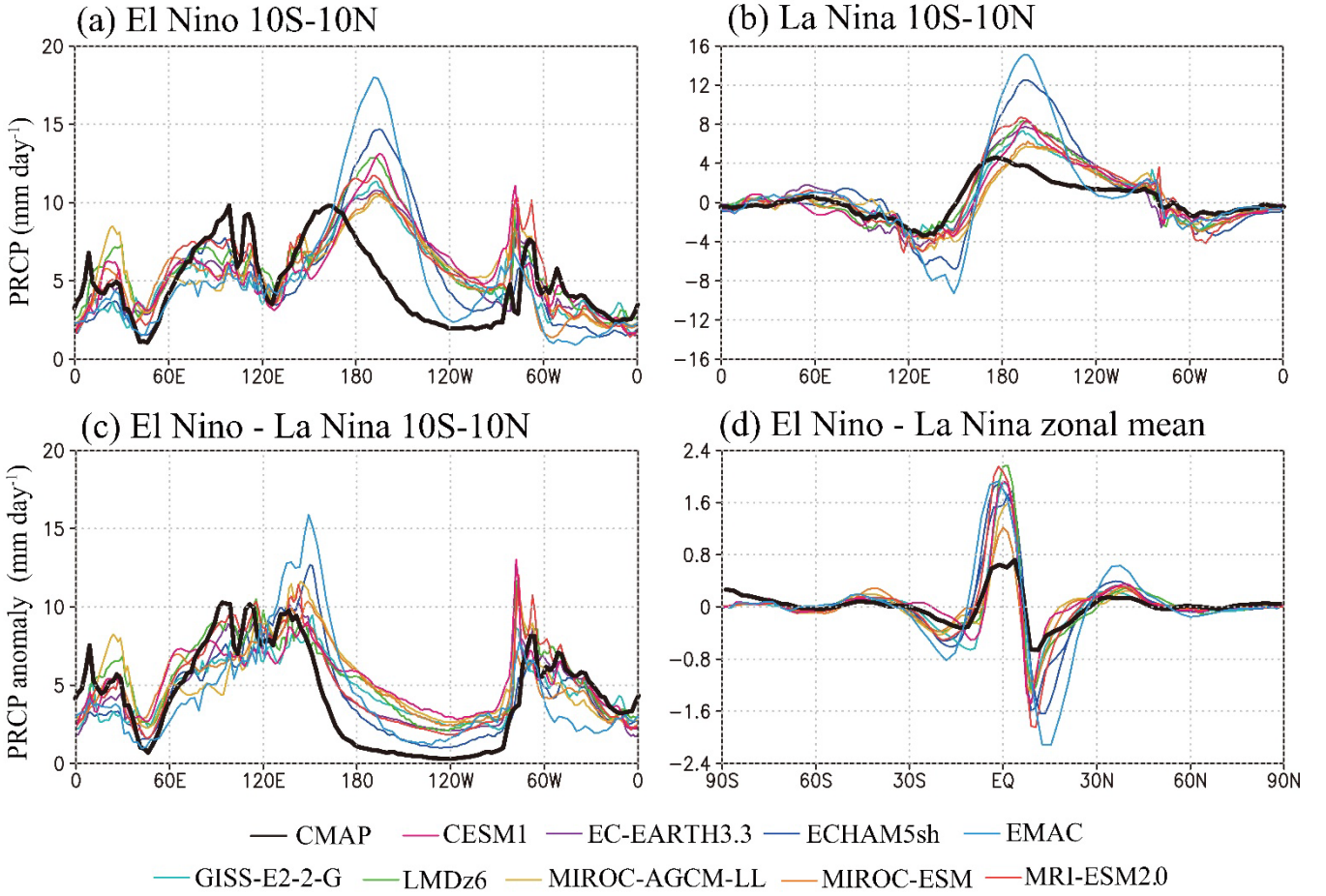
550 Fig. 9. Longitudinal variations of annual mean precipitation averaged over 10°N–10°S in (a) El Niño conditions, (b) La Niña conditions and (c) their differences. (d) Latitudinal variations of zonal mean El Niño minus La Niña precipitation differences. Black line shows CMAP observations and color lines display results for the individual models.
