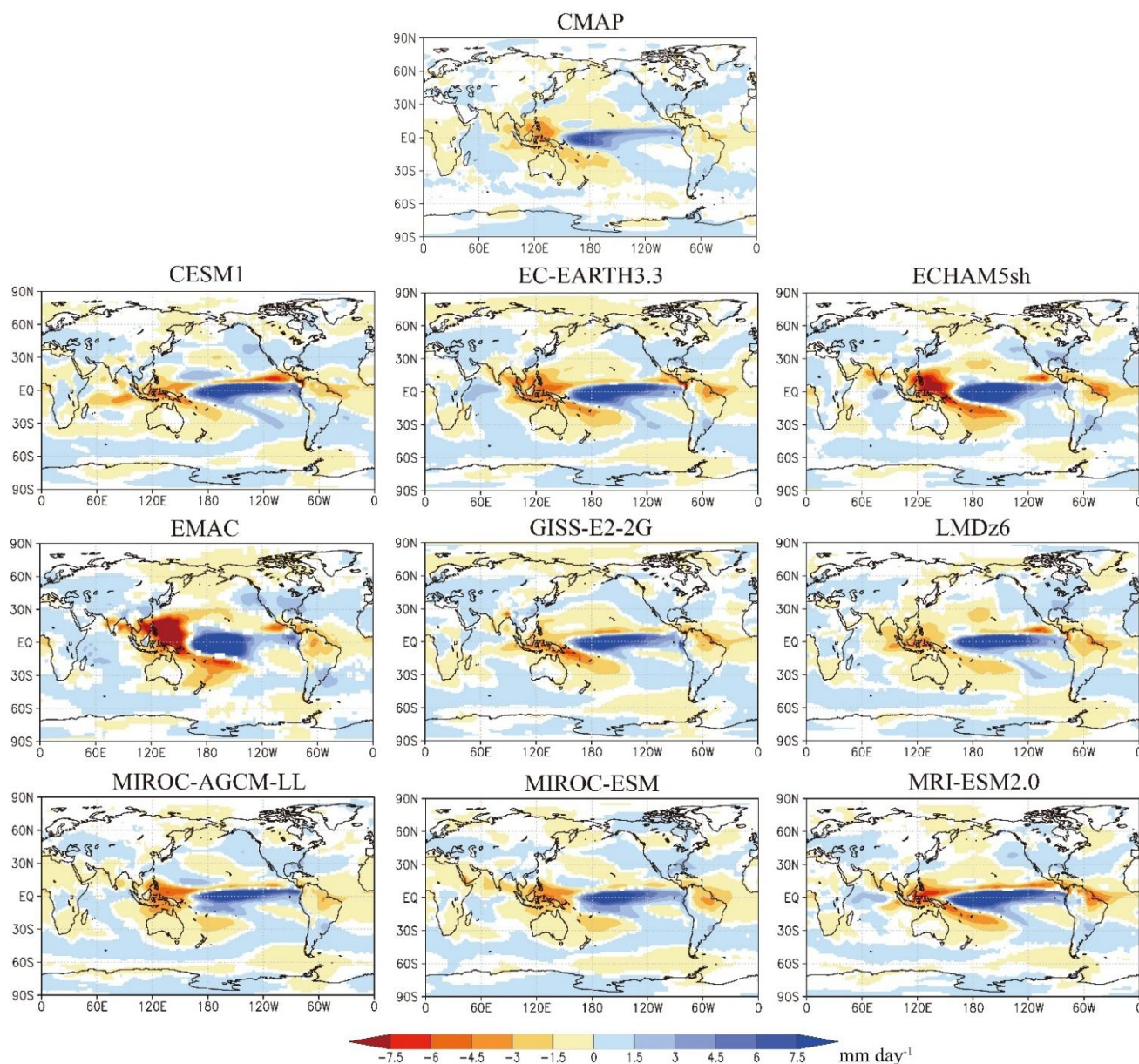
535 Fig. 8. Climatological annual mean precipitation differences for El Niño minus La Niña conditions for (center-top) CMAP and (others) individual models. Differences with absolute values \geq 0.1 \text{ mm day}^{-1} are shaded in CMAP, and those with a statistical confidence \geq 95\% are shaded for models.
