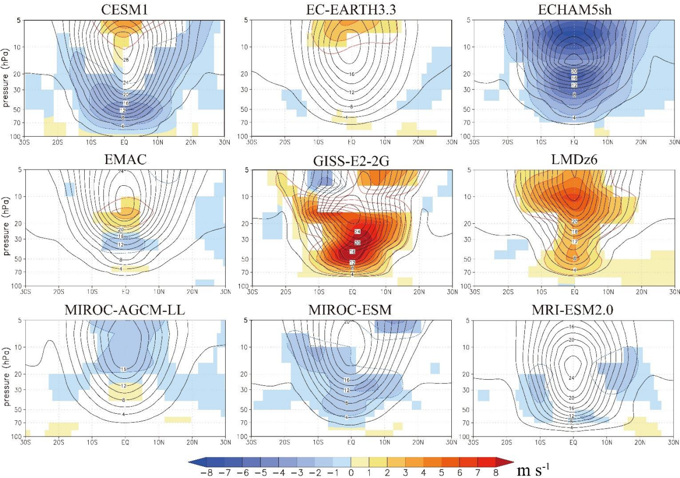
385 Fig. 4: Contours show the latitude-height cross sections of the mean QBO amplitude in El Niño runs, with intervals of 2 m s -1 . The El Niño minus La Niña QBO amplitude differences are shown with colored shading with interval of 1 m s -1 . Color shading is shown only where the differences have a statistical confidence \geq 95\% .
