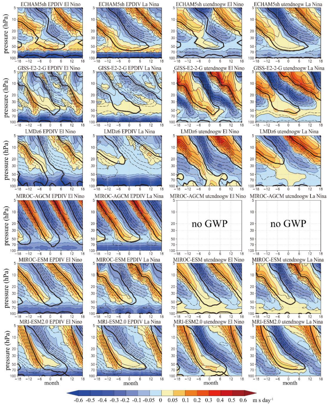
Fig. 12: The contours in each panel show the QBO cycle composites of the zonal mean zonal wind averaged over 10°S–10°N for one model in either El Niño (columns 1 and 3) or La Niña (columns 2 and 4) experiments. The color shading in columns 1 and 2 shows the EP flux divergence from resolved motions averaged over 10°S–10°N. The color shading in columns 3 and 4 shows the mean flow forcing from the non-orographic gravity wave drag parameterizations also averaged over 10°S–10°N. The QBO composite in each case is made relative to month zero which corresponds to the westerly-to-easterly phase transition of the zonal wind at 20 hPa. The contour interval is 5 m s -1 . The color intervals are ±0.05, 0.1, 0.15, 0.2, 0.3, 0.4, and 0.5 m s -1 day -1 .
