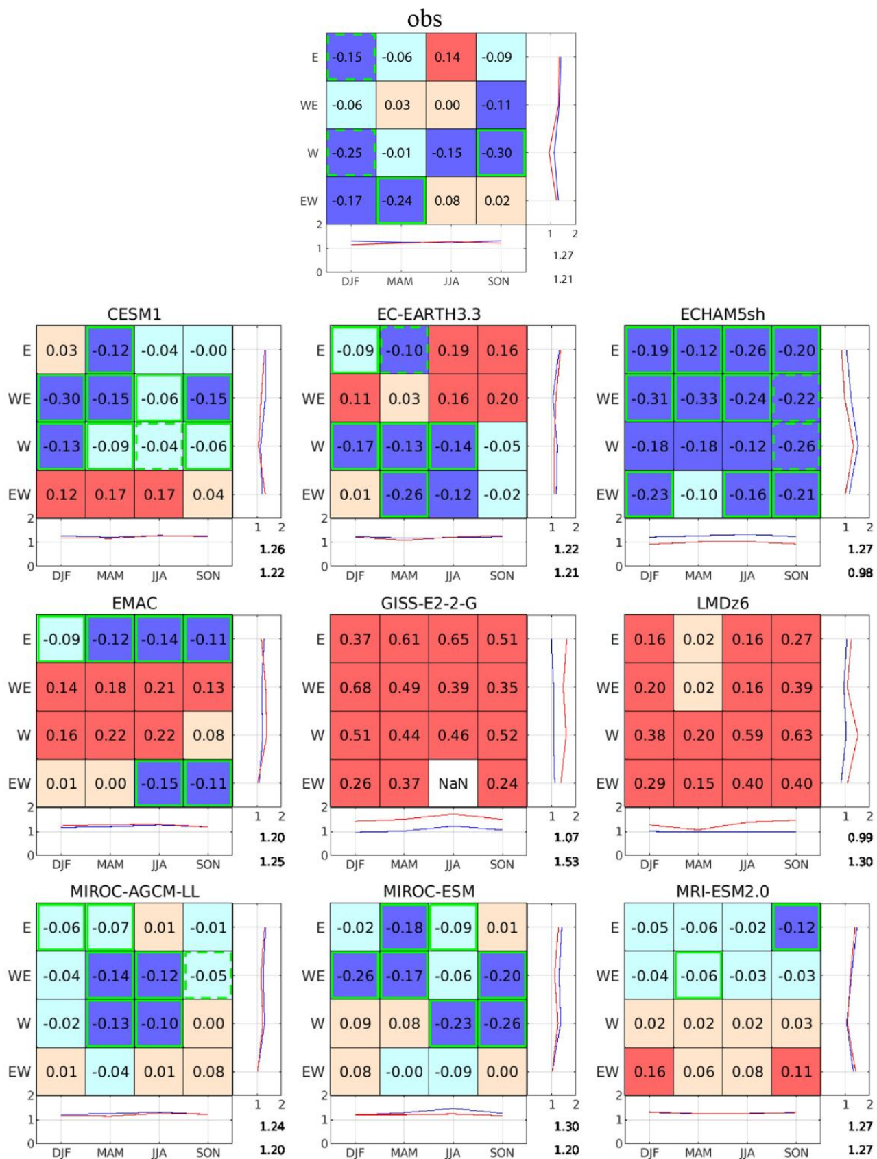
480 Fig. 6: Same as Fig. 5, but for QBO amplitude, defined as the distance from the origin in the two-dimensional phase space constructed 485 from the first two EOF components of equatorial zonal wind anomalies. Red (blue) shading indicates stronger (weaker) amplitude during El Niño. Mean values and composite lines follow the same format as in Fig. 5.
