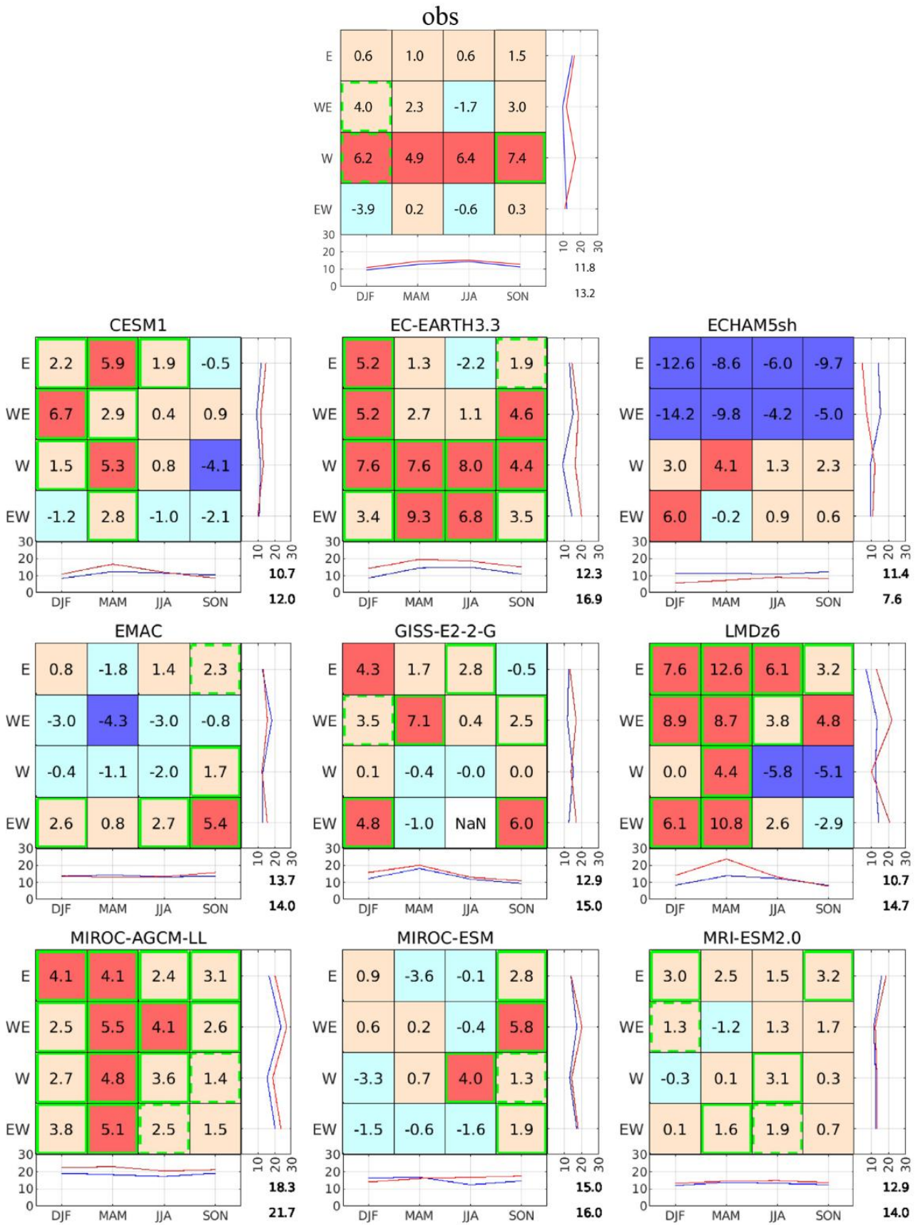
Fig. 5: Composite differences in QBO phase progression rate (unit: degrees per month) between El Niño and La Niña conditions, classified by QBO phase at 50 hPa and season. The top-center panel shows results from radiosonde observations, and the remaining panels show outputs from nine QBOi models. Red (blue) shading indicates faster (slower) phase progression during El Niño. Green outlines denote statistically significant differences at the 90 % confidence level. Right and bottom subpanels show seasonal and QBO-phase averages, respectively. The two values in the lower-right corner indicate mean values for La Niña (top) and El Niño (bottom), and the line plot shows their distributions (blue for La Niña, red for El Niño).
