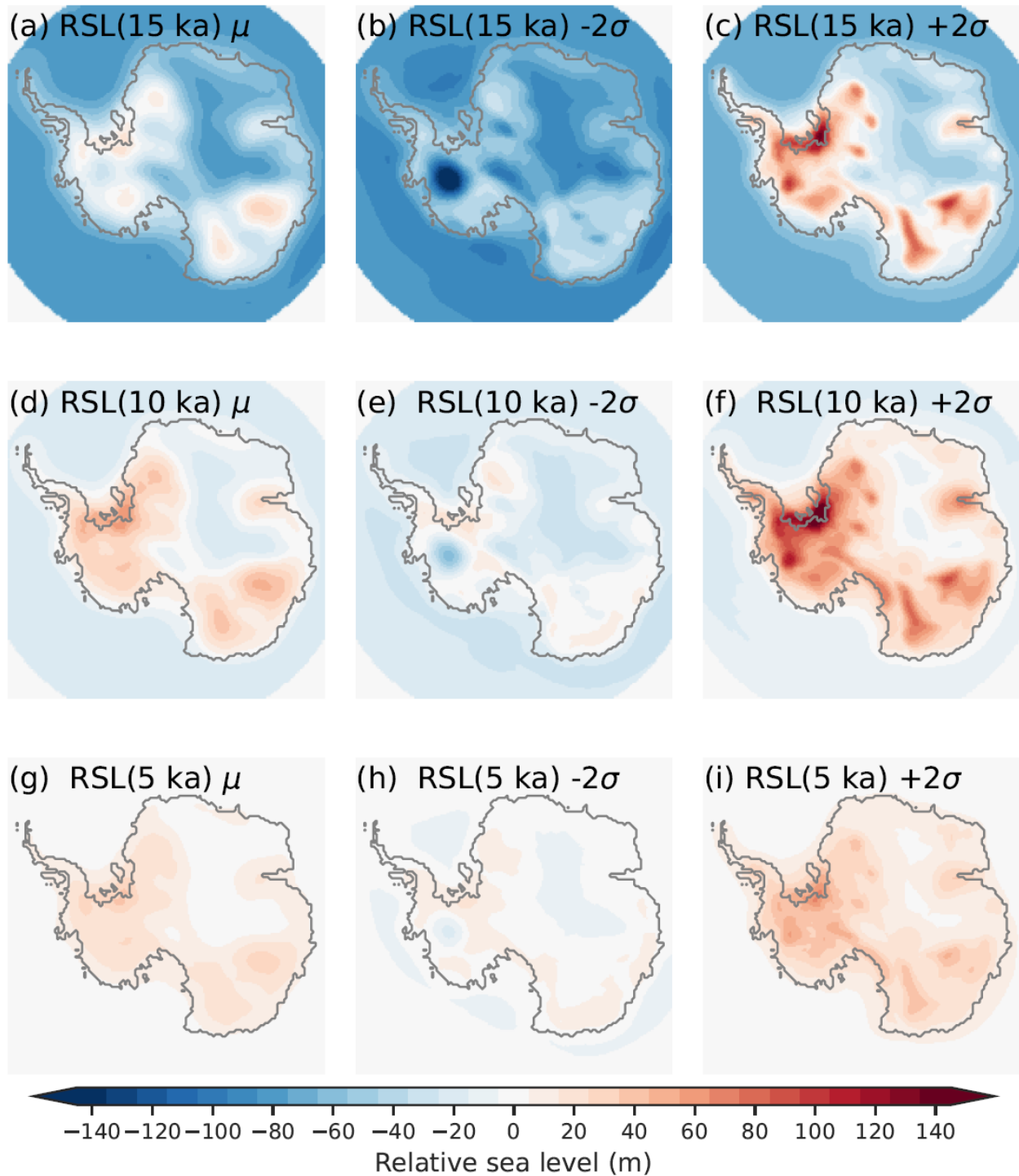
580 Figure 4: The not-ruled-out-yet (NROY) sub-ensemble mean (left), minus 2\sigma (middle), and plus 2\sigma (right) regional Antarctic RSL during the deglaciation at 15 ka (top), 10 ka (middle), and 5 ka (lower). The 2\sigma ranges are the nominal 95% ensemble intervals based on the equivalent Gaussian quantiles.
