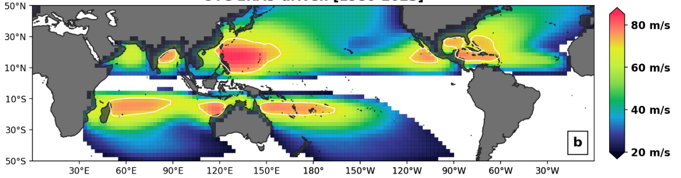
Fig. 10: 2.5-degree resolution map of (a) peak 1-min sustained winds recorded in IBTRACS over the 1980-2023 period and (b) expected 44-year peak sustained winds from the ERA5-driven UTC stochastic set (110'000 years of activity). The white contours represent the 70 m/s wind level (Cat5 threshold).
