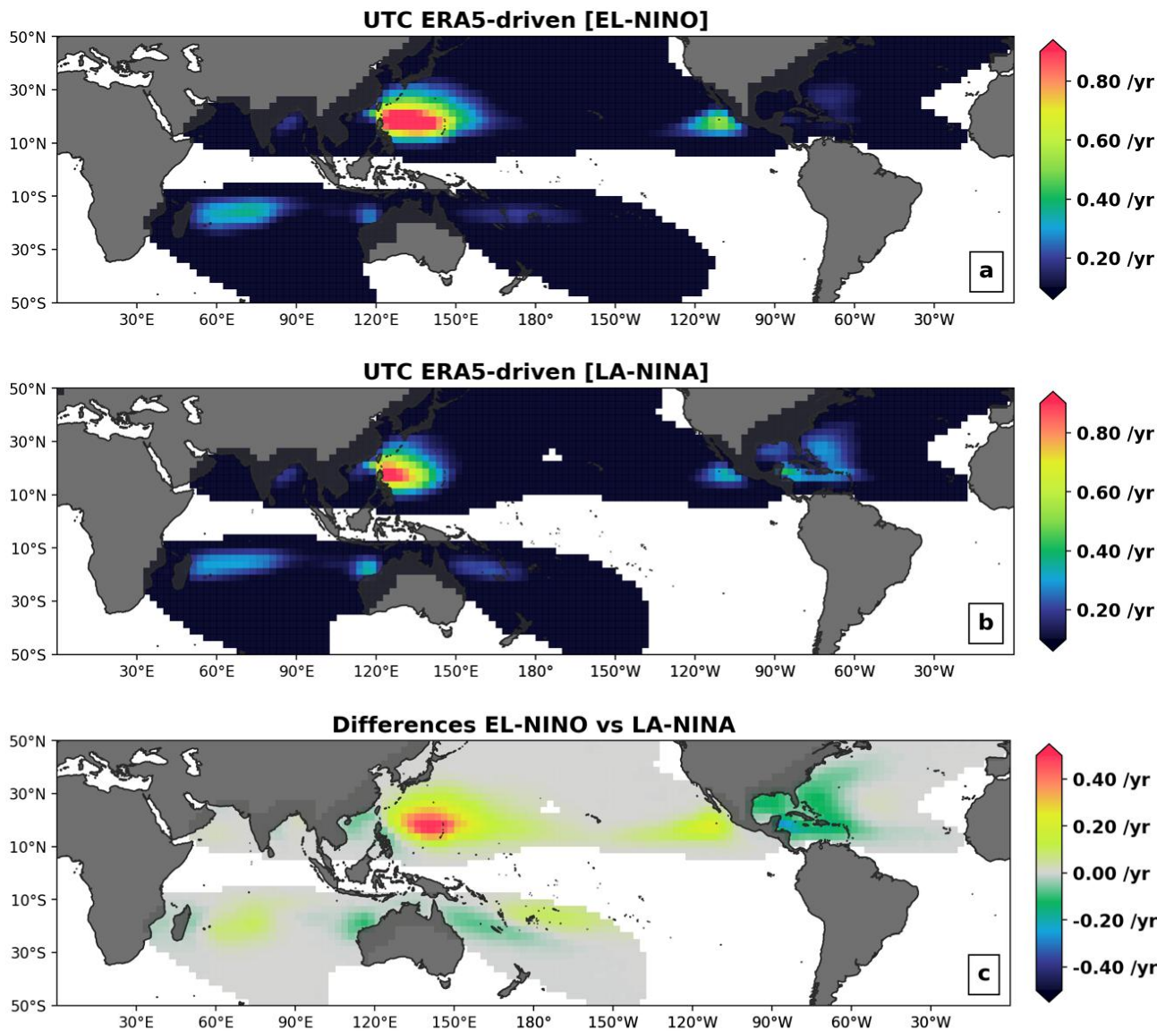
Fig. 12: Annual occurrence rates of category 3 tropical cyclones for 2 subsets of the 110'000-year UTC event set, characterizing the 10 strongest El Niño (a) and La Niña (b) seasons in the period 1980-2023; each hemisphere uses the ENSO conditions of the in-season months (ASO for the Northern hemisphere and DJF for the Southern hemisphere). The absolute differences between El Niño and La Niña rates of Cat3+ are shown in the last panel (c).
