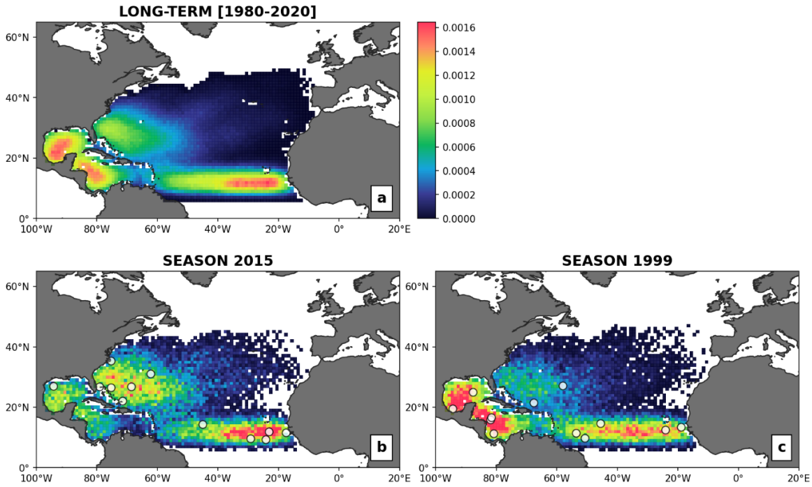
265 Fig. 6: Spatial genesis density maps at 1 deg resolution; a) shows smoothed out static version of historical occurrences while b) and c) illustrate the dynamic spatial probability of genesis accounting for SST and wind shear anomalies. The white dots show the historical cyclone genesis occurrence for the two years considered (2015 and 1999, see Fig. 7).
