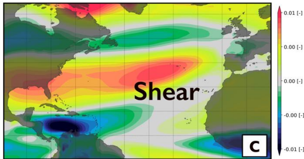
Figure A 2: Example of climate connector to conditions the ratio of North Atlantic storms seeded in the MDR region. a) relationship between the climate connector chosen (see Table A.2 – first row) and the rate in MDR. b, c and d) show the mode of variability associated with this climate connector.
