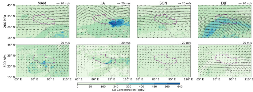
Fig. 8. Spatial distribution of CO concentration surrounding the Tibetan Plateau across different seasons, alongside mean horizontal wind vectors at 200 hPa and 500 hPa, represented by arrows. The study area is outlined in purple. The CO spatial distribution data is available from GEOS-CF, while the meteorological fields are derived from ERA5.
