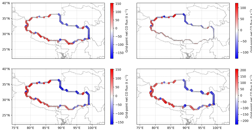
Fig. 5. The total CO flux for each grid across different seasons, based on data from May 2018 to April 2024, categorized into spring, summer, autumn, and winter. Red indicates external influx to the Tibetan Plateau, while blue represents internal efflux. Bubble size is proportional to flux magnitude, with positive and negative values
