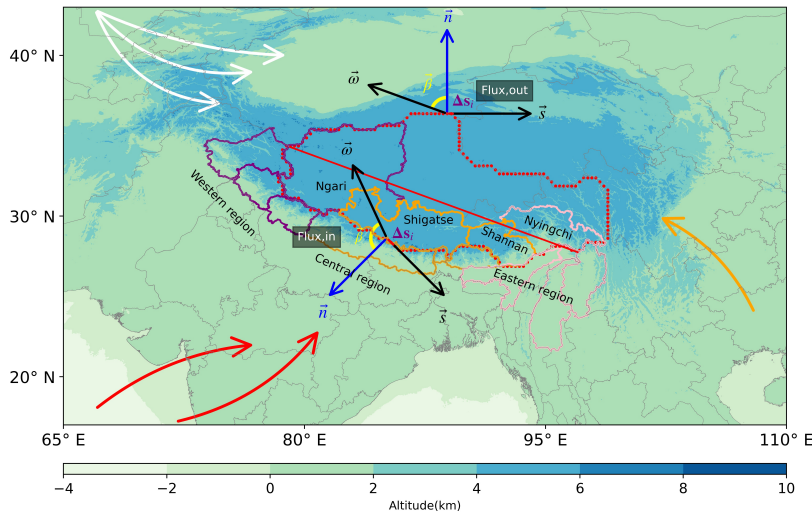
Fig. 2. Geographical description of the Tibetan Plateau and demonstration of the closed-loop integral method for CO flux calculation, with red points indicating the closed-loop. The black arrow \omega represents the wind field vector, s is the step vector for integration, and the blue arrow n denotes the boundary normal vector. \beta is the angle between the wind field vector \omega and the boundary normal vector n , while \Delta s represents the integration step length. White arrows indicate the westerly circulation over the plateau, red arrows represent the South Asian monsoon, and orange arrows indicate the East Asian monsoon. Surrounding areas are categorized into western (in purple), central (in orange), and eastern (in pink) regions. Within the Tibetan Plateau, highlighted areas include Ngari Prefecture, Shigatse City, Shannan City, and Nyingchi City. Elevation data is sourced from NOAA NCEI. The red bold line split the closed-loop of the Tibetan Plateau into southeastern and northeastern segments.
