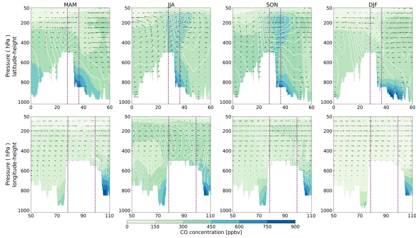
Fig. 9. The first row shows the latitudinal–altitude distribution of CO concentrations in different seasons averaged over the range 50°–110° E (positions correspond to different columns). The white contours at intervals of 18 \text{ m s}^{-1} represent the westerly (solid) and easterly (dashed) mean meridional winds; the white areas represent the terrain, and the arrows represent the wind vectors (vertical speed units are 10^{-4} \text{ hPa s}^{-1} , zonal wind units are \text{m s}^{-1} ); the study area is marked by the purple dashed line. The second row is calculated from the longitude–altitude angles, averaged over the range 27°–33°N. Here the white contours represent the southerly (solid) and northerly (dashed) mean zonal winds, and the horizontal component of the wind vector is the meridional wind ( \text{m s}^{-1} ). The meteorological fields are from ERA5.
