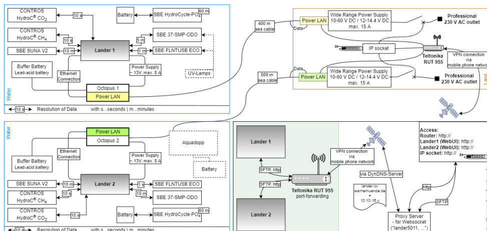
Figure A 1: The detailed overview of the measuring system, including the landers (left side), the power supply on land site (right top) and the remote access configuration (right bottom). Left: A dashed line represents equipment, that was used only for the actual lander. The captions at the arrows describes the resolution of measurements. Both landers were connected with a wired cable connection to ensure (right top) power supply and powerline communication. The hardware for this approach was bundled in the in-house developed “Octopus” device. The station on land enables remote power cycling and provides hardware for power supply and VPN connection. Right bottom: A schematic flowchart of the used VPN infrastructure, which enables control and adjustments to lander data and sensors schedules.
