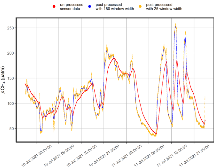
985 Figure C 1: The effects of the different post-processing methods on the sensor data (red). Strong smoothing (blue) resulted in a lower level of signal detail compared to weak smoothing (gold), but the impact of different window widths is predominantly low.
