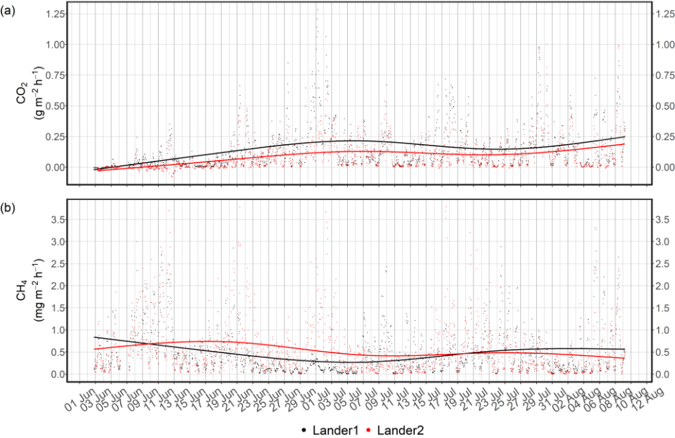
Figure E 2: Calculated GHG fluxes using the Wanninkhof, (2014) wind speed parameterization approach for \text{CO}_2 and \text{CH}_4 at both landers. A smoothing was used to highlight the trend and differences between the landers (description of smoothing in given in Appendix D).
