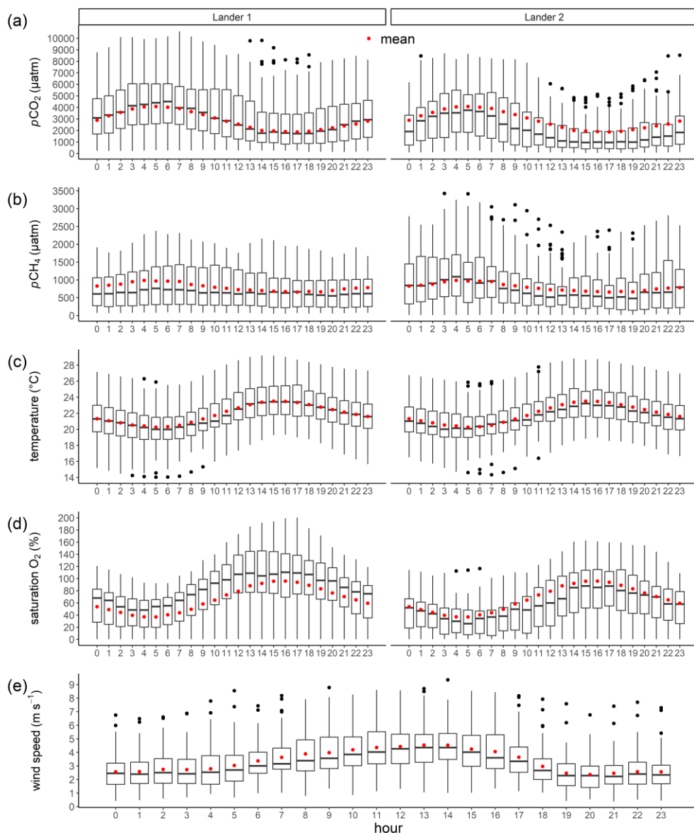
Figure 4: The distribution daily cyclicality of the mean values of p\text{CO}_2 , p\text{CH}_4 , temperature, \text{O}_2 , and wind speed derived from from-of-hourly one-hour-parts binning sections over 24 hours . The box plots show the median and the 25 / 75 % quantiles percentiles . The whiskers indicate the 5 / 95 % percentiles, and the red points denote the mean values.
