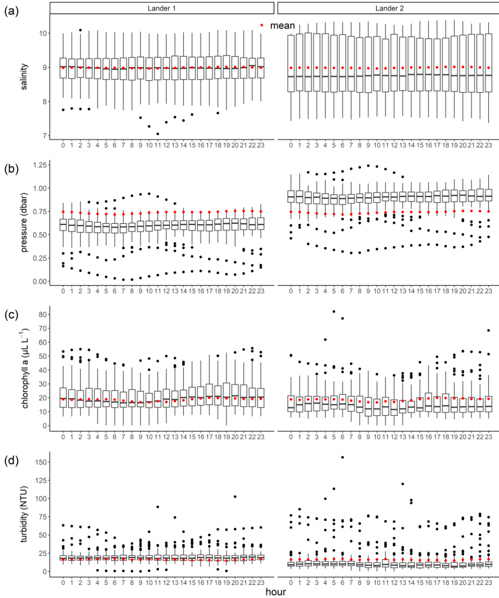
Figure E 3: The distribution-daily cyclicality of the mean values of salinity, pressure, chlorophyll a , and turbidity derived from hourly binning from one-hour parts over 24 hours . The box plots show the median and the 25 / 75 % quantilespercentiles . The whiskers indicate the 5 / 95 % percentiles, and the red points denote the mean values.
