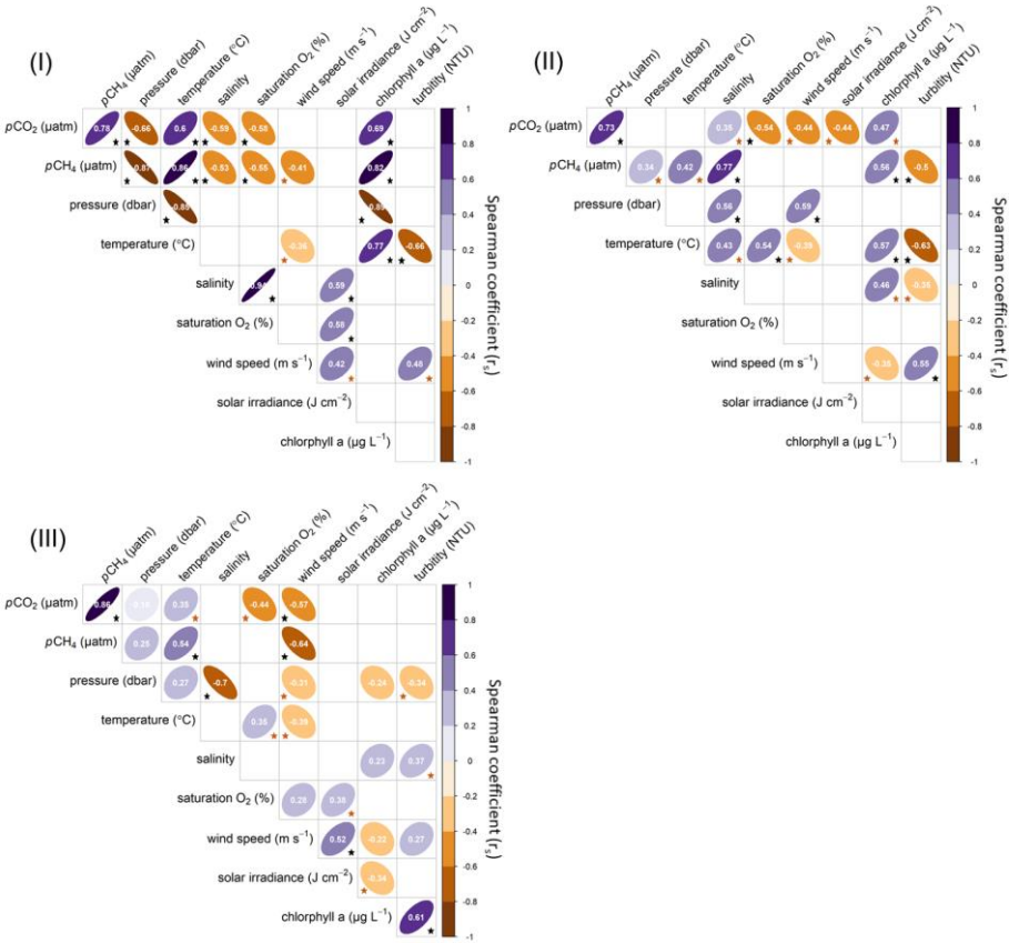
Figure E 4: Spearman correlation coefficients ( r_s ) between the measured variables of lander 1, wind speed, and solar irradiance limited to the three time periods (I) – (III). A correlation level of 0.001 was used to remove non-correlating relationships (empty fields). In addition, the Cohen convention (Cohen, 1988) was used to interpret the effect size. The black stars represent a large effect size and thus a strong correlation, while the brown stars represent a medium effect size. Wind speeds were retrieved from the station Putbus (WMO-ID 10093) and solar irradiance from Rostock-Warnemünde (WMO-ID 10170; both DWD).
