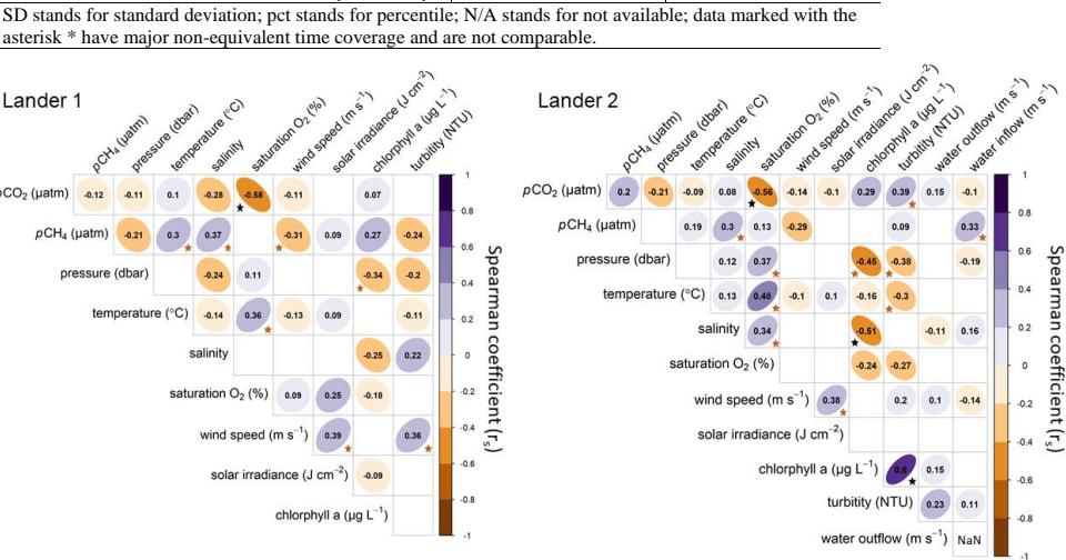
445 Figure 3: Spearman correlation coefficients ( r s ) between the measured variables, wind speed and solar irradiance of both landers. A correlation level of 0.001 was used to remove non-correlating relationships (empty fields). In addition, the Cohen convention (Cohen, 1988)
