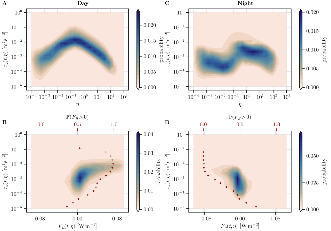
Figure 3. Probability densities of the amplitude of the vertical component of the Reynolds stress tensor \tau_w(t, \eta) against normalised frequency \eta (top row) and against the sensible heat flux F_H(t, \eta) (bottom row), estimated from 10 to 19 June 2022 via kernel densities from 8 h data during daytime (left column) and during night (right column). Red crosses show the empirical probability function that sensible heat is positive ( \mathbb{P}(F_H > 0) > 0.5 ) or negative ( \mathbb{P}(F_H > 0) < 0.5 ) (upper x-axis) vs. \tau_w .
