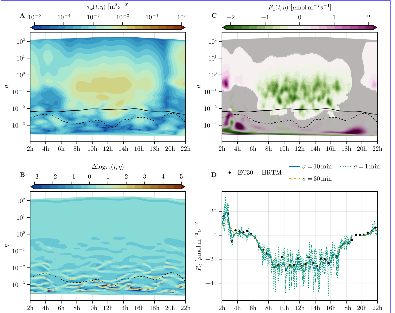
Figure 2. Turbulent transport identification and estimation of CO 2 flux on the 15 of June 2022. All time and frequency analyses are visualised in normalised frequencies \eta versus time over 24 h. A: time and frequency decomposition of the amplitude of the vertical component of the Reynold's stress tensor \tau_w . B: Laplacian of \log \tau_w in time and frequency space with an estimated time-varying spectral gap (dashed line) separating the turbulent transport at small scales from structures at larger scales. C: CO 2 flux in time and frequency space with a turbulence mask derived from analyses of A and B. A time varying 30 min spectral gap associated to the frequency separation of the standard eddy-covariance EC30 is also shown (solid line). D: High time-resolution CO 2 flux (HRTM) along CO 2 estimations with different averaging times against standard 30 min eddy-covariance (EC30).
