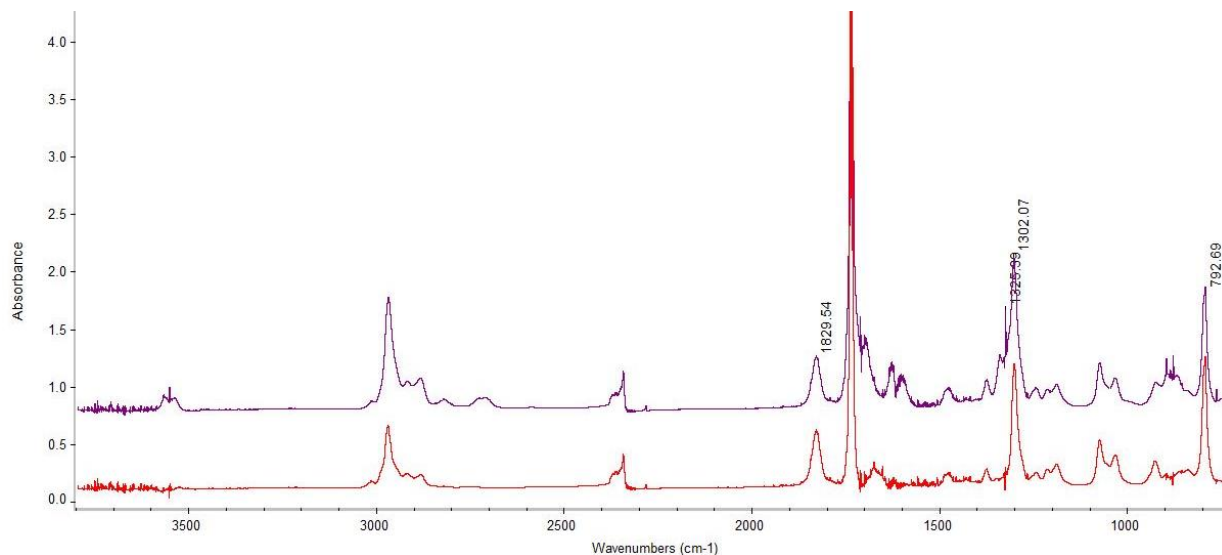
Figure 7. FTIR spectrum of the reaction of 33DMbutanal (at 21 min) with NO 3 radical (upper). Residual FTIR spectrum (assigned to peroxy-3,3-dimethylbutyryl nitrate) after elimination of N 2 O 5 , HNO 3 , 33DMbutanal and NO 2 (lower).
