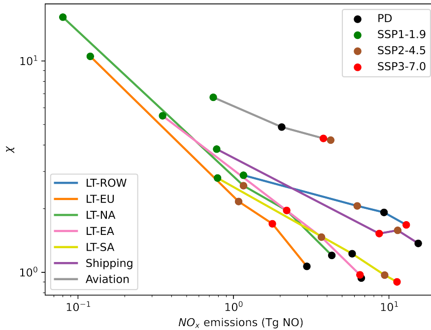
Figure 10. Dependency between \chi and the annual \text{NO}_x emissions (in \text{Tg}(\text{NO}) ). \chi is calculated as global mean over 5 years. Shown are the results of the 7 transport categories (land transport (indicated as LT-): ROW, EU, NA, SA and EA, aviation and shipping) for each simulation (colour coded).
