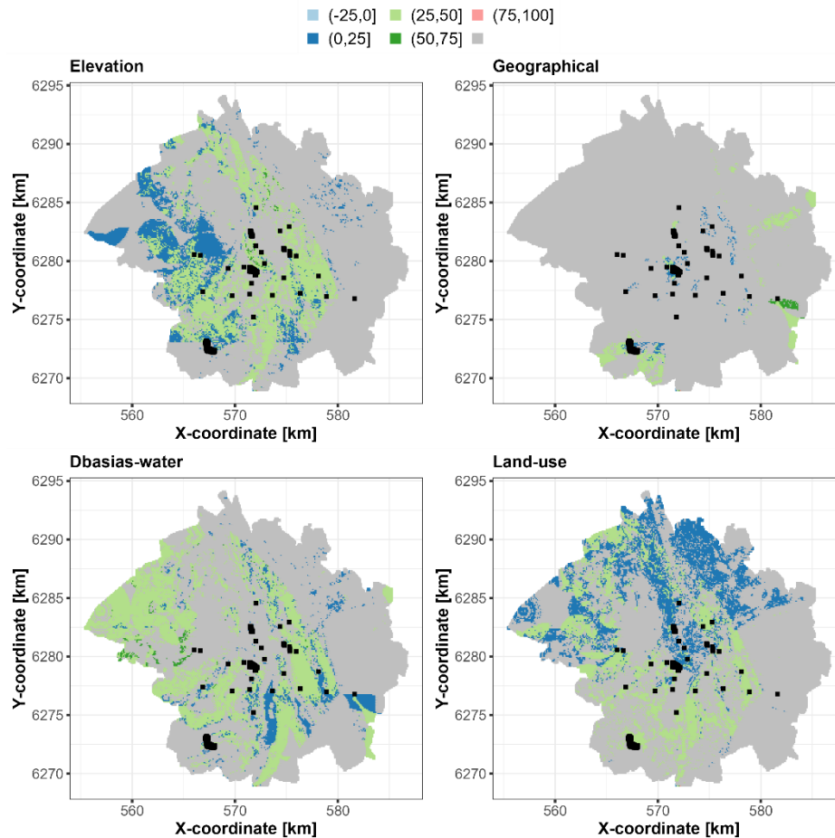
Figure 11: Locations where each corresponding group of covariates contributes significantly to the best estimate, with a scaled Shapley value exceeding that of the uncertainty by more than 25%. The colours indicate the scaled Shapley value for the best estimate. The areas in grey correspond to grid points where the condition is not met. The black squares indicate the locations of the soil samples used for RF training.
