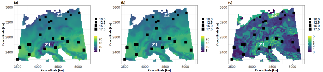
Figure 6: (a) Spatial distribution of the synthetic variable of interest modelled by Eq. 1; (b) Prediction best estimate using the conditional mean of the RF model. (c) Interquartile width IQW computed using the 25th and 75th quantiles of the qRF model. The 25 soil samples are indicated by squares whose sizes are proportional to the value of the synthetic variable of interest. The results are more specifically discussed in Sect. 4.1 for the zones indicated by Z_{1-2} .
