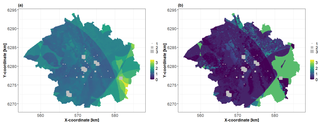
345 Figure 9: (a) Prediction best estimate of the hydrocarbon concentration ( \log_{10} scale) for the city of Toulouse using the conditional mean of the RF model. The soil samples are indicated by squares whose sizes are proportional to the \log_{10} of the hydrocarbon concentration. (b) Interquartile width IQW computed using the 25 th and 75 th quantiles of the qRF model (expressed on the same scale as the hydrocarbon concentration).
