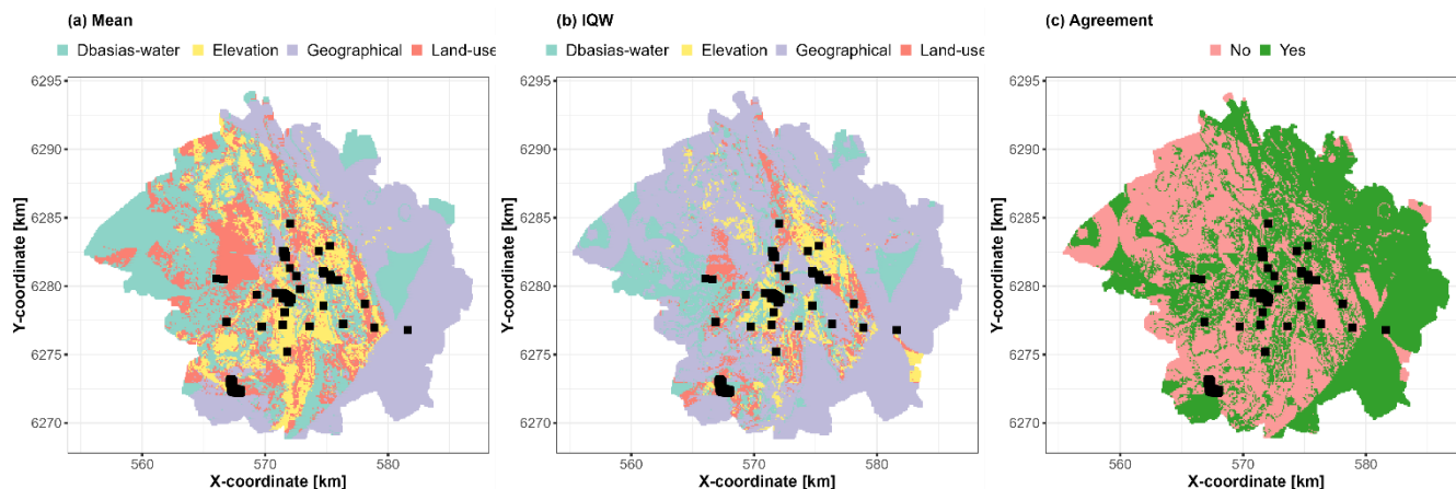
435 Figure 13: Spatial distributions of the most important group of covariates with respect to the scaled Shapley values for the prediction best estimate (mean, Panel a) and for the prediction uncertainty ( IQW , Panel b) in the city of Toulouse. Panel c shows the regions where the most important group of covariates for the mean agrees with that for IQW . The black squares indicate the locations of the soil samples used for RF training.
