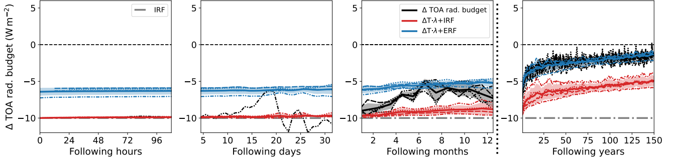
Figure 4. Same as Fig. 2, for simulated and calculated TOA radiative budget changes. Shown are TOA radiative budget change, based on the simulated surface temperature change, only considering IRF ( N_{\text{calc,IRF}} , red), the calculated TOA radiative budget change considering IRF + RA = ERF ( N_{\text{calc,ERF}} , blue) and the simulated TOA radiative budget change ( N_{\text{sim}} , black).
