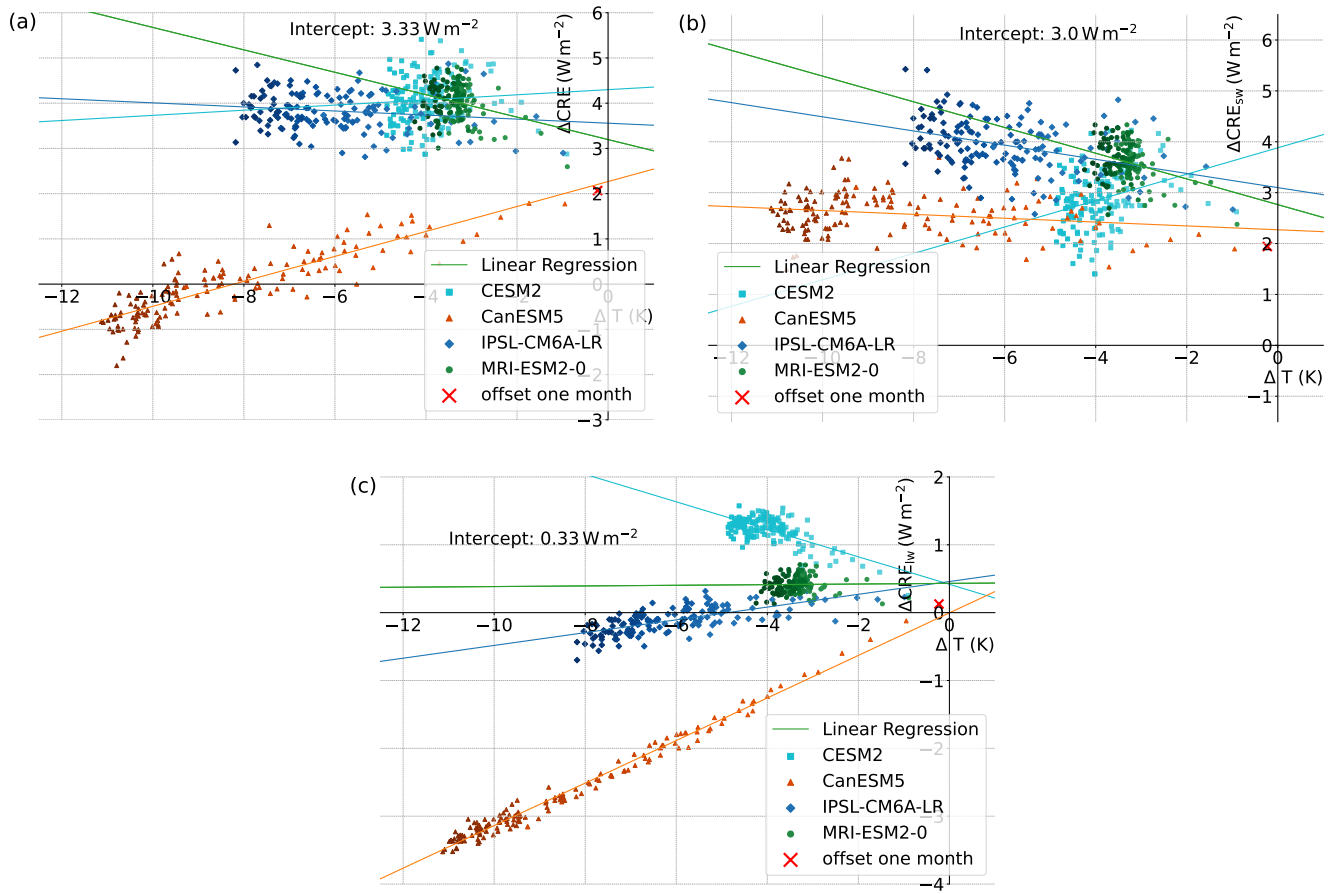
Figure A2. Same as Fig. A1 but for Linear regression plots for yearly global mean \Delta\text{CRE}_{\text{TOA}} (a) and its long- and shortwave components \Delta\text{CRE}_{\text{TOA,sw}} (b) and \Delta\text{CRE}_{\text{TOA,lw}} (c).
