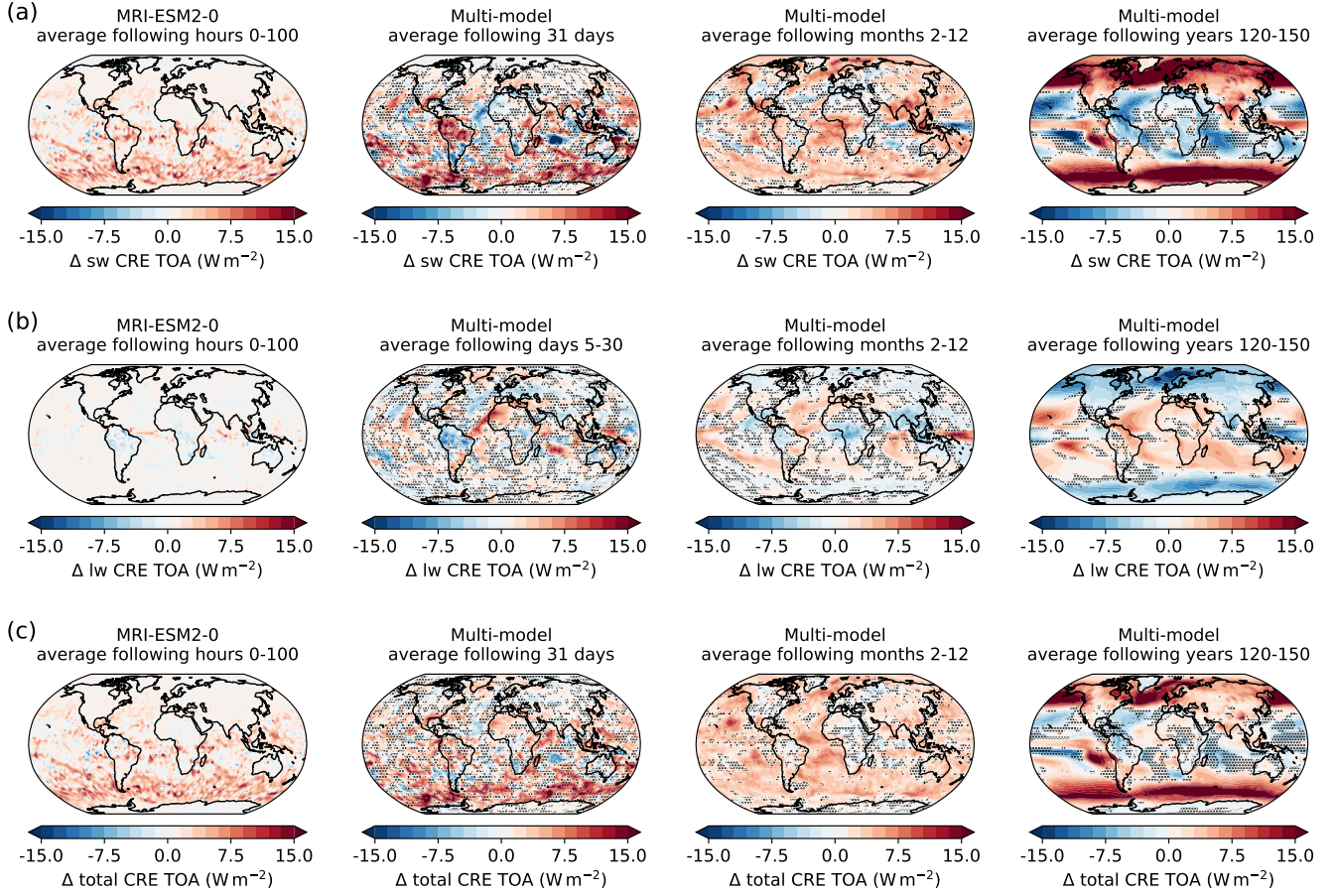
Figure B2. Same as Fig. B1 but for (a) shortwave and (b) longwave and (c) total TOA cloud radiative effect anomaly ( \Delta\text{CRE}_{\text{TOA},\text{sw}} , \Delta\text{CRE}_{\text{TOA},\text{lw}} and \Delta\text{CRE}_{\text{TOA}} ) in \text{W m}^{-2} .
