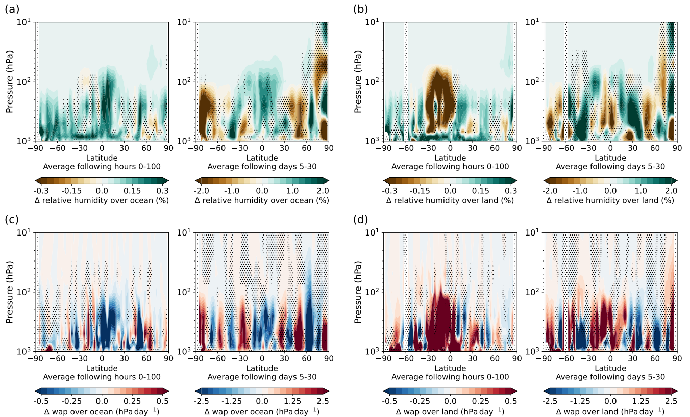
Figure 9. Zonal mean of relative humidity anomaly in % for the first 100 hours and days 5–30 (corresponds to the first two time scales of Fig. 8) averaged over ocean (a) and land (b) only and the same plots for vertical velocity (wap, positive downwards) anomaly in \text{hPa day}^{-1} averaged over ocean (c) and land (d).
