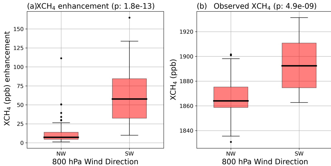
Figure 8. The distribution Distribution of the daily mean (a) simulated column tracers-tracer above the background and (b) observed XCH 4 per 800 hPa wind direction category and species . NW is for winds with an angle of 292.5 to 337.5 ° from north, while SW represents the angles between 202.5 and 247.5 °. There are 72 days with NW winds and 33 days with SW winds. The colored boxes indicate the range between the first and third quartile, while the thick solid line is the median. Outliers (values that are 1.5 times the interquartile range above (below) the third (first) quartile) are shown by black dots. The p-values of the corresponding non-parametric Mann-Whitney U tests are given in the title.
