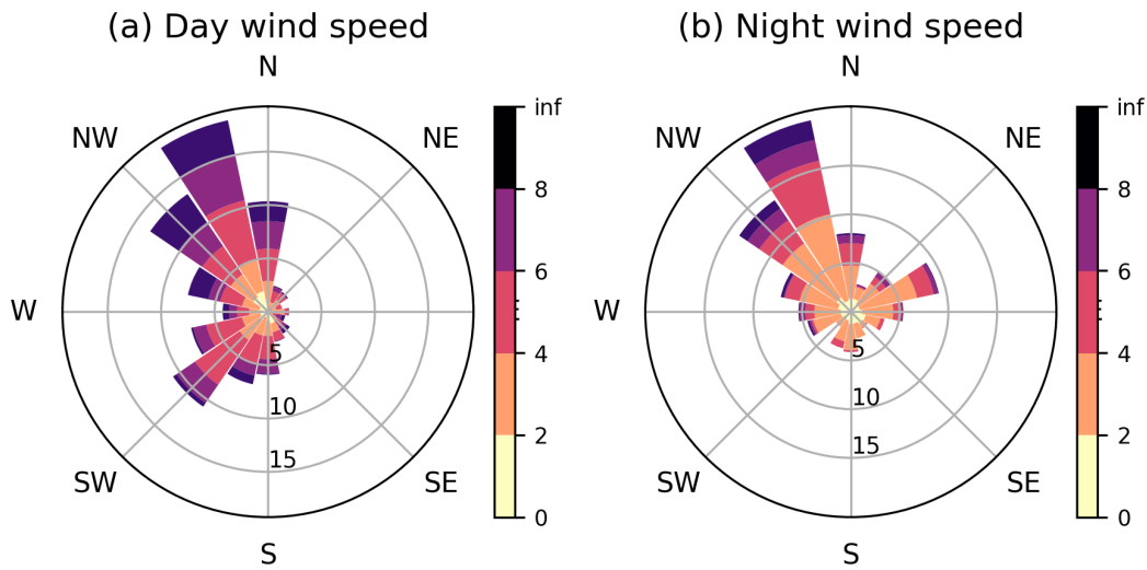
Figure C1. Wind rose from WRF-GHG simulations during the afternoon (13h - 18h LT) (a) and at night (3h - 8h LT) (b). The colors indicate the associated wind speed (in \text{m s}^{-1} ), while the lengths of the bars show the frequency of any wind direction binned by 22.5^\circ , given in percentage.
