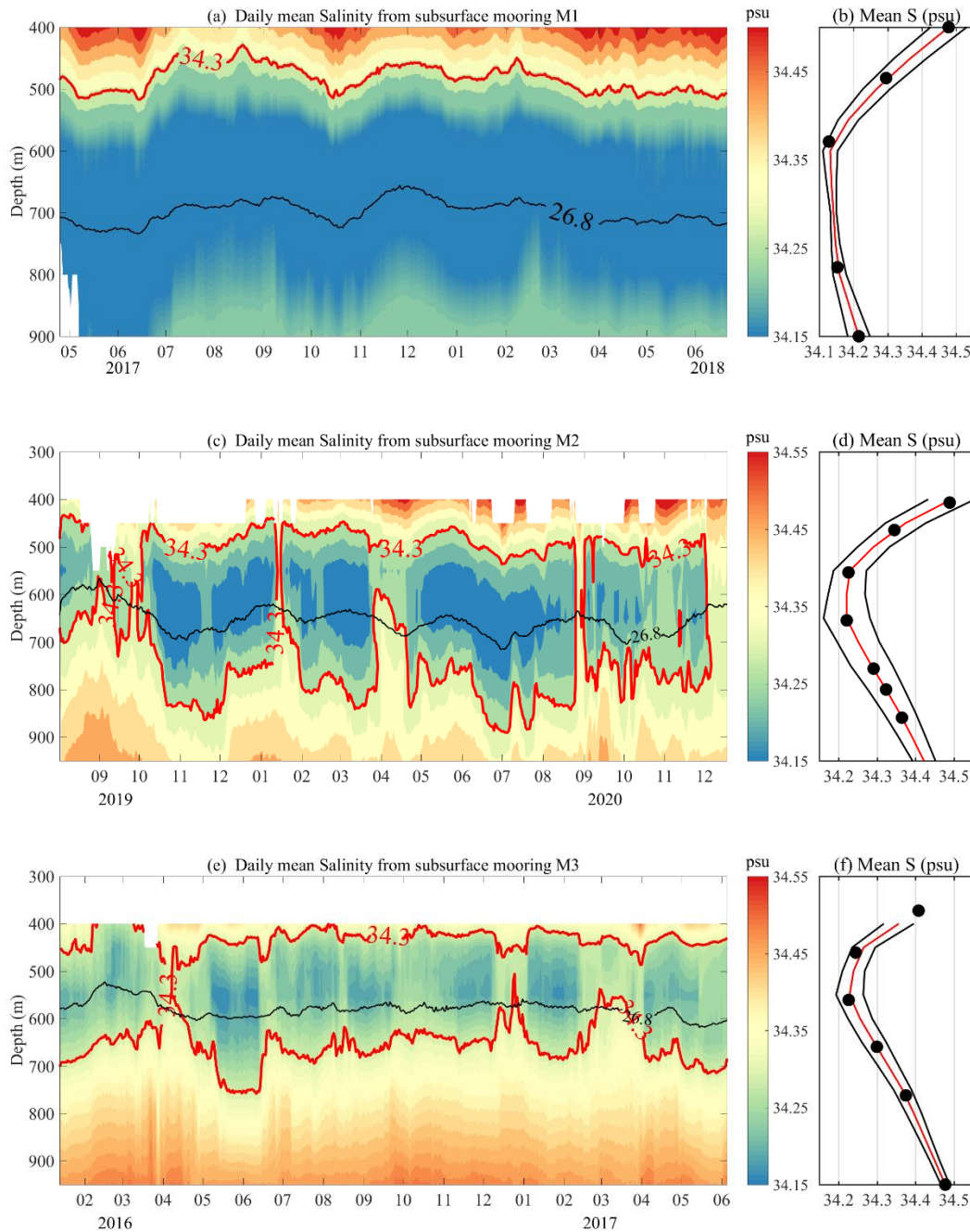
Figure 2. The observation of salinity from subsurface mooring. (a), (c) and (e) represent time series plots of salinity measured at different observation times for the three moorings, respectively. M1 is observed from April 2017-June 2018, M2 is observed from August 2019-
