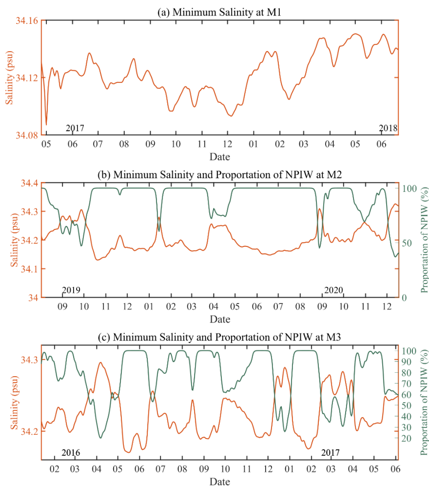
Figure 5. (a), (b) and (c) is the time series of minimum salinity (orange curve) and the proportion of NPIW (green curve). As at mooring M1, the water mass characteristics are all NPIW, it is 100 percent of the total, a straight line is not shown in the Figure.
