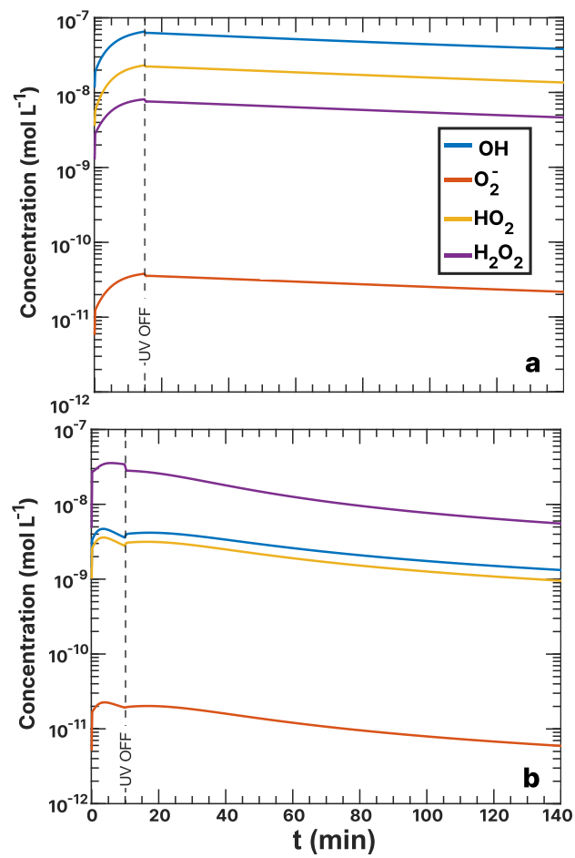
Figure F3. ROS concentrations during Fe III (Cit):CA = 1:10 ( a ) and Fe III (Cit):Cu II (HCit):CA = 1:0.2:1 ( b ) experiment simulation as a function of time. UV radiation was turned off at t = 15 min ( a ) and 10 min ( b ).
