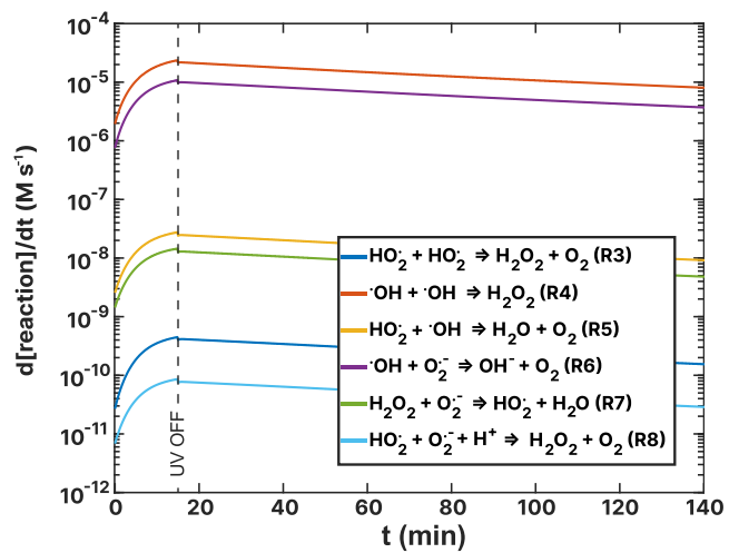
Figure F2. Turnover rates ( d/dt ) of the ROS reactions listed in Table 3 as a function of time, t , of the \text{Fe}^{\text{III}}(\text{Cit}) : \text{CA} = 1 : 10 experiment (a) and the \text{Fe}^{\text{III}}(\text{Cit}) : \text{Cu}^{\text{II}}(\text{HCit}) : \text{CA} = 1 : 0.2 : 1 experiment (b) simulations. UV radiation was turned off at t = 15 min.
