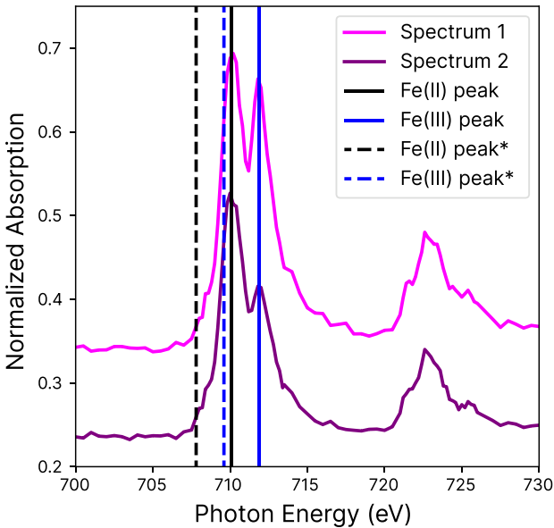
Figure A1. Iron arbsorption as a function of photon energies over the the L-edge with the iron(II) (black) and iron(III) (blue) absorption peaks (straight lines). The peaks were calibrated with measurements by Moffet et al. (2012) (stared) and they differed by 2.3 eV. Two independently measured spectra are shown.
