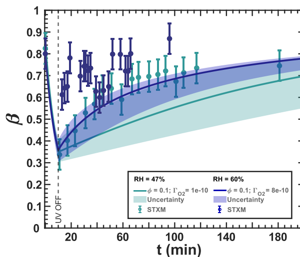
Figure 13. Iron(III) fraction, \beta , as a function of time, t , for irradiation at t = 0-10 min with a light intensity of (13.55 \pm 0.06) \text{ W m}^{-2} , RH = 60% (blue) and 47% (turquoise) with a mole ratio of \text{Fe}^{\text{III}}(\text{Cit}) : \text{Cu}^{\text{II}}(\text{HCit}) : \text{CA} = 1 : 0.02 : 1 (ten times less copper than in Figure 12). The circles with error bars represent the average of all particles mapped in one time step during the STXM experiments. Data uncertainty (error bars), model prediction and model uncertainties (straight lines and shading, respectively) are as defined in Figure 3. The iron(II) quantum yield, \phi=0.1 , was taken from the anoxic experiment shown in Figure 11, which resulted in a photolysis frequency of j = (8.1 \pm 1.0) \times 10^{-4} \text{ s}^{-1} ). Oxygen uptake coefficients, \Gamma_{\text{O}_2} , are indicated in the legend.
