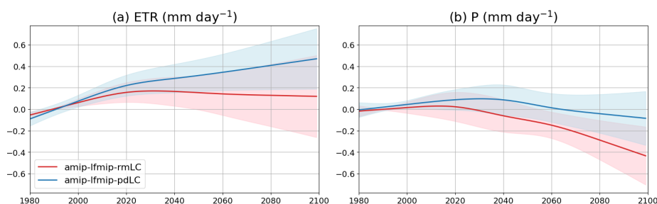
305 Figure 7: Anomalies of summer (a) evapotranspiration ( \text{mm day}^{-1} ) and (b) precipitation ( \text{mm day}^{-1} ), averaged over WCE for the period 1980-2100 using the 1980-2000 period as reference, for two experiments from LS3MIP where soil moisture is prescribed. The red line shows the multi-model mean of the simulations where the running mean of soil moisture from the historical + SSP5-8.5 scenario is prescribed (amip-lfmip-rmLC). The blue line shows the multi-model mean of the simulations where the present-day climatological soil moisture is prescribed through the simulation (amip-lfmip-pdLC, see Section 2). The shaded area represents the mean \pm one inter-model standard deviation. Seven models are used for this analysis (see Table 1). 310
