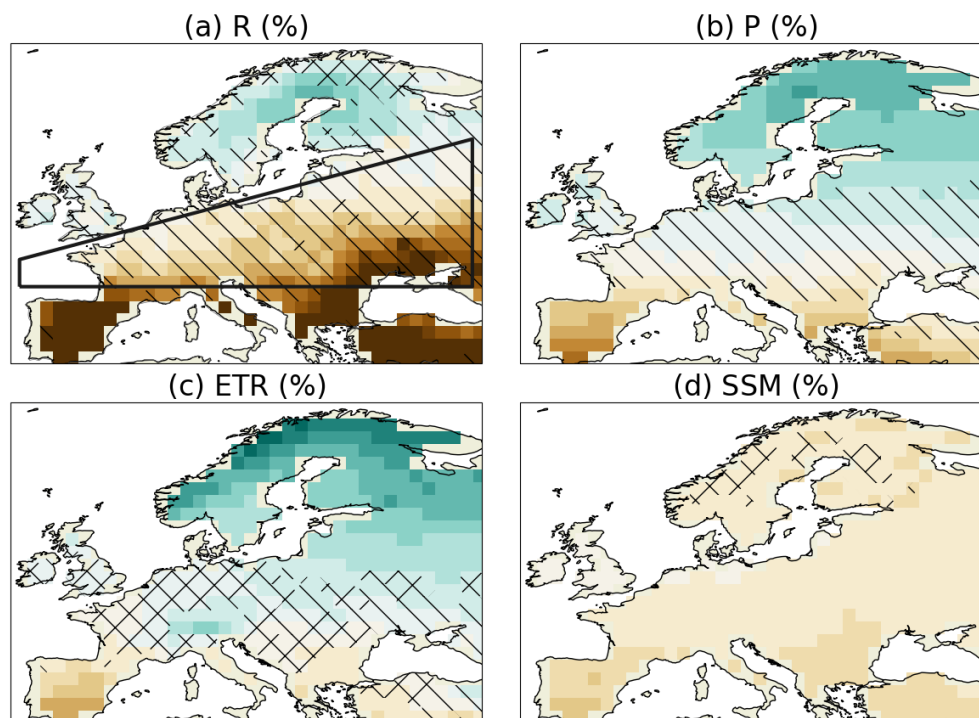
155 Figure 2: Multi-model ensemble mean of annual relative changes (%) between 1995-2014 and 2081-2100 under the SSP5-8.5 scenario 160 in (a) runoff, (b) precipitation, (c) evapotranspiration and (d) surface soil moisture. 36 CMIP6 models are used (see Table 1). On these maps, one member per model is used. The hatched area shows where less than 66% of the models project changes greater than the variability threshold. The crossed area shows where more than 66% of the models project changes greater than the variability threshold and less than 80% of the models agree on the sign of the changes. The variability threshold is defined as \gamma = \sqrt{2/20} * 1.645 * \delta_{1yr} where \delta_{1yr} is the interannual standard deviation calculated in a linearly detrended modern period (Gutiérrez et al., 2021; Zappa et al., 2021). The enclosed area in (a) is the western and central Europe (WCE) region, as defined in the Sixth Assessment Report (Iturbide et al., 2020).
