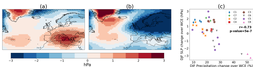
280 Figure 6: Sea level pressure changes in winter (DJF), between 1995-2014 and 2081-2100 under the SSP5-8.5 scenario, for (a) the multi-model ensemble mean of all models except models from C8 and TaiESM1 and (b) multi-model ensemble mean of C8 models and TaiESM1. The hatched area in (a) indicates where at least 80% of models agree on the sign of the change. (c) Scatterplot between winter changes in precipitation (%) averaged over WCE (x-axis) and winter changes in sea level pressure (hPa) averaged over WCE (y-axis) of all CMIP6 models. The Pearson correlation coefficient (“r”) and the corresponding p-value is given in the figure.
