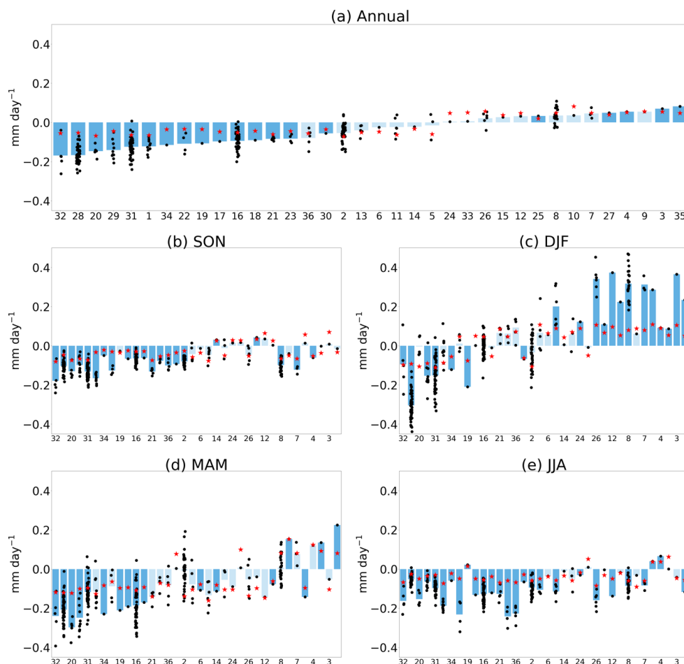
Figure 3: Changes ( \text{mm day}^{-1} ) in (a) annual and seasonal (b) autumn, (c) winter, (d) spring and (e) summer runoff over WCE, between 1995-2014 and 2081-2100 under the SSP5-8.5 scenario. Each bar corresponds to the multi-member mean of the model whose identification number (see Table 1) is given on the x-axis. The models are ordered by ascending value of annual runoff changes. The dots correspond to the changes of each member. The red stars correspond to the variability threshold, defined as \gamma = \sqrt{2/20} * 1.645 * \delta_{1yr} where \delta_{1yr} is the interannual standard deviation calculated in a linearly detrended modern period (Gutiérrez et al., 2021; Zappa et al., 2021). The variability threshold is multiplied by -1 when the multi-member mean is negative. Dark blue indicates that the changes in more than 66% of members exceed the multi-member mean of the variability threshold.
