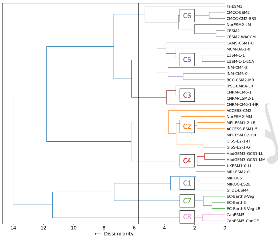
Figure 1. Hierarchical clustering tree of the 36 CMIP6 models analyzed in this study based on their seasonal changes in precipitation, evapotranspiration and runoff, averaged over WCE between the periods 2081–2100 and 1995–2014. The clusters are labeled from C1 to C8. Models within the same cluster share the same color.
