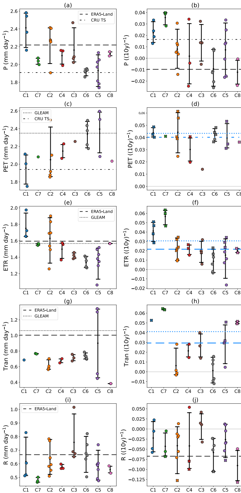
Figure 5: Annual climatological mean ( \text{mm d}^{-1} ) over 1985-2014 of (a) precipitation, (c) potential evapotranspiration, (e) evapotranspiration, (g) transpiration and (i) runoff. 10 years trends over 1985-2014 (relative to 1995-2014, (10\text{y})^{-1} ) of (b) precipitation, (d) potential evapotranspiration, (f) evapotranspiration, (h) transpiration and (j) runoff. The horizontal lines correspond to reference datasets. Blue lines indicate that the trend is significant ( p\text{-value} < 0.01 ). The models are grouped based on the hierarchical clustering. The clusters are defined in Fig. 1. The distribution is displayed with error bars indicating the 5-95% confidence interval. The colored dots and cross correspond to individual models with a single member (the first). The crosses indicate that the trend of the model is significant ( p\text{-value} < 0.01 ).
