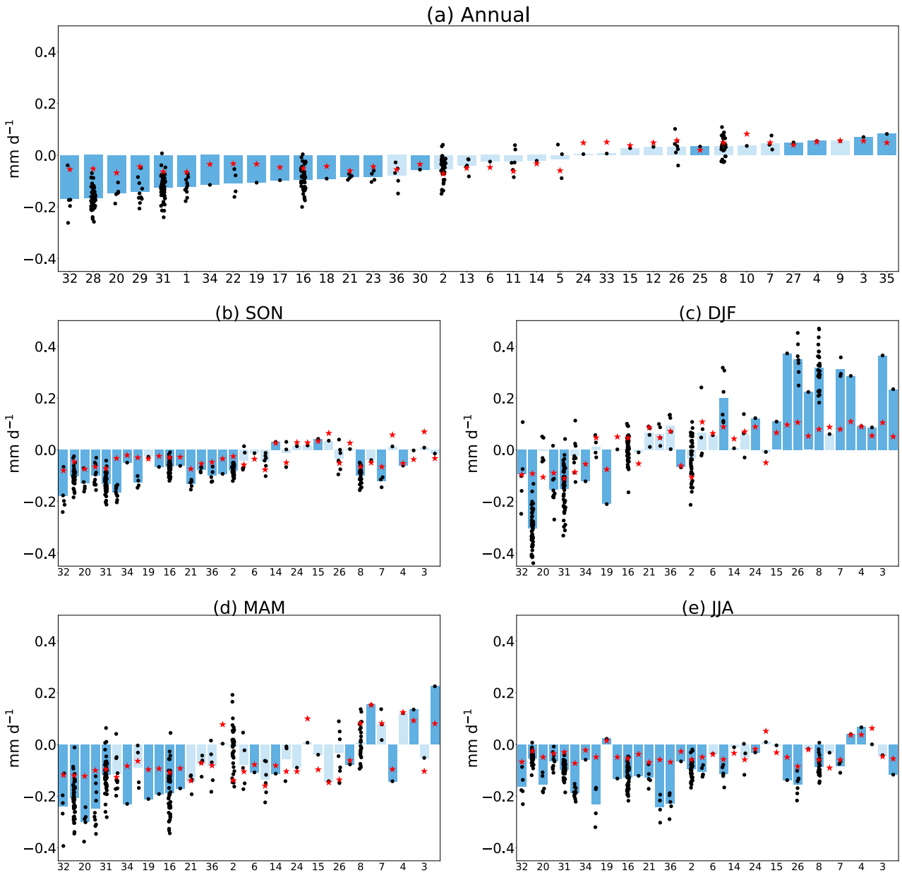
Figure 3: Changes (mm d -1 ) in (a) annual and seasonal (b) autumn, (c) winter, (d) spring and (e) summer) runoff over WCE, between 1995-2014 and 2081-2100 under the SSP5-8.5 scenario. Each bar corresponds to the multi-member mean of the model whose identification number (see Table 1) is given on the x-axis. The models are ordered by ascending value of annual runoff changes. The dots correspond to the changes of each member. The red stars correspond to the variability threshold (see the Data and Methods section) or to the variability threshold multiplied by -1 when the multi-member mean is negative. Dark blue indicates that the changes in more than 66% of members exceed the multi-member mean of the variability threshold.
