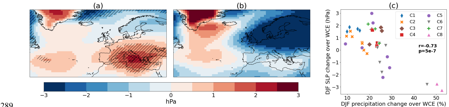
290 Figure 6: Sea level pressure changes in winter (DJF), between 2081-2100 and 1995-2014 under the SSP5-8.5 scenario, for (a) the 291 multi-model ensemble mean of all models except models from C8 and TaiESM1 and (b) multi-model ensemble mean of C8 models 292 and TaiESM1. The hatched area in (a) indicates where at least 80% of models agree on the sign of the change. (c) Scatterplot between 293 winter changes in precipitation (%) averaged over WCE (x-axis) and winter changes in sea level pressure (hPa) averaged over WCE 294 (y-axis) of all CMIP6 models. The Pearson correlation coefficient and the corresponding p-value are given in the sub-figure.
