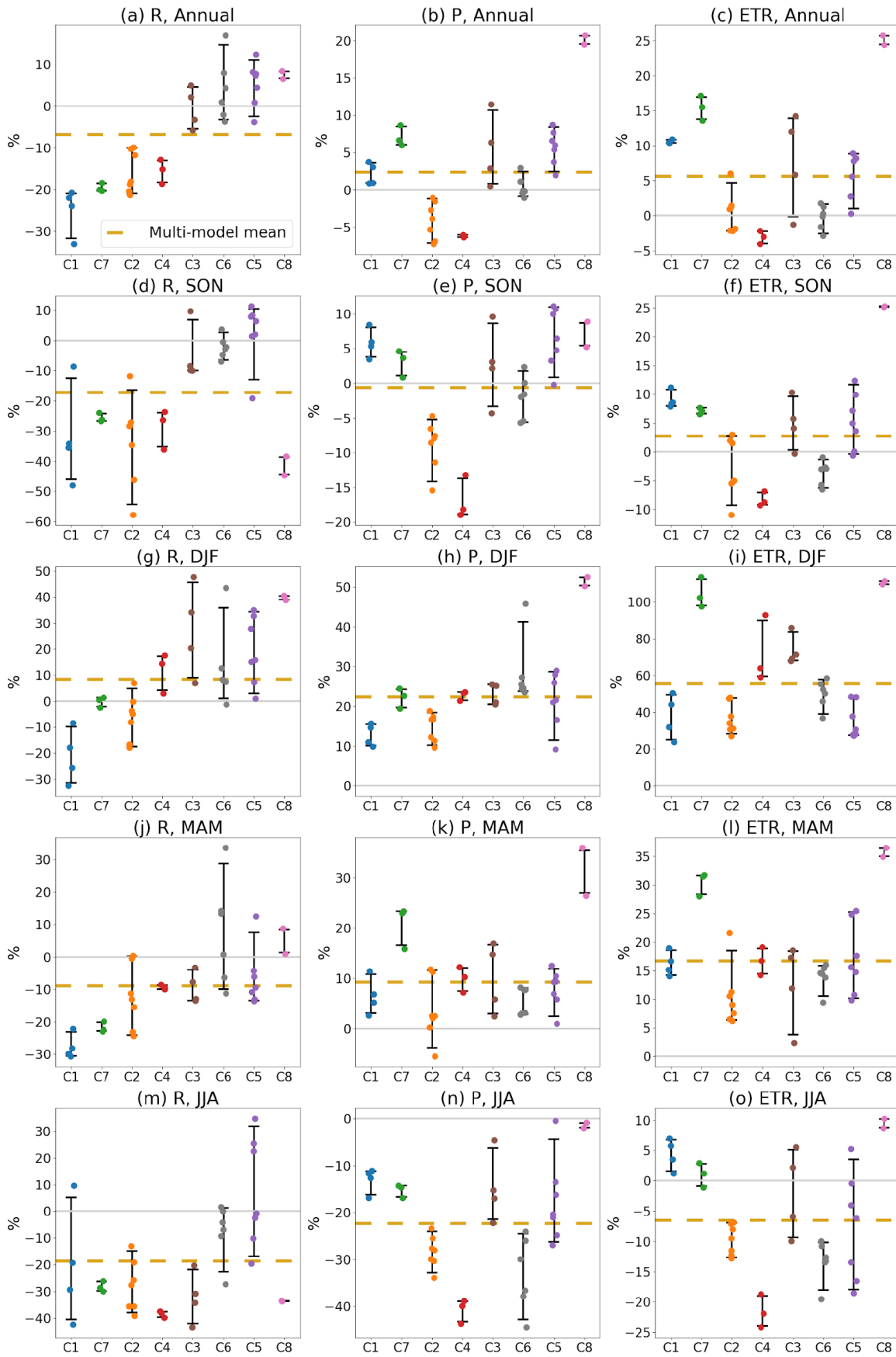
Figure 4: Relative changes (%) between 2081-2100 and 1995-2014 under the SSP5-8.5 scenario, in (a, d, g, j, m) runoff, (b, e, h, k, n) precipitation, and (c, f, i, l, o) evapotranspiration for the eight clusters identified through hierarchical clustering (see Section 2), for annual (a, b, c), autumn (d, e, f), winter (g, h, i), spring (j, k, l) and summer (m, n, o) changes. The clusters are arranged in ascending order based on their mean annual changes in runoff. The gold dashed line corresponds to the multi-model mean. The 5-
