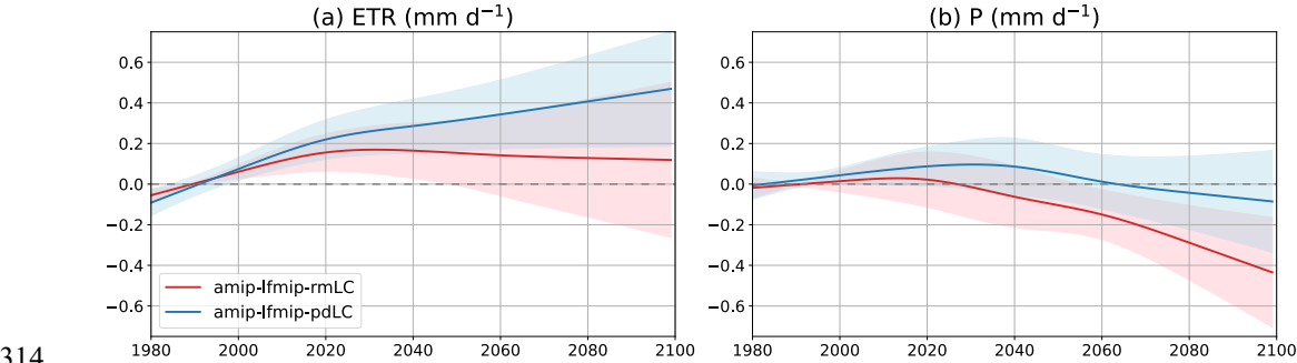
Figure 7: Anomalies of summer (a) evapotranspiration ( \text{mm d}^{-1} ) and (b) precipitation ( \text{mm d}^{-1} ), averaged over WCE for the period 1980-2100 using the 1980-2000 period as reference, for two experiments from LS3MIP where soil moisture is prescribed. The red line shows the multi-model mean of the simulations where the running mean of soil moisture from the historical + SSP5-8.5 scenario is prescribed (amip-lfmip-rmLC). The blue line shows the multi-model mean of the simulations where the present-day climatological soil moisture is prescribed through the simulation (amip-lfmip-pdLC, see Section 2). The shaded area represents the mean \pm one inter-model standard deviation. Seven models are used for this analysis (see Table 1).
