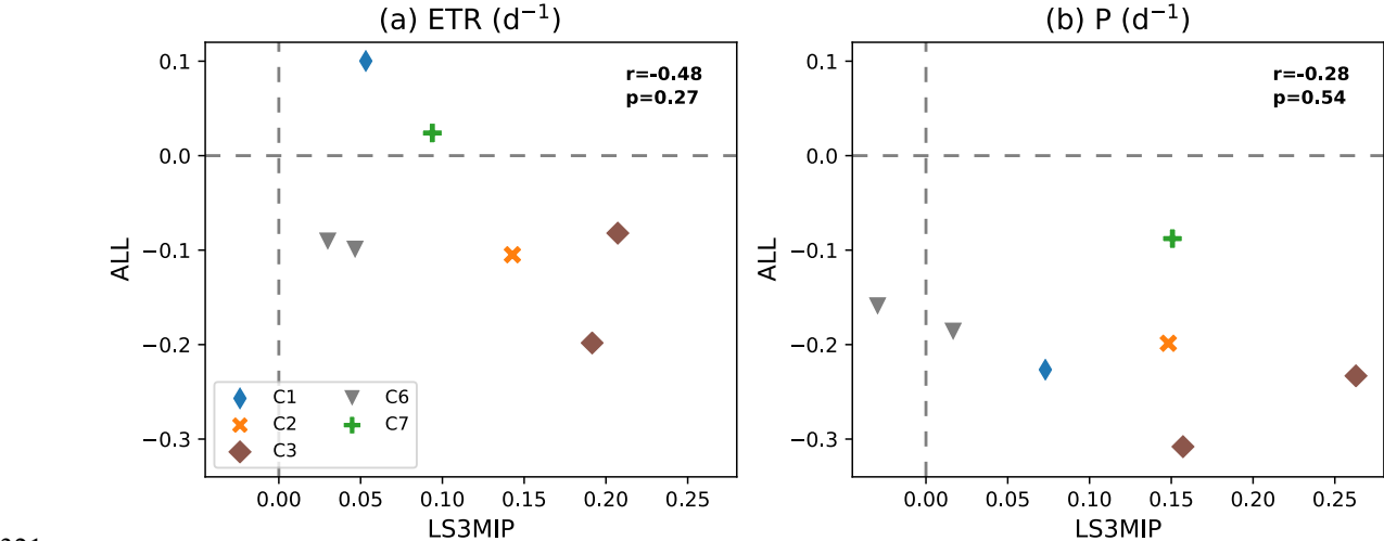
Figure 8: (y-axis) Absolute changes in summer (a) evapotranspiration and (b) precipitation over WCE between 2081-2100 and 1995-2014 for the SSP5-8.5 scenario and historical simulations standardized by the changes in soil moisture in each model ( \text{d}^{-1} ) versus (x-axis) difference between changes in amip-lfmip-rmLC (evolving soil moisture) and amip-lfmip-pdLC (constant soil moisture), standardized by the changes in soil moisture in the amip-lfmip-rmLC simulation in each model ( \text{d}^{-1} ). The Pearson correlation coefficient and corresponding p-value are given in the sub-figures. The seven models for which LS3MIP simulations are available are shown Table 1.
