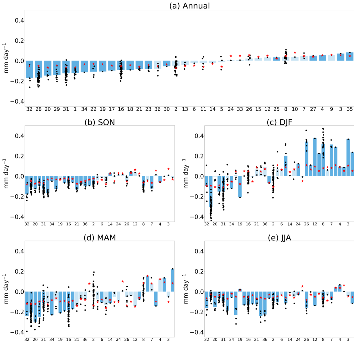
185 Figure 3: Changes ( \text{mm day}^{-1} ) in (a) annual and seasonal ((b) autumn, (c) winter, (d) spring and (e) summer) runoff over WCE, between 1995-2014 and 2081-2100 under the SSP5-8.5 scenario. Each bar corresponds to the multi-member mean of the model whose identification number (see Table 1) is given on the x-axis. The models are ordered by ascending value of annual runoff changes. The dots correspond to the changes of each member. The red stars correspond to the variability threshold (see the Data and Methods section) or to the variability threshold multiplied by -1 when the multi-member mean is negative. Dark blue indicates that the 190 changes in more than 66% of members exceed the multi-member mean of the variability threshold.
