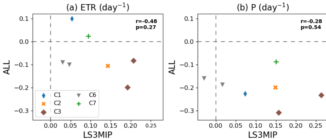
Figure 8: (y-axis) Absolute changes in summer (a) evapotranspiration and (b) precipitation over WCE between 1995-2014 and 2081-2100 for the SSP5-8.5 scenario and historical simulations standardized by the changes in soil moisture in each model ( \text{day}^{-1} ) versus (x-axis) difference between changes in amip-lfmip-rmLC (evolving soil moisture) and amip-lfmip-pdLC (constant soil moisture), standardized by the changes in soil moisture in the amip-lfmip-rmLC simulation in each model ( \text{day}^{-1} ). The Pearson correlation coefficient and corresponding p-value are given in the sub-figures. The seven models for which LS3MIP simulations are available are shown Table 1.
