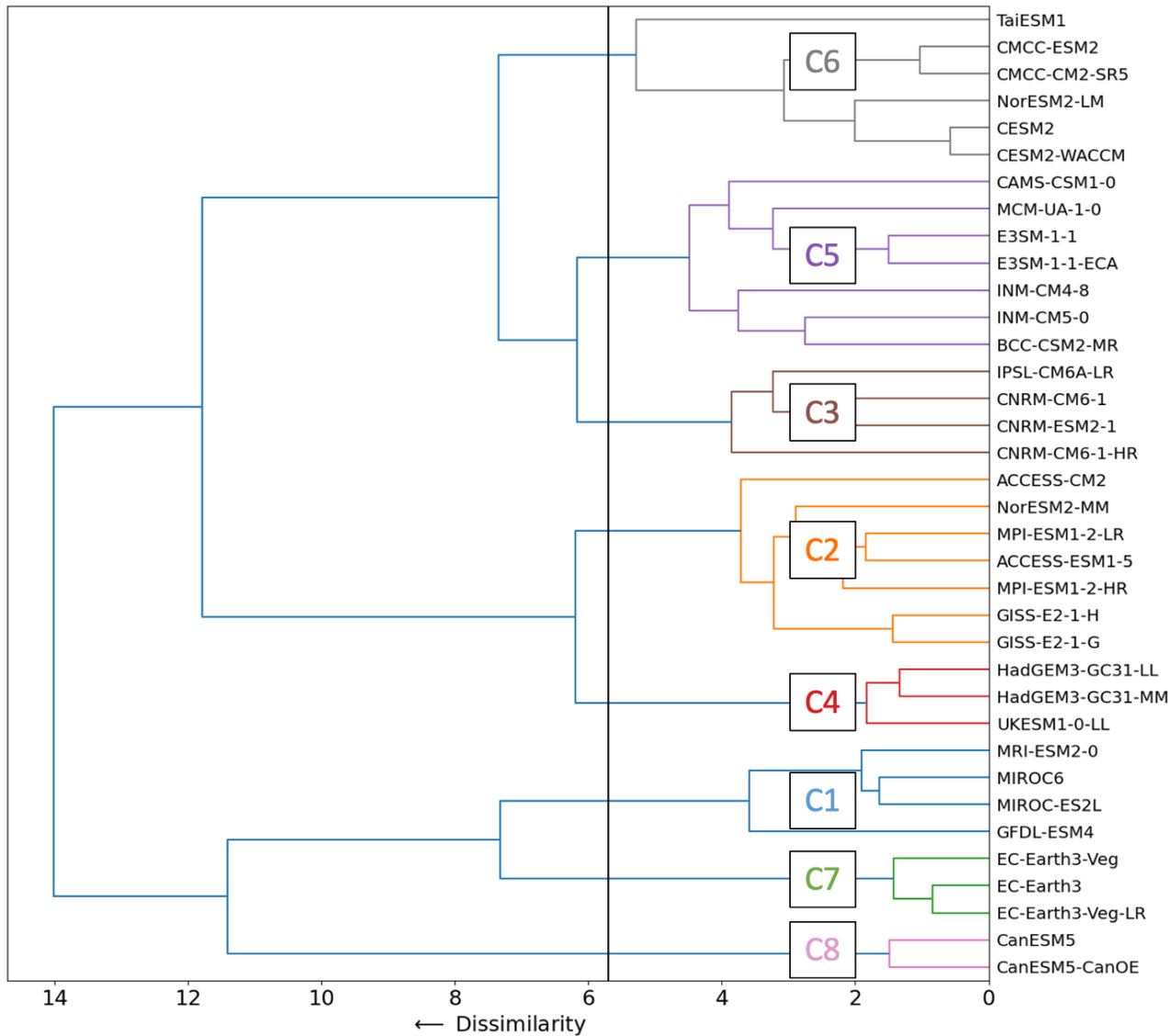
145 Figure 1: Hierarchical clustering tree of the 36 CMIP6 models analyzed in this study based on their seasonal changes in precipitation, evapotranspiration and runoff, averaged over WCE between the periods 2081-2100 and 1995-2014. The clusters are labeled from C1 to C8. Models within the same cluster share the same color.
