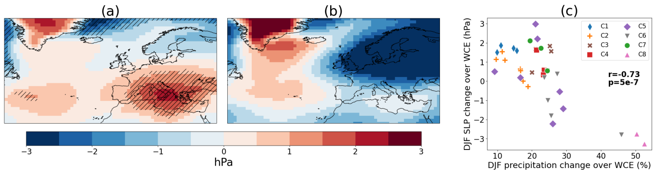
290 Figure 6: Sea level pressure changes in winter (DJF), between 1995-2014 and 2081-2100 under the SSP5-8.5 scenario, for (a) the multi-model ensemble mean of all models except models from C8 and TaiESM1 and (b) multi-model ensemble mean of C8 models and TaiESM1. The hatched area in (a) indicates where at least 80% of models agree on the sign of the change. (c) Scatterplot between winter changes in precipitation (%) averaged over WCE (x-axis) and winter changes in sea level pressure (hPa) averaged over WCE (y-axis) of all CMIP6 models. The Pearson correlation coefficient and the corresponding p-value are given in the sub-figure. 295
