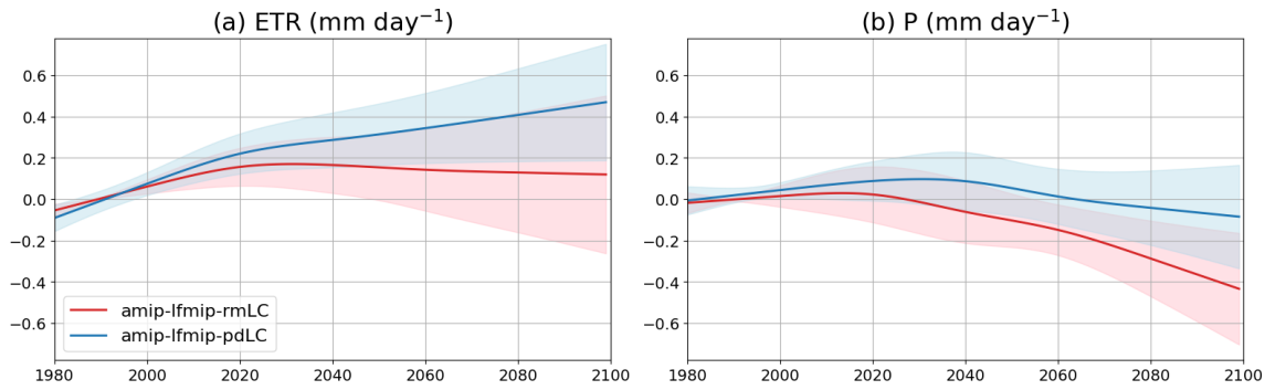
Figure 7: Anomalies of summer (a) evapotranspiration ( \text{mm day}^{-1} ) and (b) precipitation ( \text{mm day}^{-1} ), averaged over WCE for the period 1980-2100 using the 1980-2000 period as reference, for two experiments from LS3MIP where soil moisture is prescribed. The red line shows the multi-model mean of the simulations where the running mean of soil moisture from the historical + SSP5-8.5 scenario is prescribed (amip-lfmip-rmLC). The blue line shows the multi-model mean of the simulations where the present-day climatological soil moisture is prescribed through the simulation (amip-lfmip-pdLC, see Section 2). The shaded area represents the mean \pm one inter-model standard deviation. Seven models are used for this analysis (see Table 1).
