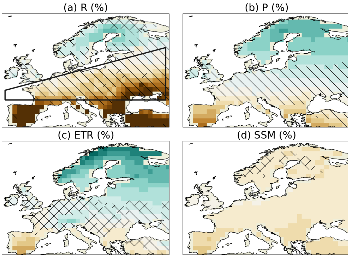
Figure 2: Multi-model ensemble mean of annual relative changes (%) between 1995-2014 and 2081-2100 under the SSP5-8.5 scenario in (a) runoff, (b) precipitation, (c) evapotranspiration and (d) surface soil moisture. 36 CMIP6 models are used (see Table 1). On these maps, one member (the first) per model is used. The hatched area shows where less than 66% of the models project changes greater than the variability threshold (see Data and Methods section). The crossed area shows where more than 66% of the models project changes greater than the variability threshold and less than 80% of the models agree on the sign of the changes. The variability threshold is defined as \gamma = \sqrt{2/20} * 1.645 * \delta_{1yr} where \delta_{1yr} is the interannual standard deviation calculated in a linearly detrended modern period (Gutiérrez et al., 2021; Zappa et al., 2021). The enclosed area in (a) is the western and central Europe (WCE) region (see Data section), as defined in the Sixth Assessment Report (Iturbide et al., 2020).
