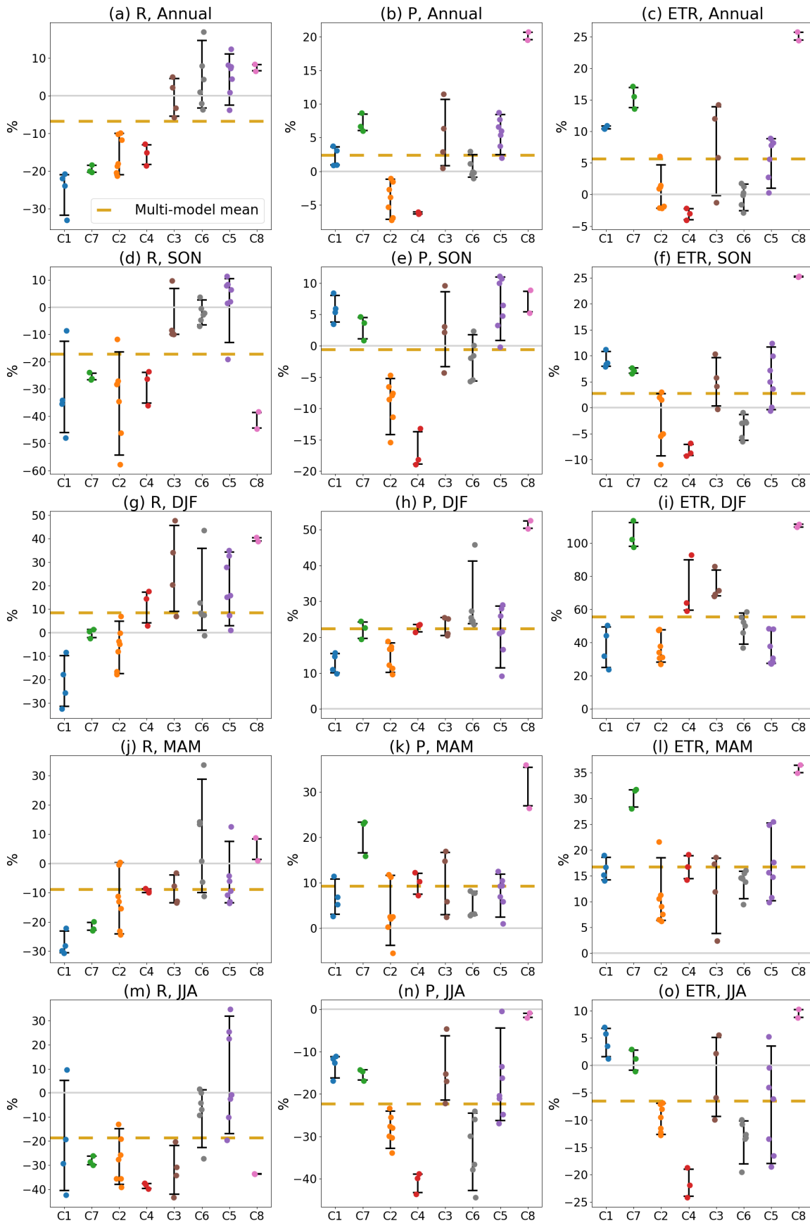
235 Figure 4: Relative changes (%) between 1995-2014 and 2081-2100 under the SSP5-8.5 scenario, in (a, d, g, j, m) runoff, (b, e, h, k, n) precipitation, and (c, f, i, l, o) evapotranspiration for the eight clusters identified through hierarchical clustering (see Section 2), for annual (a, b, c), autumn (d, e, f), winter (g, h, i), spring (j, k, l) and summer (m, n, o) changes. The clusters are arranged in ascending order based on their mean annual changes in runoff. The gold dashed line corresponds to the multi-model mean. The 5-95% confidence interval is shown with error bars for each cluster, and the results of individual models are shown with dots whose color corresponds to the cluster. 240
