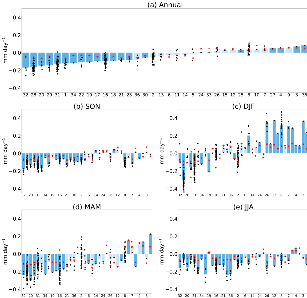
Figure 3: Changes (mm day -1 ) in (a) annual and seasonal ((b) autumn, (c) winter, (d) spring and (e) summer) runoff over WCE, between 1995-2014 and 2081-2100 under the SSP5-8.5 scenario. Each bar corresponds to the multi-member mean of the model whose identification number (see Table 1) is given on the x-axis. The models are ordered by ascending value of annual runoff changes. The dots correspond to the changes of each member. The red stars correspond to the variability threshold (see the Data and Methods section), defined as \gamma = \sqrt{2/20} * 1.645 * \delta_{1995-2014} where \delta_{1995-2014} is the interannual standard deviation calculated in a linearly detrended modern period (Gutiérrez et al., 2021; Zappa et al., 2021). The or to the variability threshold is multiplied by -1 when the multi-member mean is negative. Dark blue indicates that the changes in more than 66% of members exceed the multi-member mean of the variability threshold.
