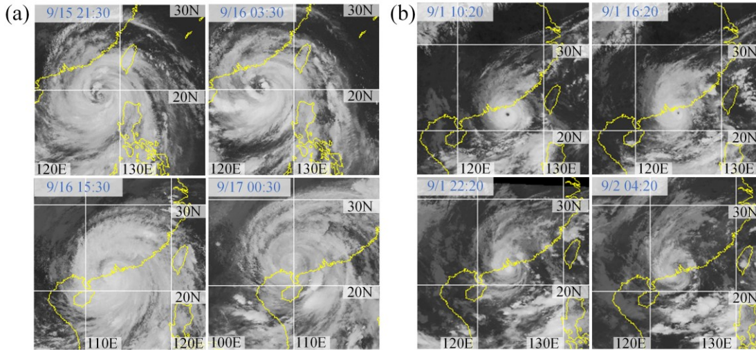
Figure 3: Infrared satellite snapshots of Mangkhut (a) and Saola (b) at 4 selected moments during landfall. Each photo spans an area of 20°×20°, or about 2,200×2,200 km (from CIMSS 2018)
