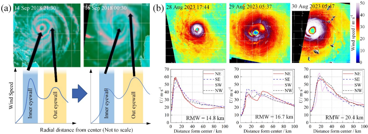
275 Figure 8: ER cycle for Mangkhut (a) and Saola (from https://www.weather.gov.hk/informtc/ Mangkhut18/windstructure.htm ) (b). Cloud image represents radial wind profiles obtained through the conversion of cross-polarized normalized radar cross section backscatter (from https://www.star.nesdis.noaa.gov/socd/ mecb/sar )
