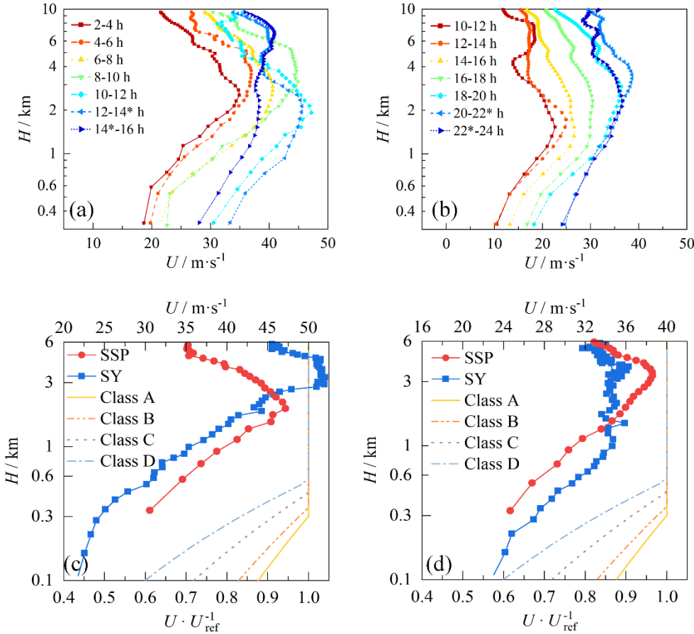
Figure 12: Vertical profiles of 2-h mean wind speed—(a): results at SSP for Mangkhut, (b) results at SSP for Saola , (c): profiles containing the maximum wind at SSP and SY during Mangkhut compared to stipulations in wind load code of China, (d): similar to (c) but for Saola . 14* and 22* in (a, b) indicate the landfall moments of Mangkhut (14:00) and Saola (22:00).
