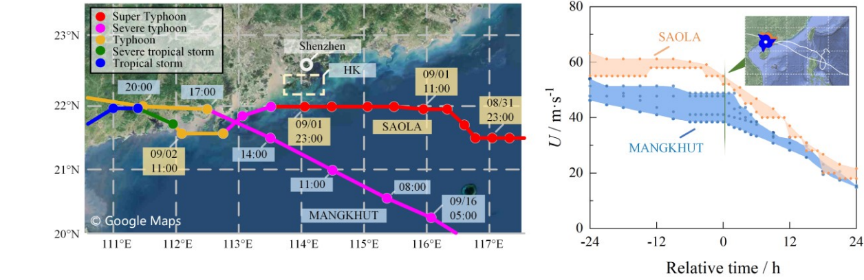
Figure 1: Evolution of the track and intensity of Mangkhut and Saola (Image: Google Maps). (a): center track from CMA, (b) TC intensity in form of envelopes based on the best-track data issued by CMA, HKO, TCC and JTWC. Relative time = 0 (from Google Maps) in (b) denotes the moment when the storms moved closest to HK, i.e., at 14:00 on 16 th Sep 2018 for Mangkhut , and at 22:00 on 1 st Sep 2023 for Saola (hereafter)
