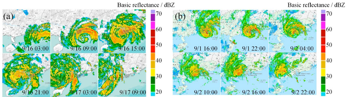
Figure 4: Echo-grams from ground-based weather radar for Mangkhut (a) and Saola (b). All grams correspond to a geographical area of 1000×1000 km (from 108° E/18° N to 119° E/27° N)
