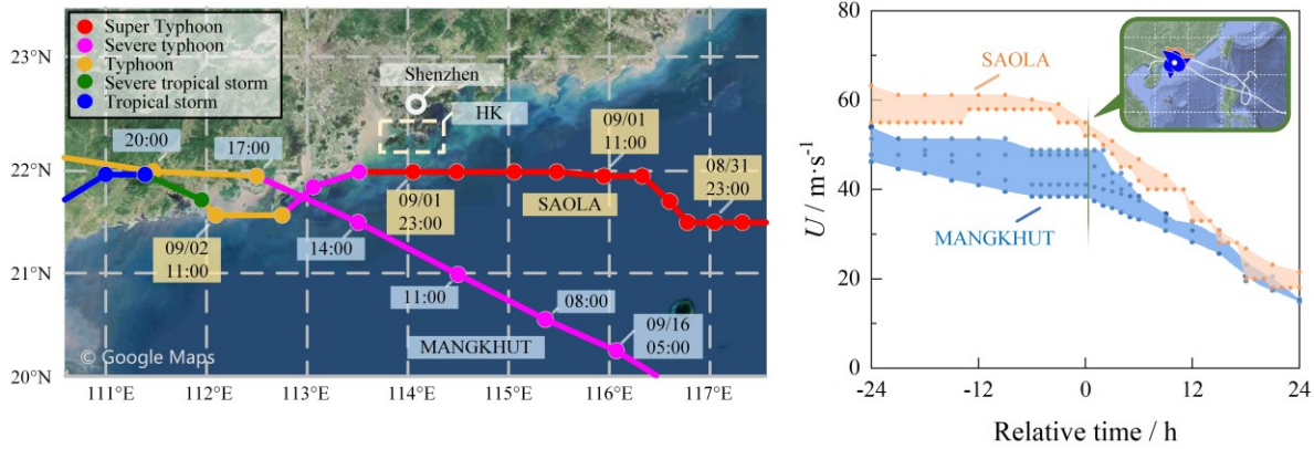
Figure 1: Evolution of the track and intensity of Mangkhut and Saola . (a): center track from CMA, (b) TC intensity in form of envelopes based on the best-track data issued by CMA, HKO, TCC and JTWC. Relative time = 0 (from Google Maps) in (b) denotes the moment when the storms moved closest to HK, i.e., at 14:00 on 16 th Sep 2018 for Mangkhut , and at 22:00 on 1 st Sep 2023 for Saola (hereafter)
