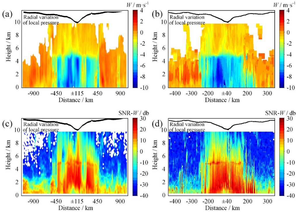
Figure 11: Vertical profiles of nominal vertical speed ( W ) and associated signal-to-noise ratio ( SNR ) at SSP—(a): W for Mangkhut , (b): W for Saola , (c): SNR for Mangkhut , (d): SNR for Saola .
