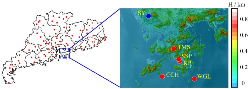
Figure 2: Layout of metrological sites in HK and Guangdong Province: the red dots in the left picture correspond to the 86 natural meteorological stations
