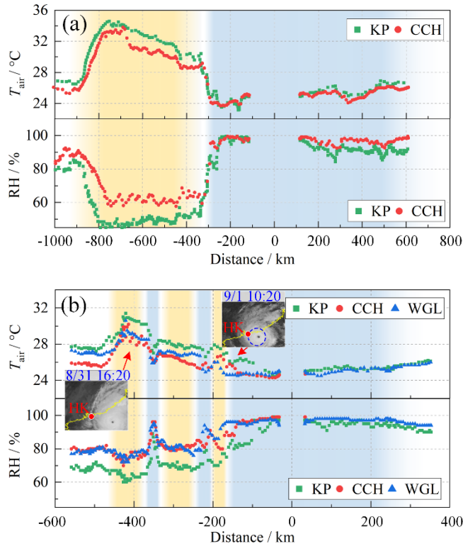
Figure 5: Radial distribution of dry-bulb temperature ( T_{air} ) and relative humidity (RH) at 3 sites in HK during the landfall of Mangkhut (a) and Saola (b)
