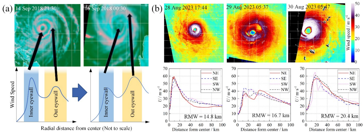
Figure 8: ER cycle for Mangkhut (a) and Saola (from https://www.weather.gov.hk/informtc/Mangkhut18/windstructure.htm ) (b). Cloud image represents radial wind profiles obtained through the conversion of cross-polarized normalized radar cross section backscatter (from https://www.star.nesdis.noaa.gov/socd/mech/sar )
