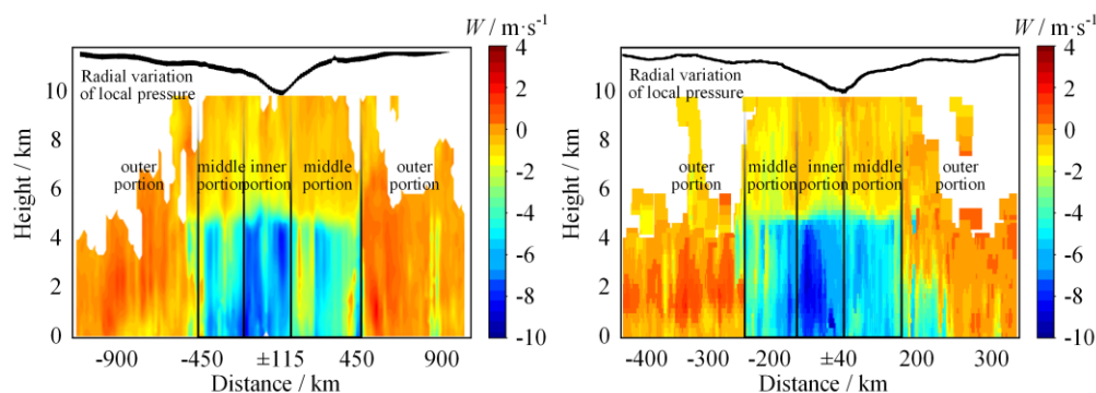
Fig.3. Vertical profiles of nominal vertical speed ( W ) and associated signal-to-noise ratio ( SNR ) at SSP—(a): W for Mangkhut , (b): W for Saola
