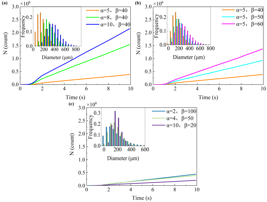
Figure 11. Number of snow particles as a function of time. (a) variation of shape parameter \alpha , scale parameter \beta = 40 , const. (b) variation of scale parameter \beta , shape parameter \alpha = 5 , const. (c) \alpha \times \beta = \text{Average diameter } \bar{d} = 200 \mu\text{m} .
