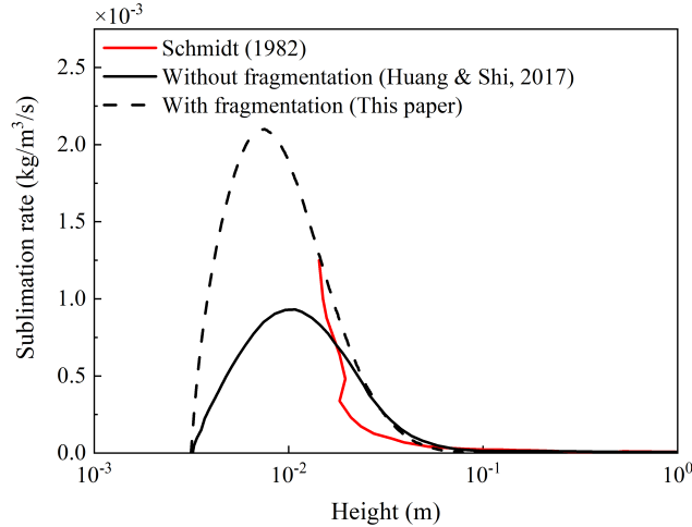
Figure 3. Comparison of total sublimation rate profile for this paper and field observations, (Schmidt, 1982), for ( u_* = 1.1 m/s, z_0 = 3.2 \times 10^{-4} m, T = 265.65 K).
