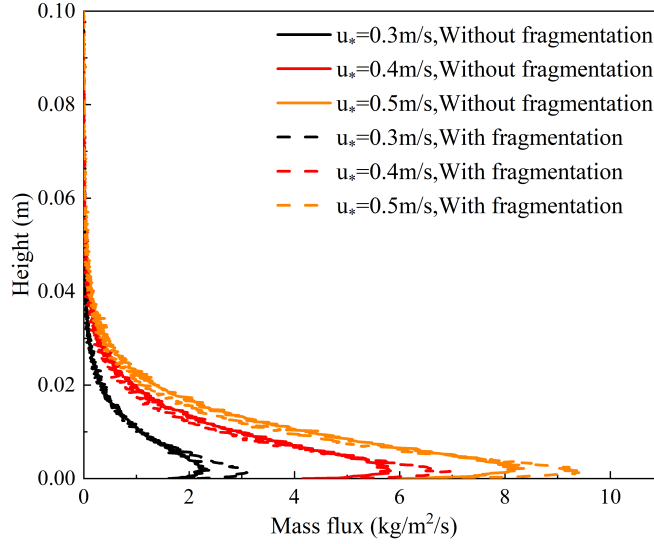
Figure 9. Simulated horizontal mass flux profile of snow particles with/without considering fragmentation, under wind conditions of u_* = 0.3, 0.4 , and 0.5 m/s.
