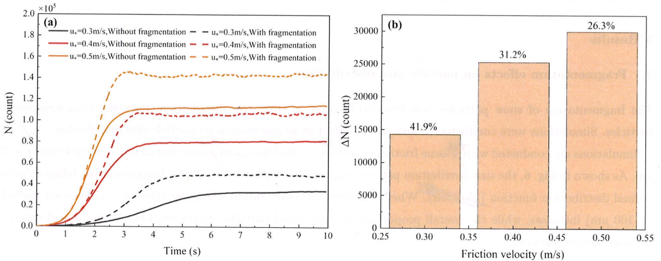
Figure 7. (a) Saltating particle number variation with time under wind conditions of u_* = 0.3, 0.4 and 0.5 m/s. (b) Increment number and ratios of saltation snow particles in the air. All results from simulations of the present study.
