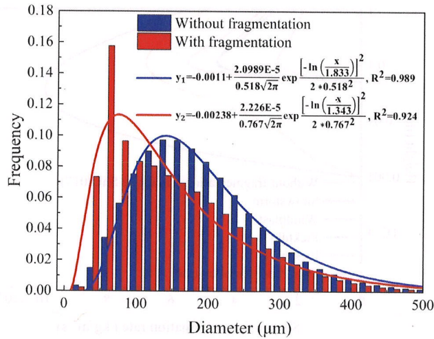
Figure 6 Size distribution with and without considering the particle fragmentation. in the simulation
