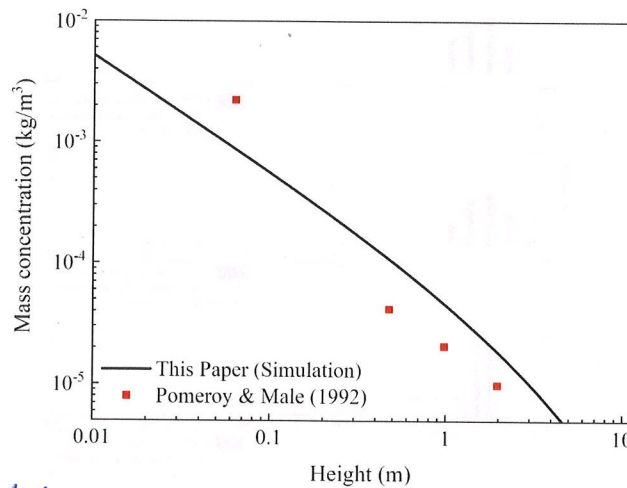
simulated Figure 4. Comparison of mass concentration for this paper and field observations, (Pomeroy and Male, 1992) for ( u_* = 0.31 m/s, T = 265 K) .
