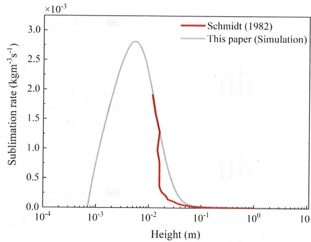
Figure 3. Comparison of total sublimation rate for this paper and field observations, (Schmidt, 1982) for ( u_* = 0.63 m/s, z_0 = 7 \times 10^{-4} m, T = 267.45 K) .
