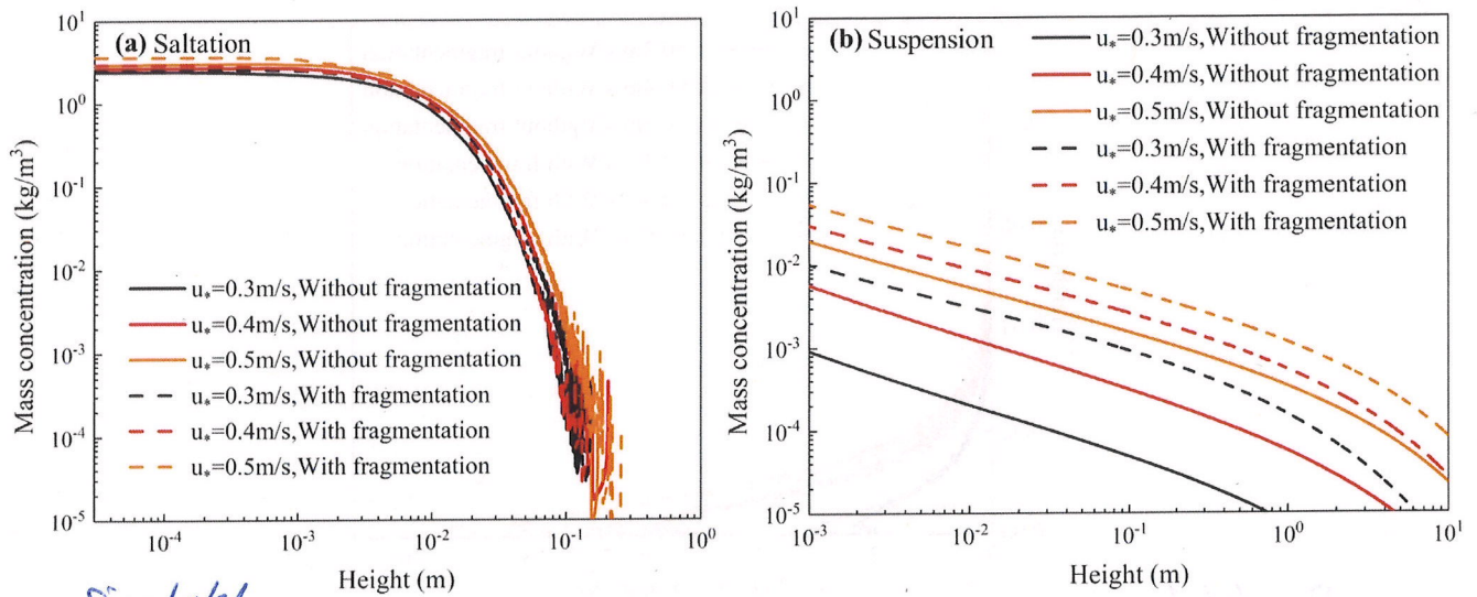
Figure 8. Simulated Mass concentration of (a) saltating on and (b) suspension particles with/without considering fragmentation, under wind conditions of u_* = 0.3, 0.4 and 0.5 m/s.
