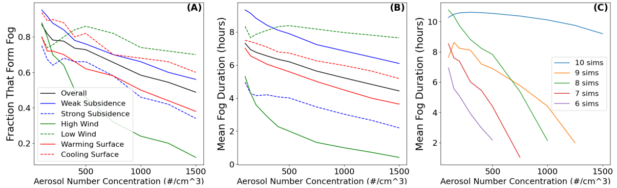
Figure 3. Relationships between N_a and (A) the fraction of simulations that form fog at some time, and (B) the mean fog duration including non-foggy simulations with respect to N_a averaged over different simulation subsets based on input parameter values. Panel (C) shows the aerosol "base-case" mean duration of foggy simulations with respect to N_a for combinations of w_{sub} , U_g , and dT_{surf} in which the specified number of simulations (continuously starting from the lowest N_a ) all formed fog.
