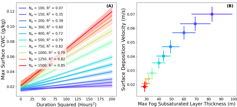
Figure 5. The left panel shows relationships between the square of fog duration (an assumed proxy for fog area) and max surface CWC CWC during the fog event. Trend-lines are shown for each input value of aerosol content with 95% confidence interval shaded. The right panel shows the maximum thickness of the subsaturated layer during fog and the cloud droplet deposition velocity in the lowest model level averaged for each value of N_a . The standard deviations of are shown for both axes. R^2 values are shown for each N_a listed in panel A . Note low R^2 values at low N_a , which result from the weak overall relationship between squared fog duration and maximum surface fog density. Relative to the overall simulation variability of fog density at the surface, the trend lines do a good job of describing the relationship between squared duration and density at low N_a .
