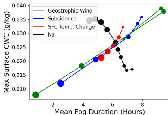
Figure 4. Plots of mean Mean fog duration over all non-outlier simulations (both foggy and non-foggy) and as a function of max surface CWC averaged over each input parameter value. Point size represents the relative value of each input parameter, with the largest points representing U_g = 15 m/s, w_{sub} = 3.5 mm/s, SST rate of change = 2 K/day, and N_a = 1500 cm -3 .
