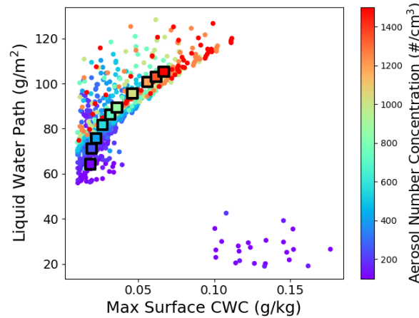
Figure 2. Scatter plot of maximum surface CLWC CWC and liquid water path at the time of maximum surface CLWC CWC for all simulations that produced fog. Points are colored by N_a . Note the well-separated group of points at the lower-right of the plot. In addition to low N_a , simulations in this outlier group had a cooling surface and typically low U_g . Square points with black borders represent mean values for each aerosol concentration with the outlier points excluded.
