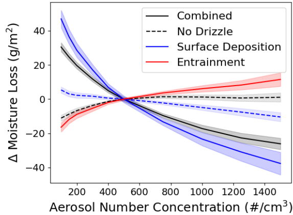
Figure 6. Plot of impacts of N_a on boundary layer moisture loss due to entrainment and surface deposition relative to N_a = 500 \text{ /cm}^3 . Dashed blue line represents surface deposition of cloud droplets only and dashed black line shows combined moisture loss due to entrainment and cloud droplet deposition.
