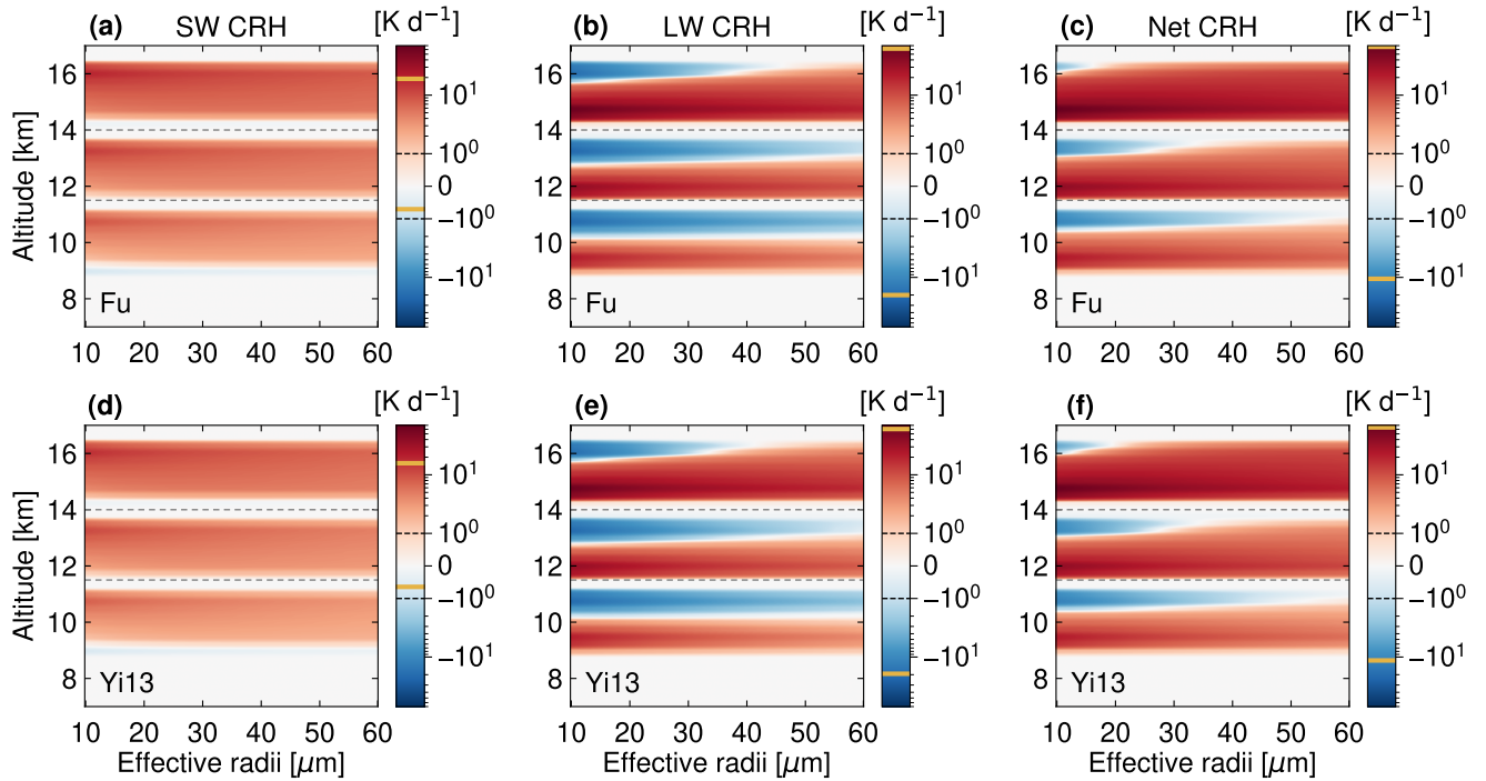
Figure S14. Heating rate matrix visualizations including CRH interscheme difference profiles for ice crystal effective radii ranging from 10 to 60 \mu\text{m} (Test 4). Three separate profiles are calculated for low, middle, and high cloud temperatures of 201 K, 218 K, and 236 K as in test 3. Columns, axes, and colorbar are as in Fig. S4, with a general range from -70 to 70 \text{K day}^{-1} . The limit between the linear and logarithmic scale is 1 \text{K day}^{-1} .
