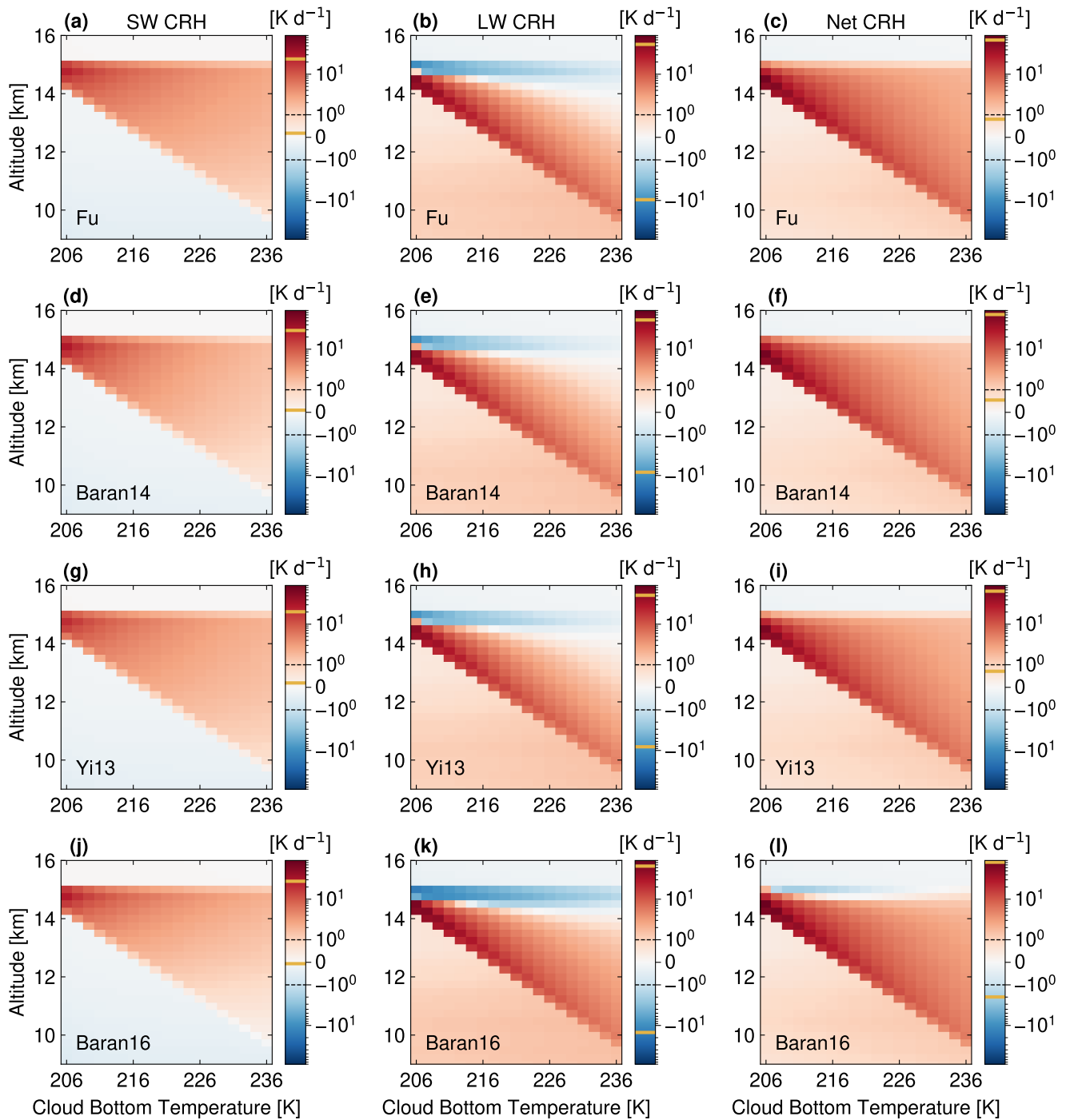
Figure S8. Matrix visualizations including 19 CRH profiles each for cloud depths from 0.5 to 5 km, with fixed cloud top temperature of 203 K (Test 2a). Panels, axes, and colorbar are as in Fig. S4, with a general range from -90 to 90 K day^{-1} .
