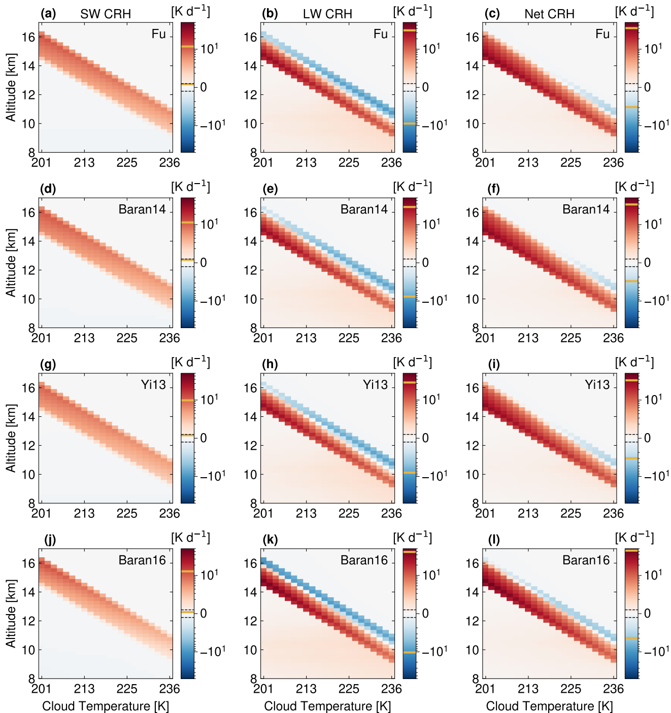
Figure S4. Matrix visualizations including 22 CRH profiles each for middle cloud temperatures from 201 K to 236 K (Test 1). Each column panel shows the corresponding radiative components (SW, LW, and Net), and each row corresponds to the schemes under test. The corresponding height position of the layer cloud is depicted in the y-axis while the CRH magnitude is represented in the color bar, with a general range from -60 to 60 K day^{-1} . Yellow lines in the color bar show the corresponding CRH range for each panel. Black dash lines in the color bar mark the limit between the linear and logarithmic scale in the color bar ( 1 K day^{-1} ).
