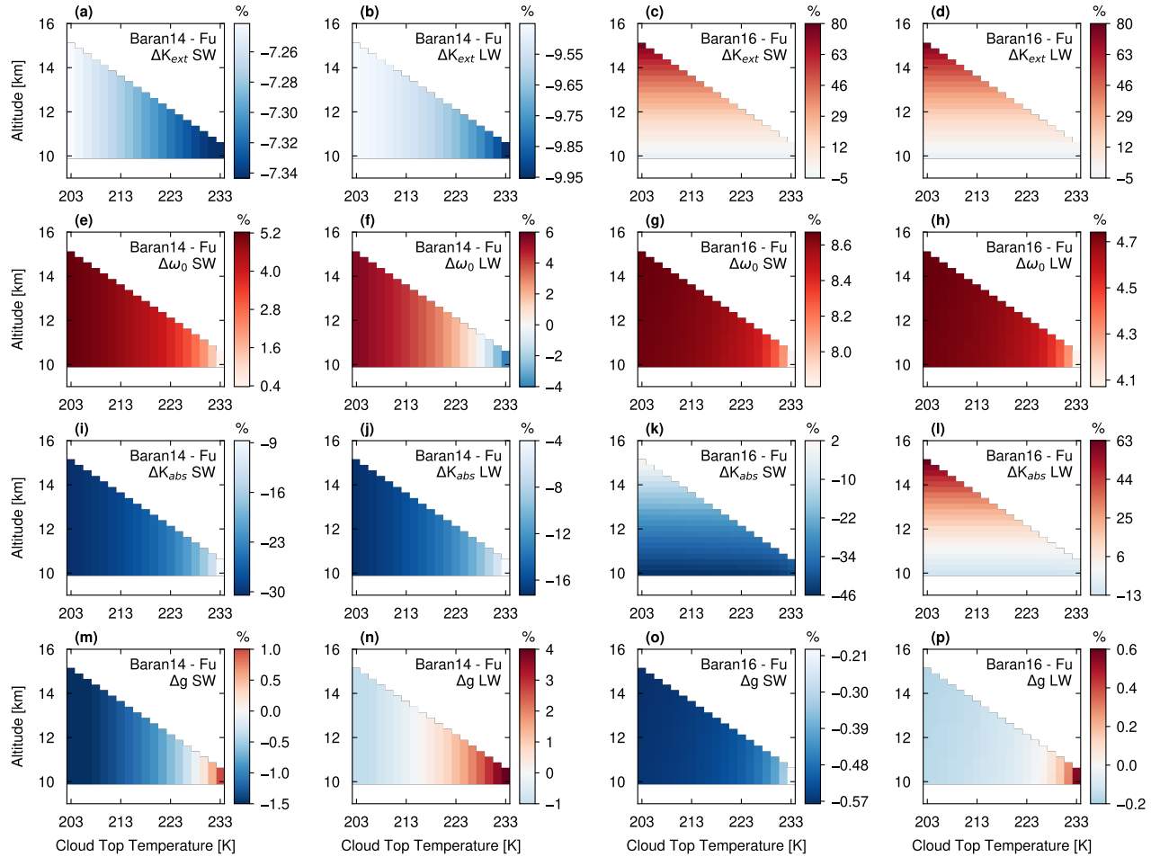
Figure S11. Matrix visualizations including interscheme relative difference profiles for the K_{ext} , \omega_0 , K_{abs} and g , with the same depth range as in Fig. S9 and with fixed cloud bottom temperature of 237 K (Test 2b). Panels, axes, and colorbar are as in Fig. S5.
