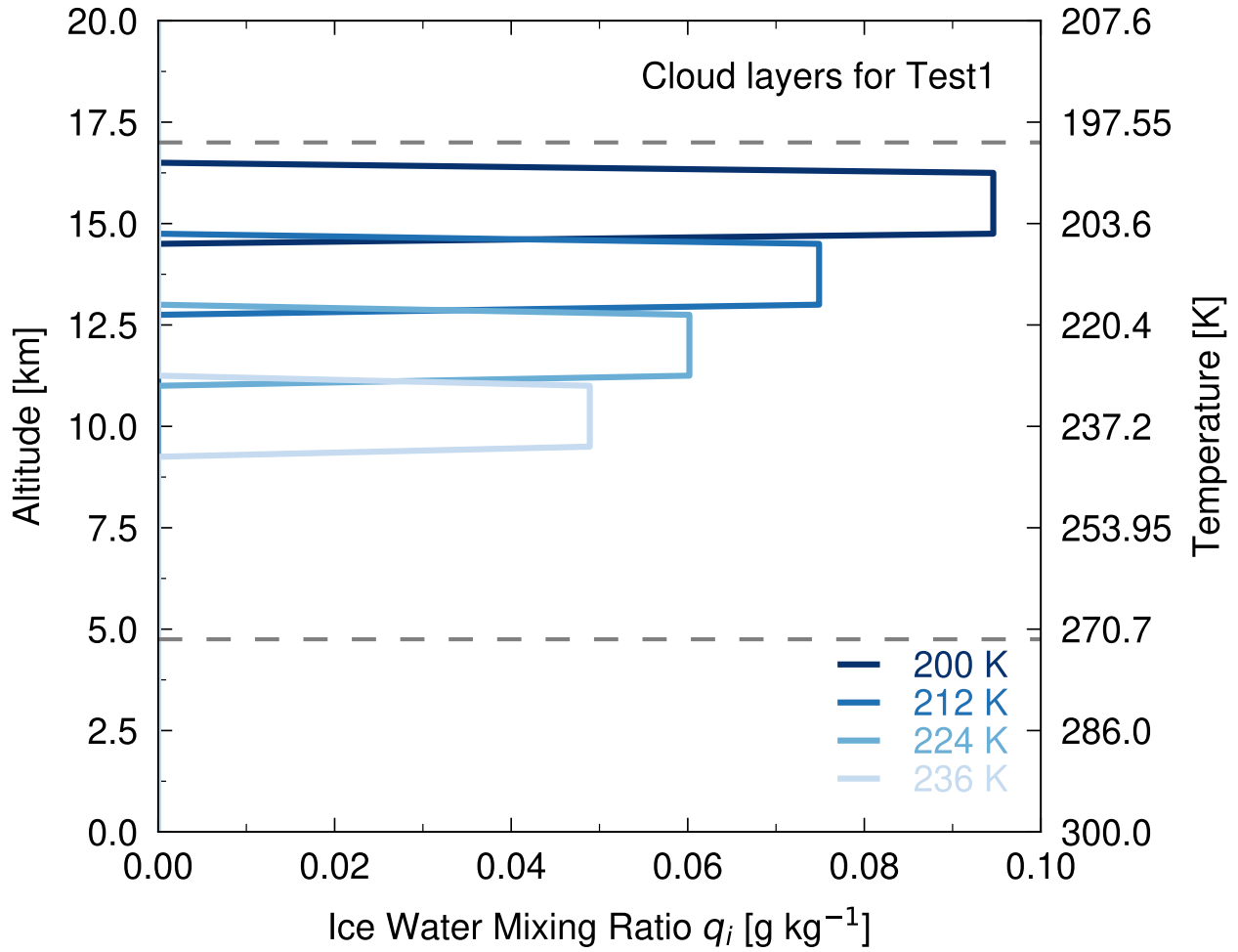
Figure S1. Ice clouds profile for different temperature perturbation levels (Test 1). A geometrical depth of 1.5 km and an IWP of 30 \text{ g m}^{-2} is used to compute q_i
