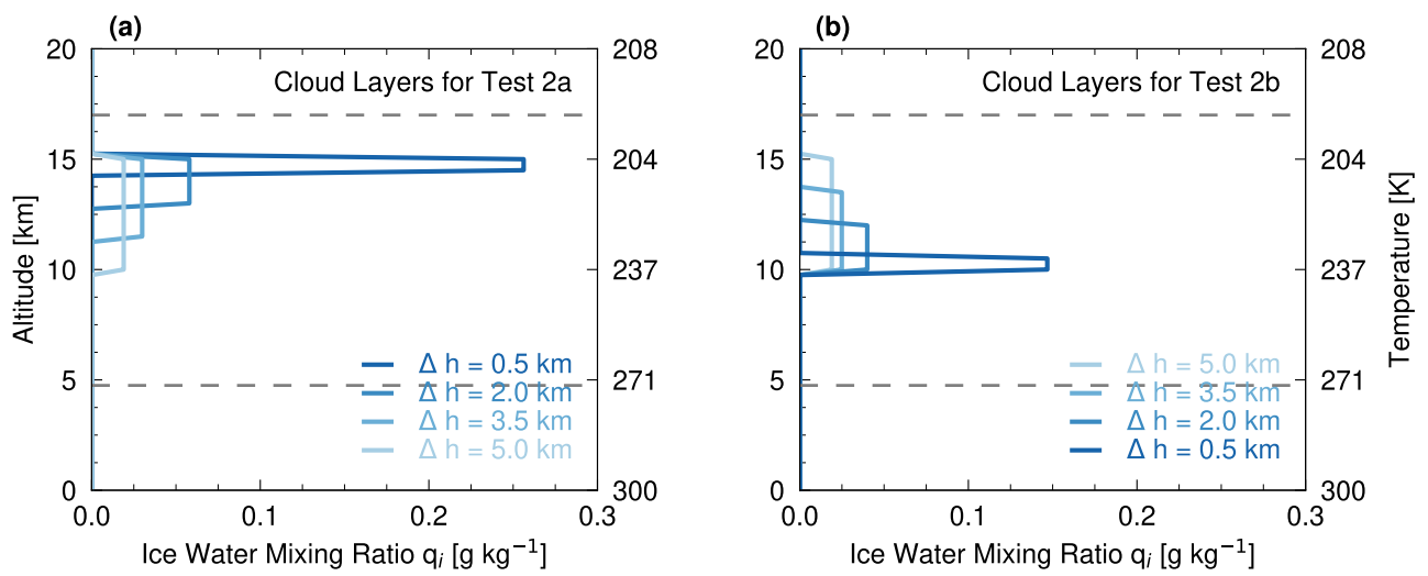
Figure S2. Ice clouds profile for different geometrical depths. Test 2a (a) and test 2b (b). An IWP of 30 \text{ g m}^{-2} is used to compute q_i .
