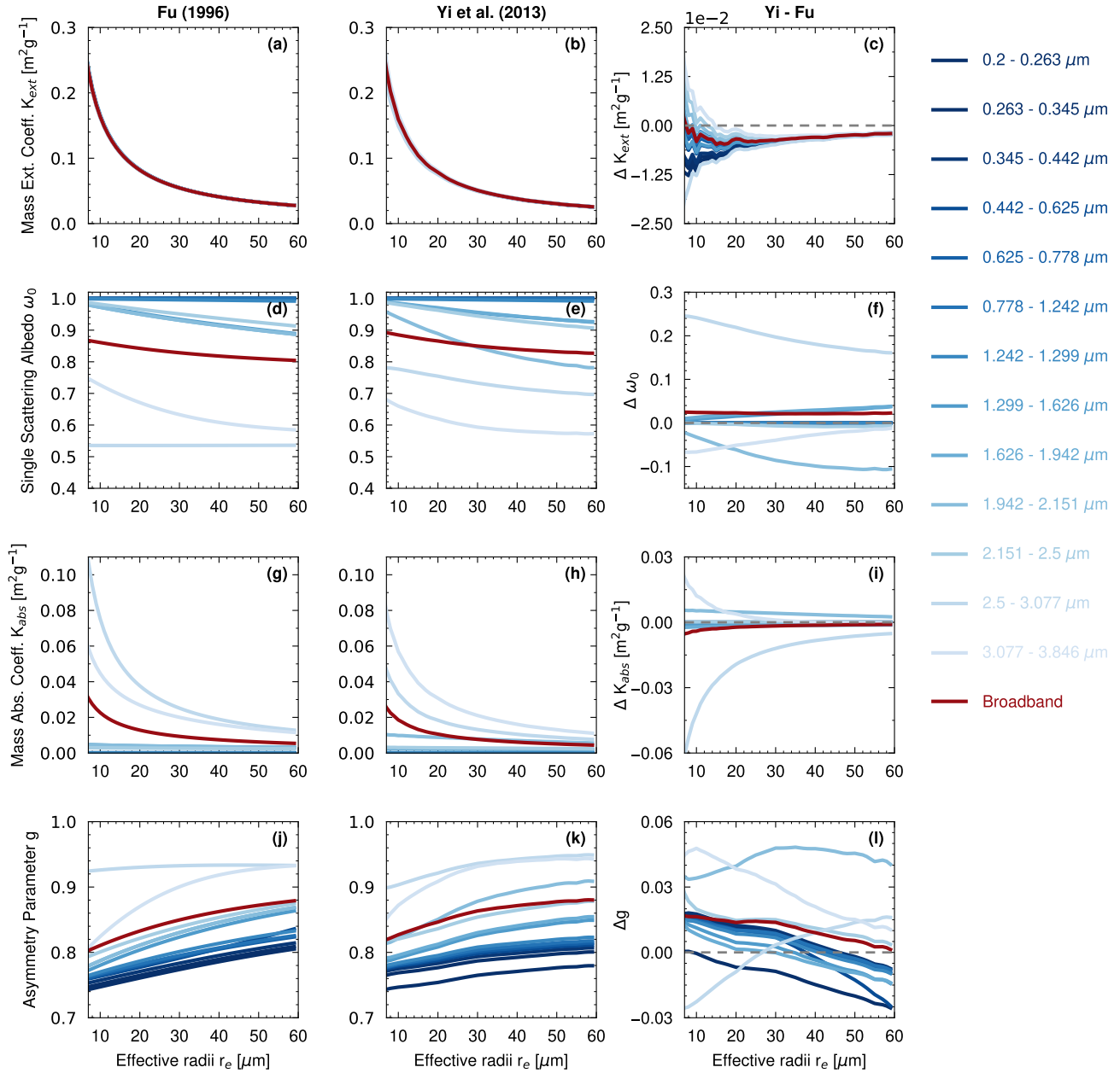
Figure S6. Shortwave (SW) optical parameterizations as a function of ice crystal effective radii. Each row shows the optical properties from top to bottom: mass extinction coefficient K_{ext} , single scattering albedo \omega_0 , mass absorption coefficient K_{abs} and asymmetry parameter g . The left column shows Fu scheme, the middle column Yi13 scheme, and the interscheme difference is shown in the right column. 13 RRTMG SW bands, and broadband calculation is included in each panel.
