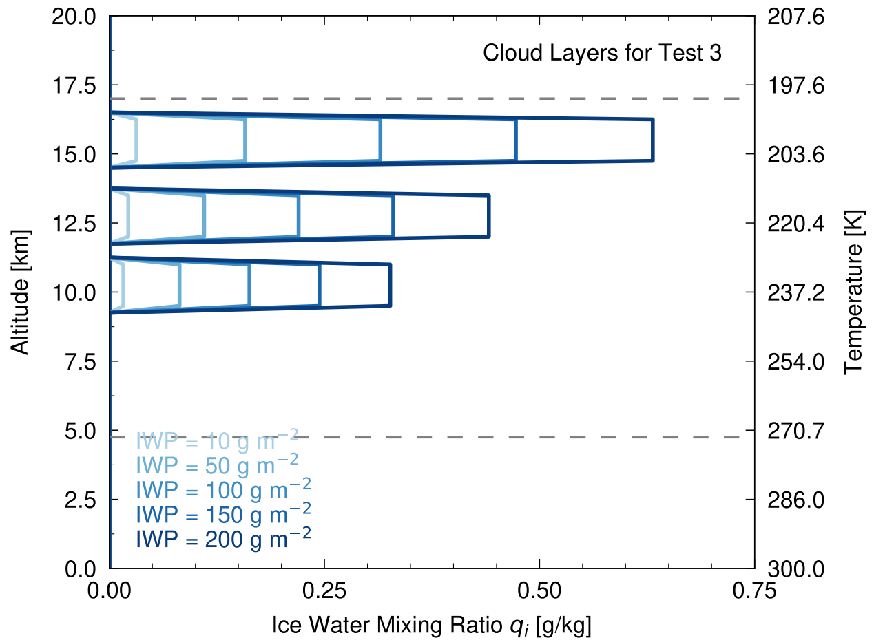
Figure S3. Ice clouds for different IWP and three temperature perturbation levels (Test 3). A geometrical depth of 1.5 km is used to compute q_i
