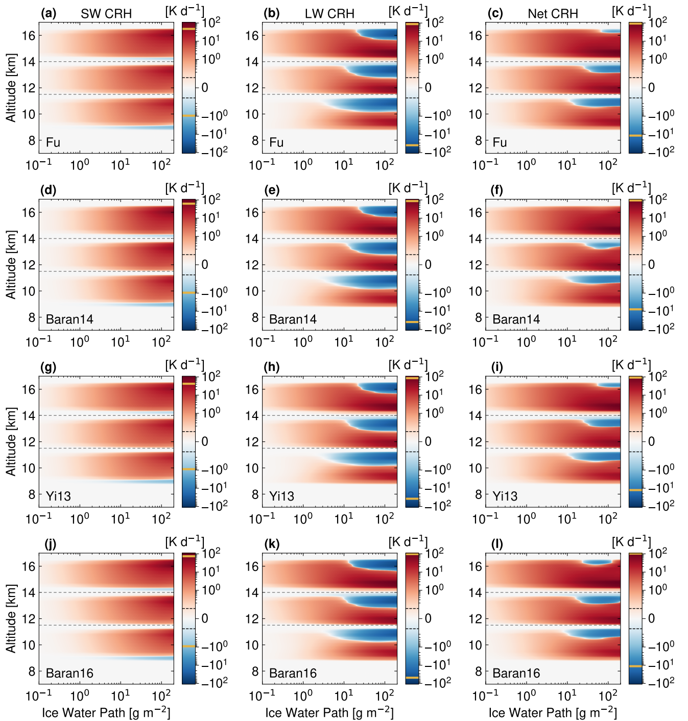
Figure S12. Matrix visualizations including CRH profiles for IWPs from 0.1 to 200 \text{ g m}^{-2} in Test 3. Three separate differences are shown for cloud temperatures of 201 K, 218 K, and 236 K, corresponding to high, middle, and low altitudes. Panels, axes, and colorbar are as in Fig. S4, with a general range from -100 to 100 \text{ K day}^{-1} . The limit between the linear and logarithmic scale is 0.01 \text{ K day}^{-1} .
