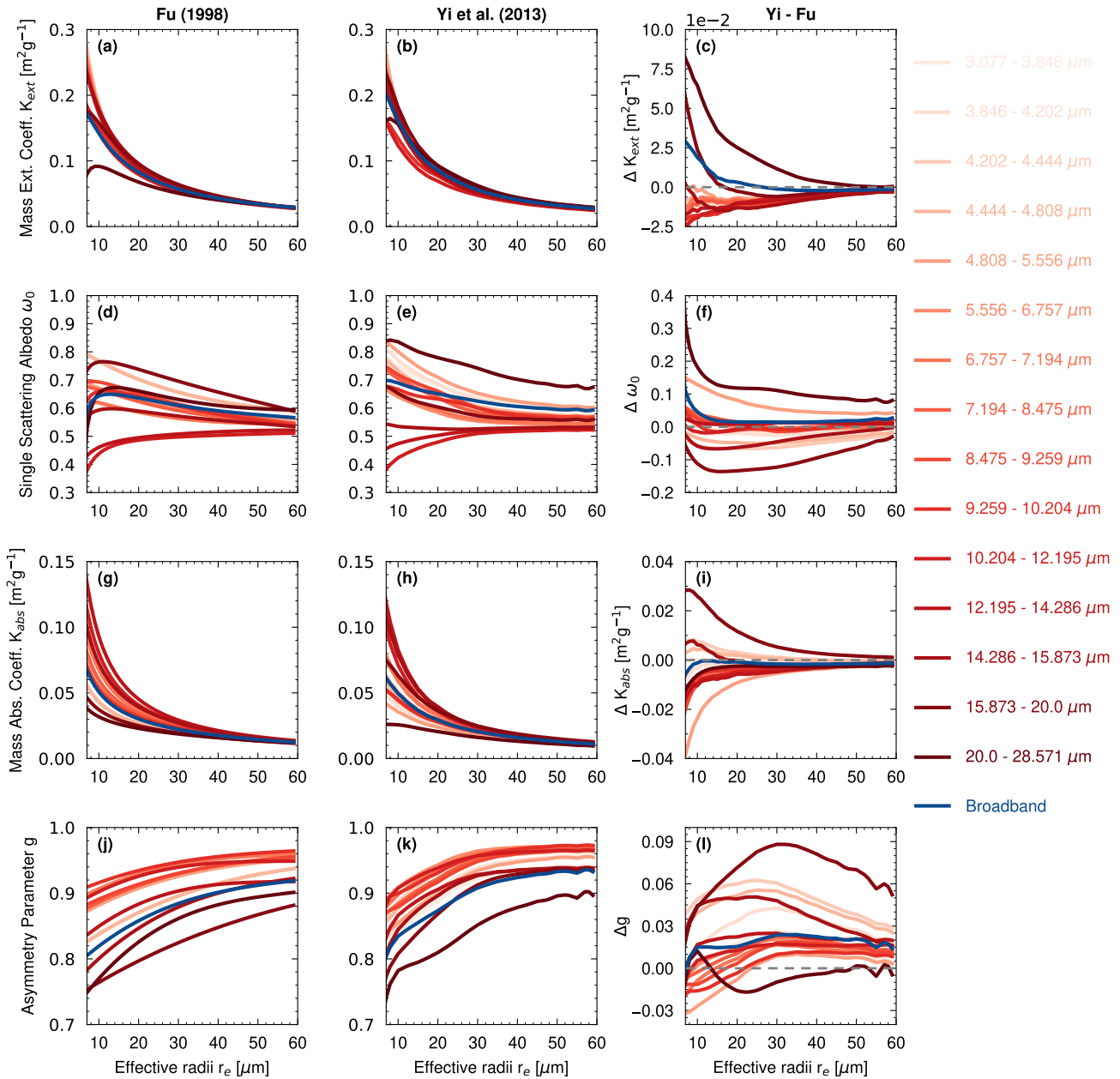
Figure S7. Longwave (LW) optical parameterizations as a function of ice crystal effective radii. Panels distribution are as in Fig. S6. 15 RRTMG LW bands, and broadband calculation is included in each panel.
