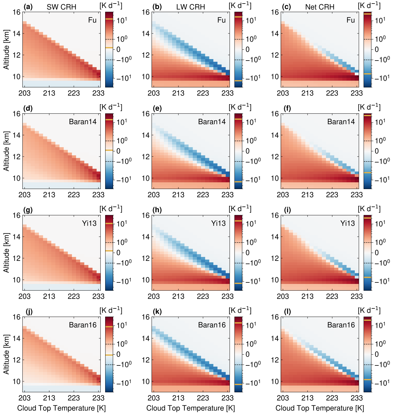
Figure S10. Matrix visualizations with the same depth range as in Fig. S8 and with fixed cloud bottom temperature of 237 K (Test 2b). Panels, axes, and colorbar are as in Fig. S4, with a general range from -30 to 30 \text{ K day}^{-1} .
