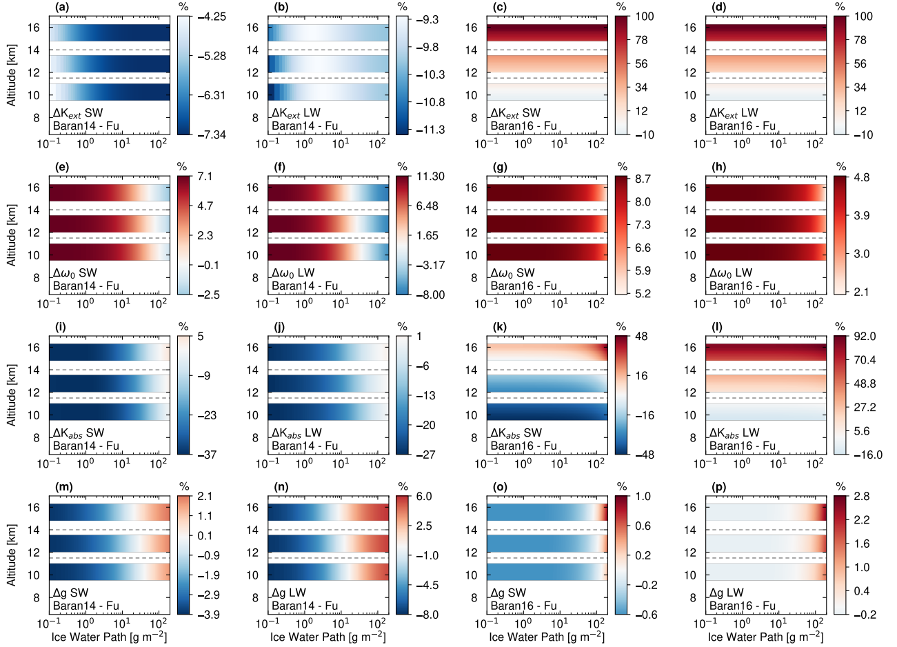
Figure S13. Matrix visualizations including interscheme relative difference profiles for the K_{ext} , \omega_0 , K_{abs} and g . The IWP range and the three independent cloud layers are as in Fig. S12 (Test 3). Panels, axes, and colorbar are as in Fig. S5.
