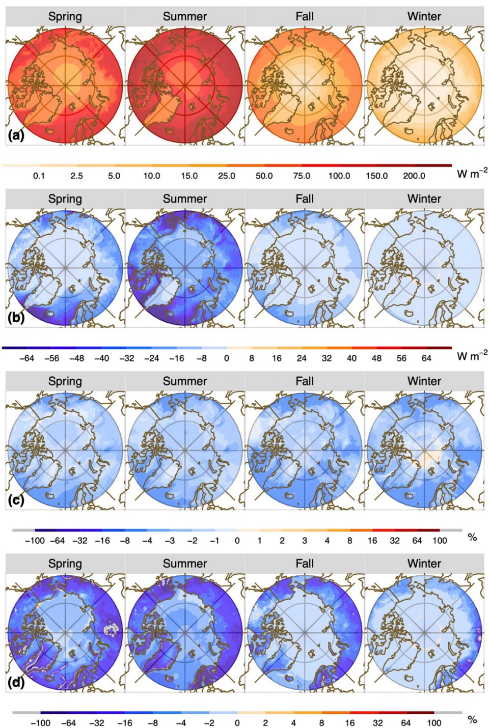
525 Figure 5, similar to Figure 2, but for results according to the net shortwave radiation (SWN).
