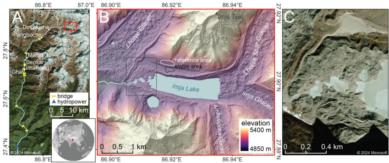
120 Figure 1: Context maps for the Imja Lake moraine dam. A) Microsoft satellite basemap showing the area downstream of Imja Lake, including settlements and infrastructure along the Dhudh Kohsi river. B) Color-shaded relief map from median composite of EarthDEM strips acquired during the 2014-2019 period (Porter et al., 2022). C) © Microsoft satellite basemap detail of the Imja Lake moraine dam. Microsoft product screen shots reprinted with permission from Microsoft Corporation.
