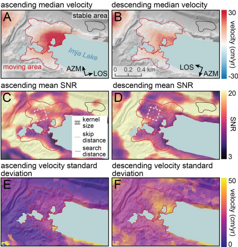
405 Figure 6: Sentinel-1 SAR image feature tracking results for the full 2017-2024 time series, including all 192 pairs on ascending (left) and 210 pairs on descending (right) orbits. A, B) Per-pixel median feature tracking velocity in the slant-range direction (along the line-of-sight). Results are masked in areas with high InSAR coherence (Figure 4), where feature tracking products are not used during inversion. C, D) Per-pixel median signal-to-noise (SNR) ratio. E, F) Per-pixel standard deviation of the feature tracking velocity in range direction. Higher standard deviation values are observed for locations with 1) greater temporal variability, 2) fewer reliable displacement measurements, and/or 3) larger measurement error. 410
