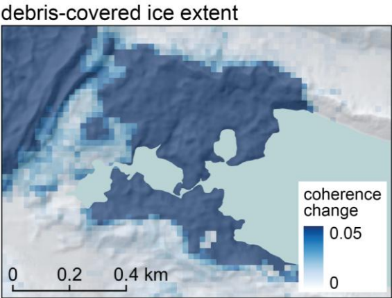
Figure 5: Seasonal change in median coherence offers a proxy to map the spatial distribution of buried ice.
