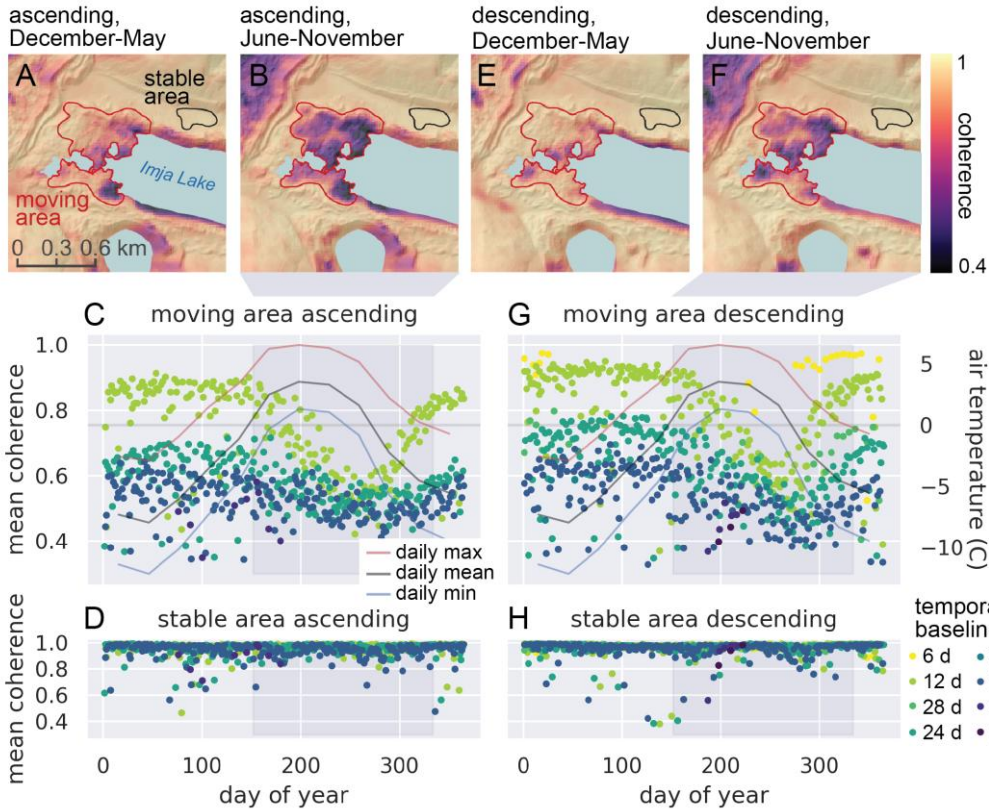
370 Figure 4: Imja Lake moraine dam InSAR coherence and air temperature. Mean coherence maps for all 439 12-day pairs of ascending Sentinel-1 SAR images during the colder months (A) and warmer months (B). C) Mean coherence of the moraine dam moving area in all ascending interferograms. Lines show mean daily maximum, mean, and minimum air temperature for each month from the nearby Pyramid Weather Station (UCAR/NCAR-Earth Observing Laboratory et al., 2011). D) Mean coherence of the stable area for all ascending interferograms. Panels E-H show corresponding plots for descending pairs.
