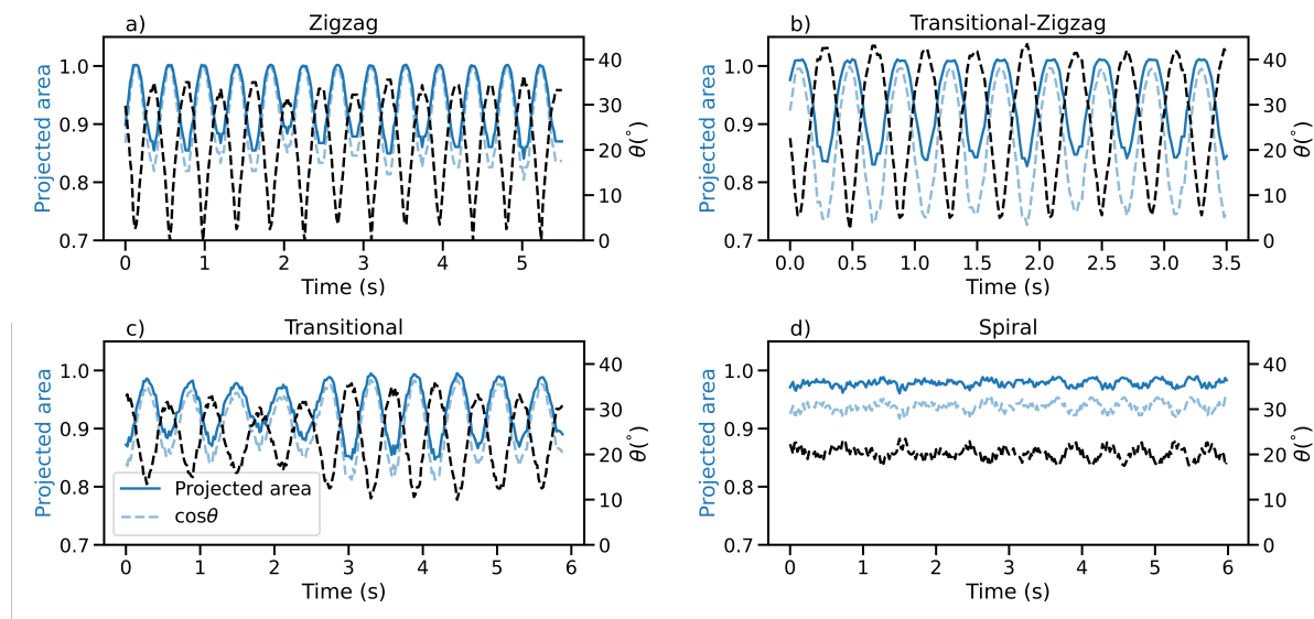
Figure 8. Time-series of modelled projected areas as seen from below for each case study, normalised by the maximum observed projected area (blue). \theta (dashed, black) and \cos\theta (dashed, light blue) provided for reference.
