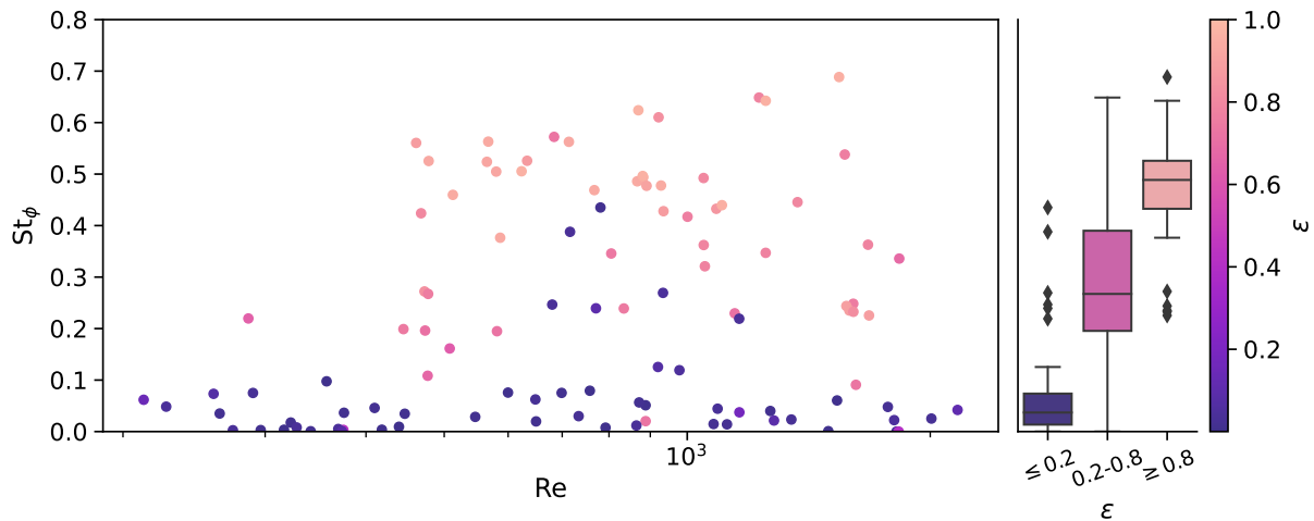
Figure 15. Scatter plot of azimuth Strouhal numbers ( St_\phi ) for each unstable experiment versus Reynolds number, coloured by \epsilon . Experiments where \theta_{amp} < 2.5^\circ marked with crosses. Box plots of observed Strouhal numbers for particles with \theta_{amp} > 2.5^\circ alongside.
