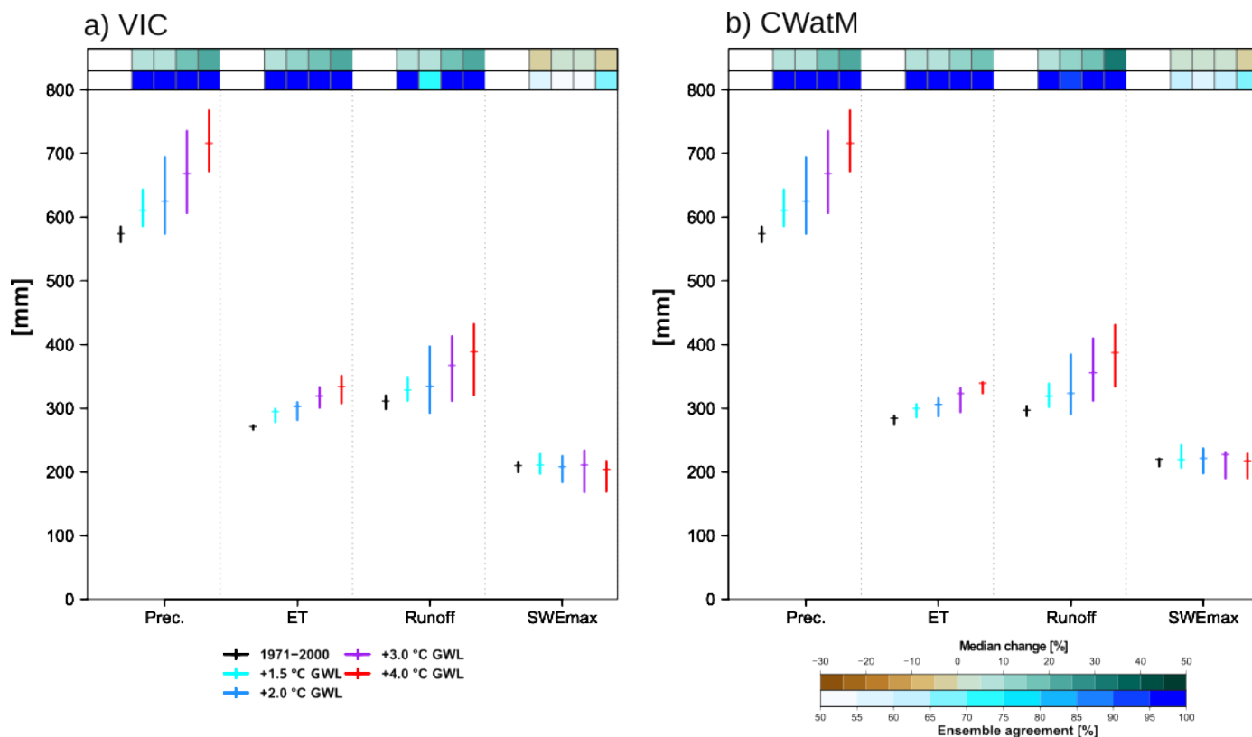
Figure 4. Historical (1971-2000) and projected annual water balance variables ([mm]) at 1.5 to 4.0 °C GWLs obtained from the GCM ensemble. The results show basin-averaged values for the entire Liard River basin, consisting of precipitation used as forcings, and a) VIC and b) CWatM simulated evapotranspiration (ET), runoff and maximum snow water equivalent (SWE max ). Top panels show the median change (%) at the four GWLs relative to 1971-2000, along with the model agreement of ensemble members (%) of the GCM ensemble with the direction of median change.
