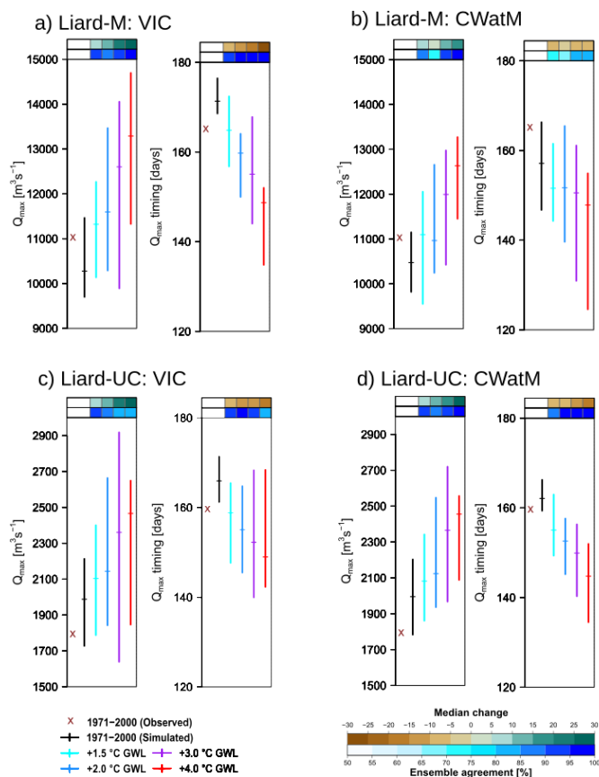
Figure 7. Historical (1971-2000) and projected annual maximum flows and their timing at 1.5 to 4.0 °C GWLs obtained from the GCM ensemble. Top panels show median change [%] at four GWLs relative to 1971-2000, along with the model agreement of ensemble members [%] of the GCM ensemble with the direction of median change.
