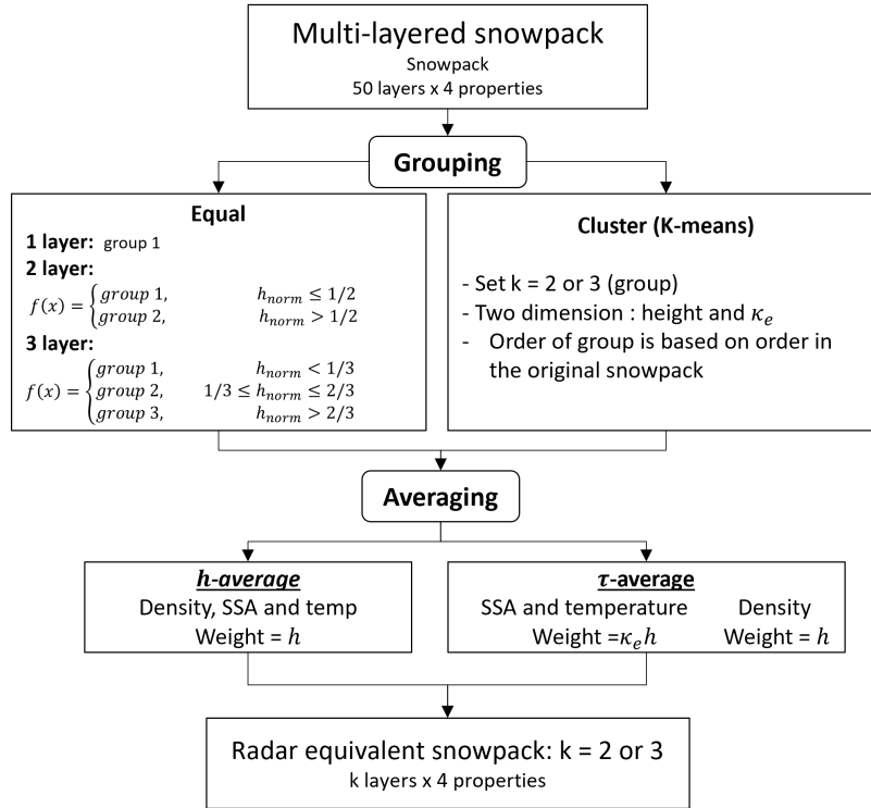
Figure 1. Schematic of the methodology. Necessary steps in the snowpack simplification are shown vertically and the different options (grouping and averaging) are shown horizontally where h_{\text{norm}} is the normalized height and h is the layer thickness. The 4 snow properties considered are: thickness, density, temperature and SSA.
