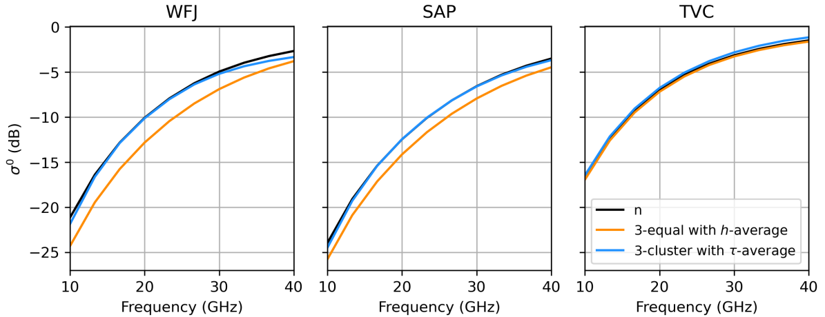
Figure 5. Backscatter simulations of 3-equal with h -average and 3-cluster with \tau -average methods as a function of frequency
