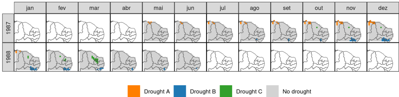
435 Figure 3: Example of simultaneously occurring drought events identified by the space-time clustering and tracking algorithm. Colored patches denote drought clusters belonging to different event IDs at each time step. White indicates no grid cells meet the drought criterion at that time step (non-drought), and grey denotes the non-drought grid cells when exists at least one drought event at that time step.
