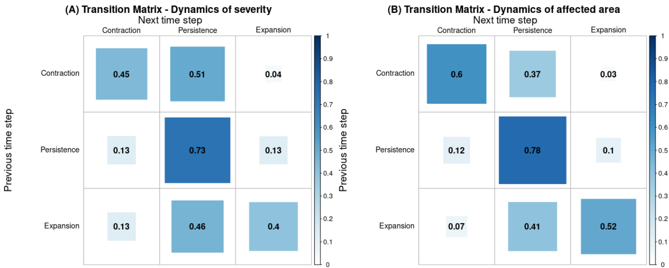
620 Figure 8: Transition matrix indicating the probability of a drought event remaining in the same phase or transitioning to another. Higher values along the diagonal suggest a strong persistence of each phase, whereas higher off-diagonal values indicate frequent transitions between phases.
