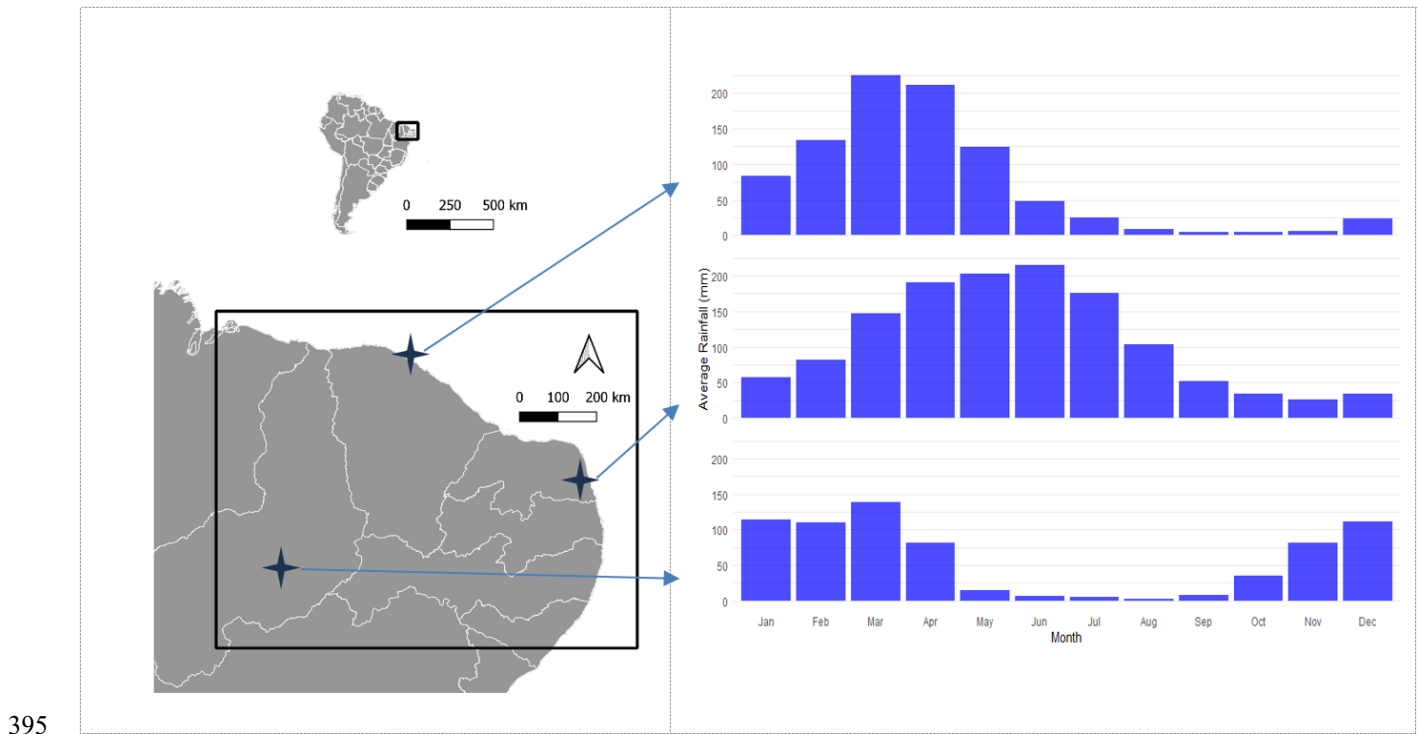
400 Figure 2: Location map showing the northern portion of Northeast Brazil (NEB). The rainfall charts are representative of the northern zone influenced by ITCZ, the eastern zone influenced by Southeast Trade Winds, and the southern zone influenced by Cold Fronts. Rainfall data CRU TS v4.05 from 1950 to 2018.
