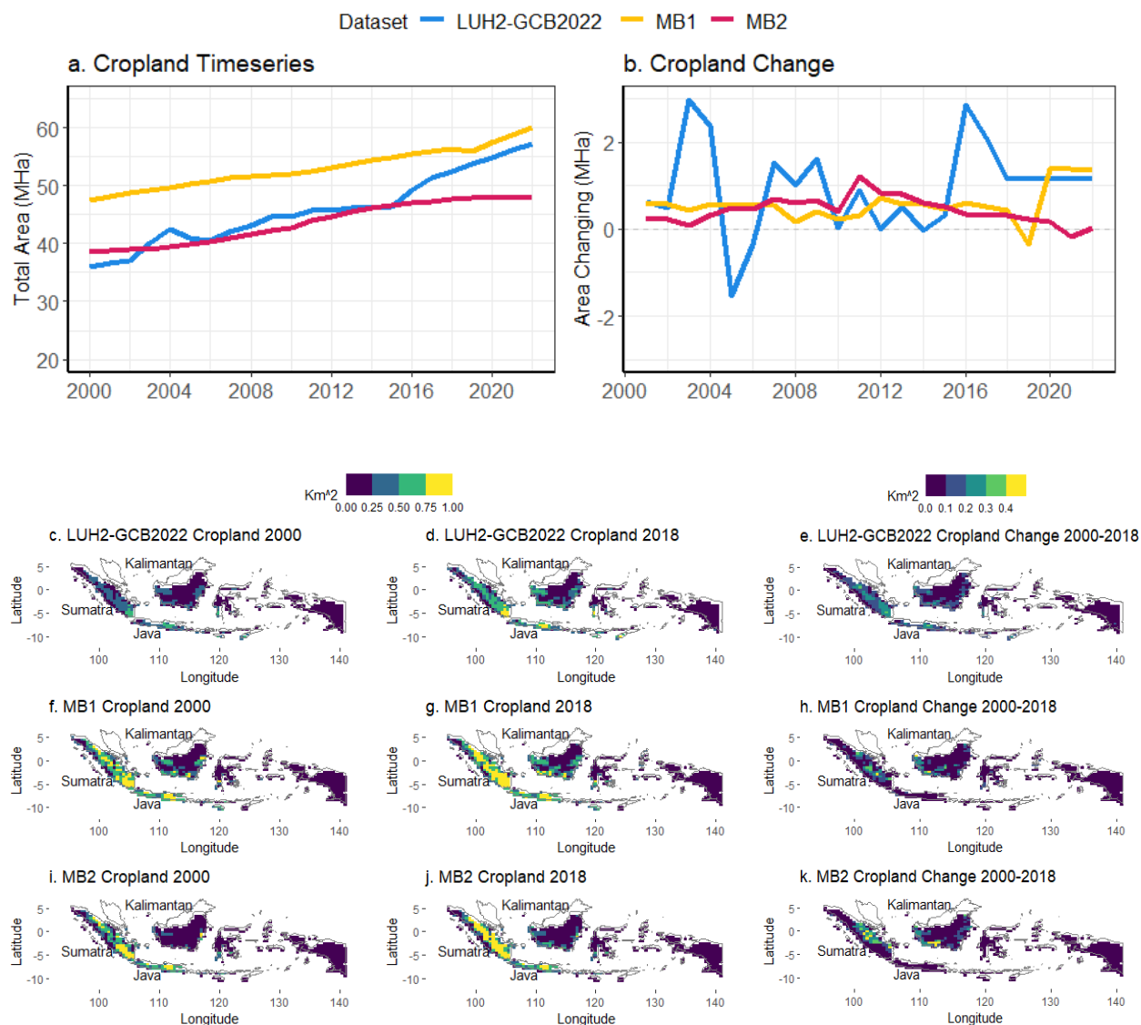
Figure 2: The comparison of data drivers timeseries of (a) cropland areas (MHa); (b) annual cropland area change (MHa); spatial distribution of cropland fraction in (c)LUH2-GCB2022 in 2000; (d) LUH2-GCB2022 in 2018; (e) LUH2-GCB2022 change between 2000 and 2018; (f) MB1 in 2000; (g) MB1 in 2018; (h) MB1 change between 2000 and 2018; (i) MB2 in 2000; (j) MB2 in 2018; (k) MB2 change between 2000 and 2018.
