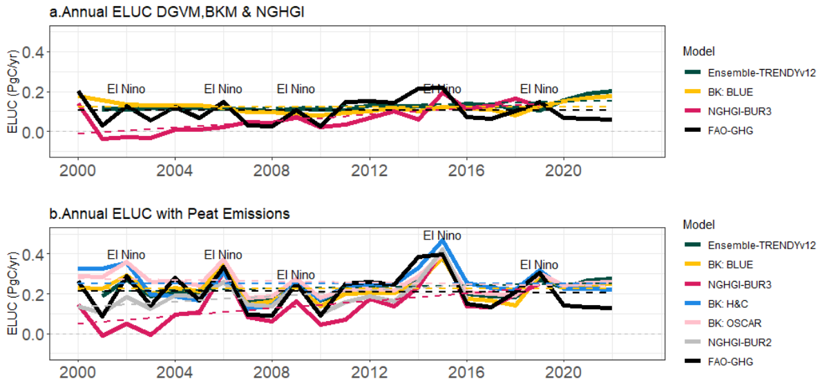
Figure 4: ELUC comparison of different models over the period 2000-2022 (a) Annual ELUC from DGVMs, BKM's and NGHGI; (b) Annual ELUC from BLUE and BUR3 models with and without peat emissions + Ensemble TRENDY v12
